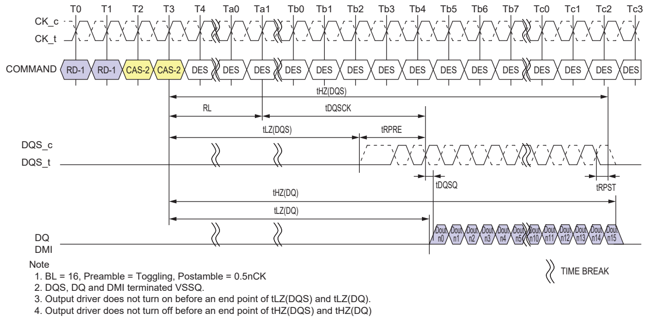
Figure 4.7 — Read Timing
