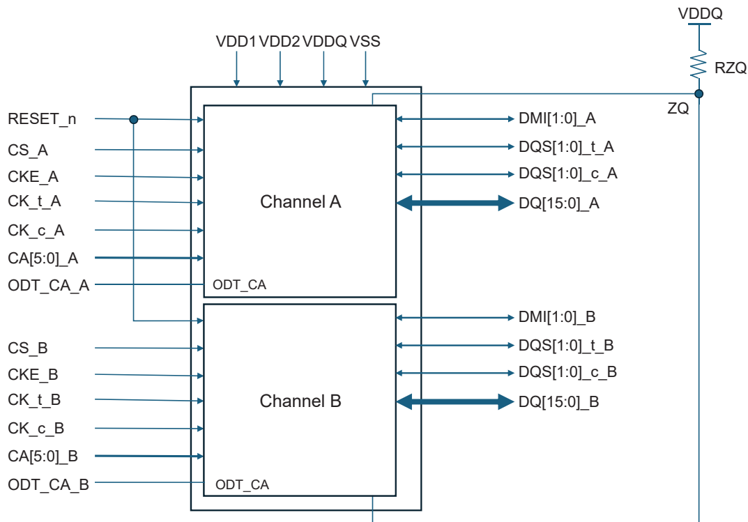
Figure 3.1 – Dual-channel (x32), Single-rank Package Diagram
