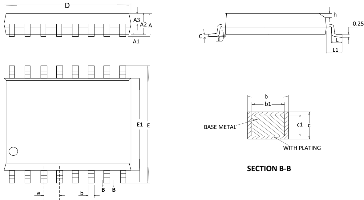
SSOP16 Package
