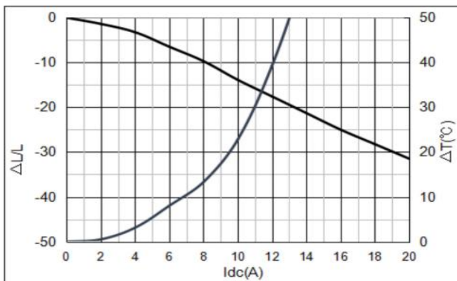
YSPI0520-R47M
