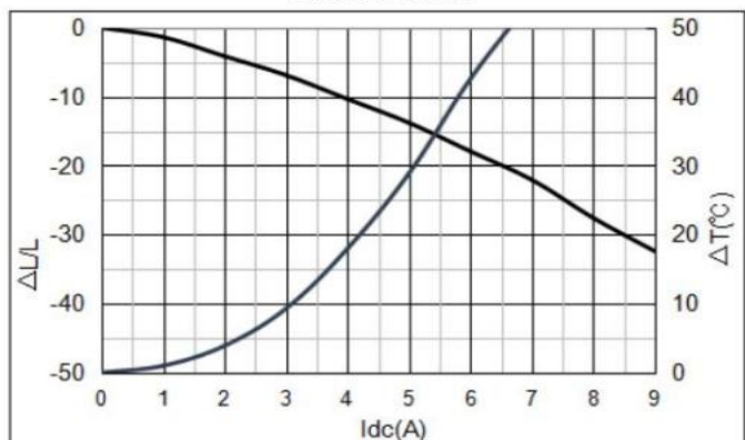
YSPI0520-3R3M
