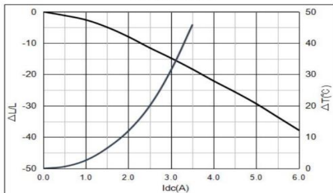
YSPI0520-6R8M
