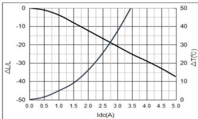
YSPI0520-6R8M
