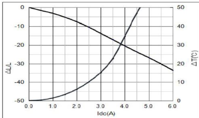
YSPI0840-470M
