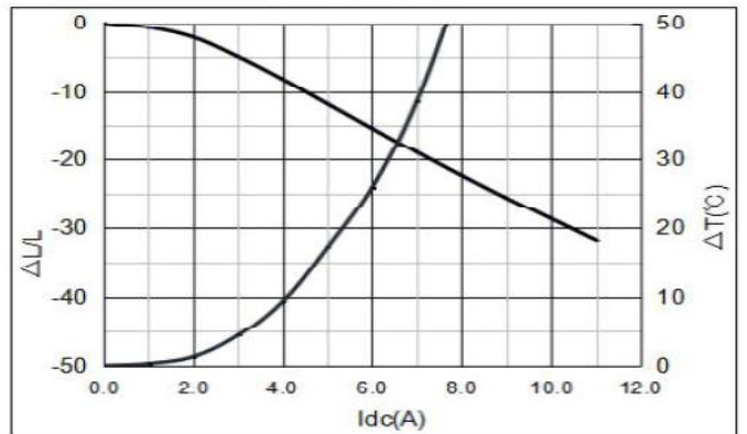
YSPI0840-150M
