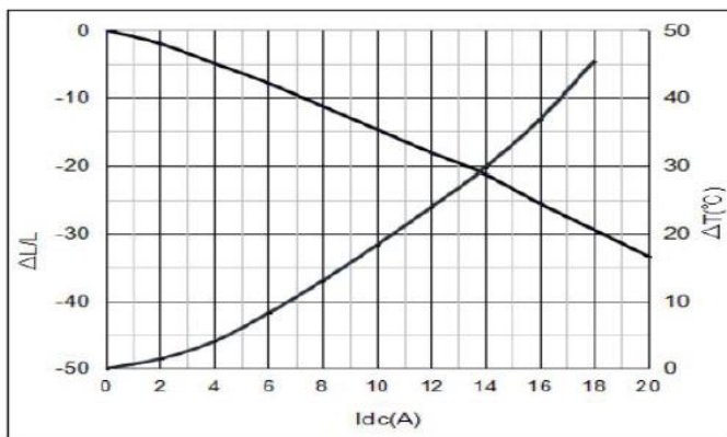
YSPI0840-2R2M
