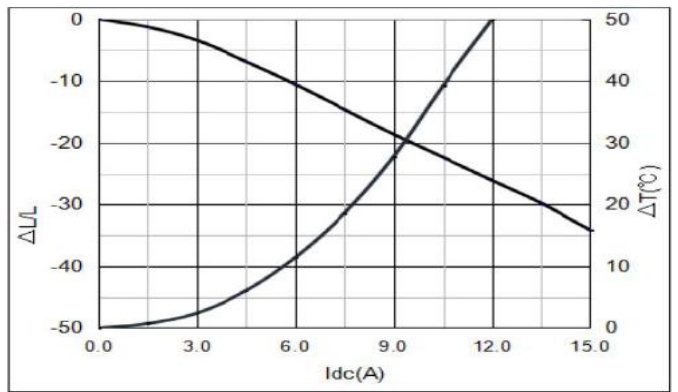
YSPI0840-6R8M
