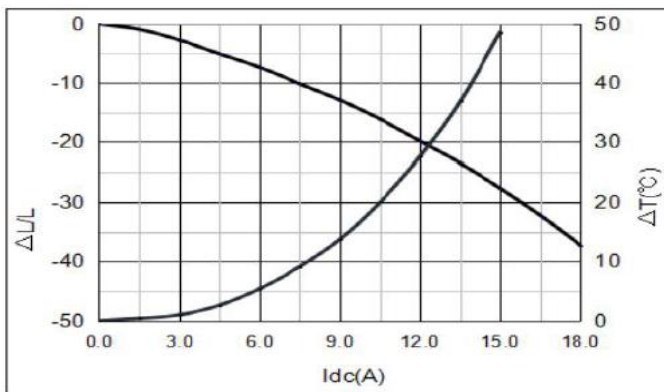
YSPI0840-4R7M
