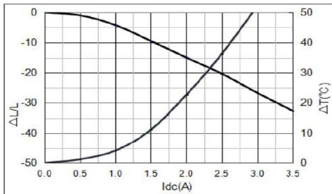
YSPI0840-470M
