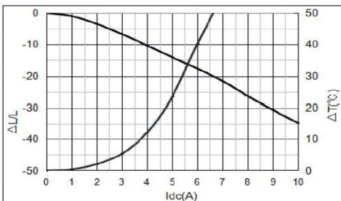
YSPI0840-100M
