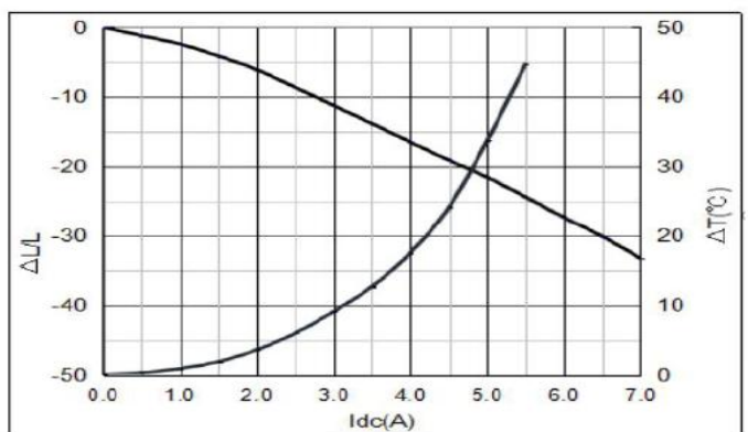
YSPI0840-150M
