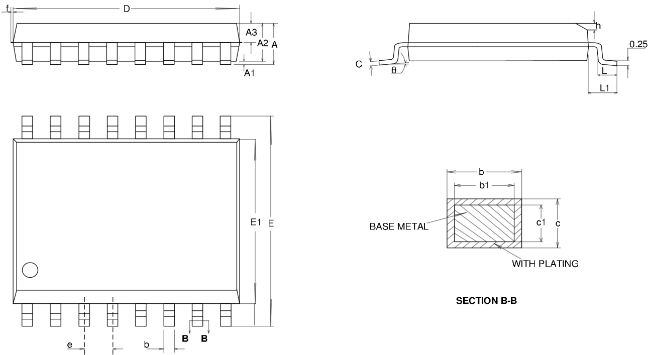
SSOP16 Package
