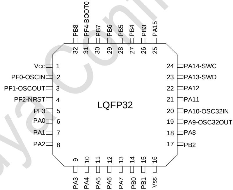
图 3-2 LQFP32 Pinout2 PY32F030K2xTx / PY32F030K2xT-E (Top view)
