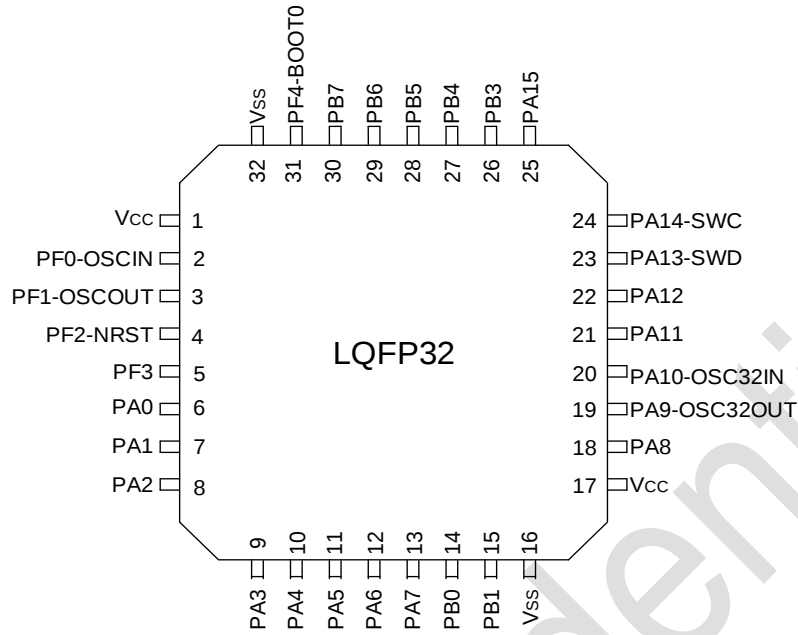
图 3-1 LQFP32 Pinout1 PY32F030K1xTx (Top view)
