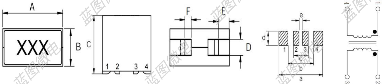
Recommended Land Pattern
