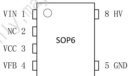
Fig2. Pin Definitions
