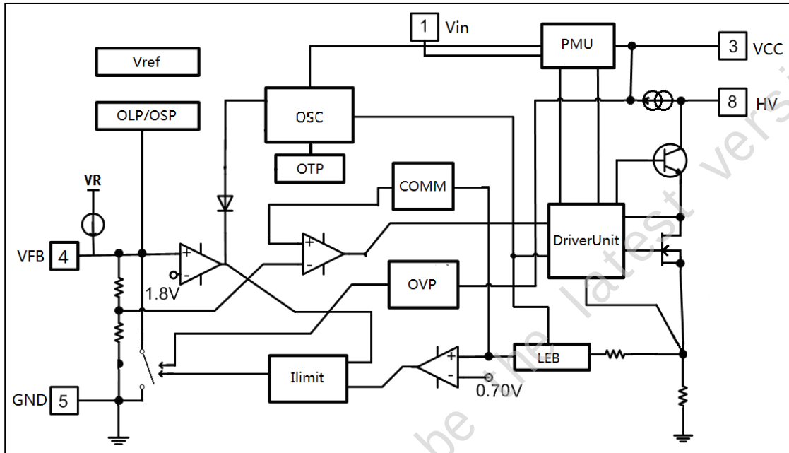
Fig1. Internal functional block diagram
