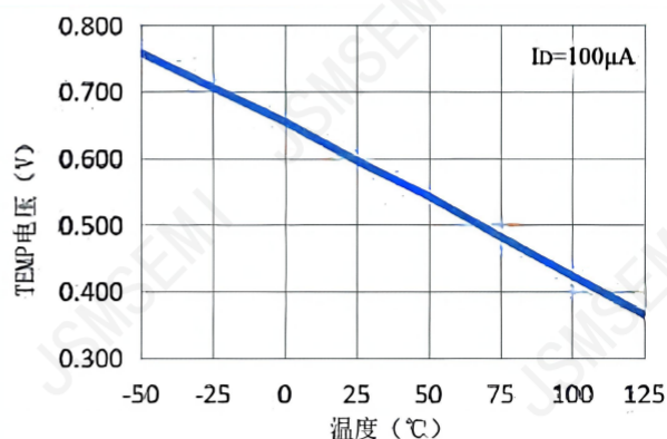
Figure 17. TEMP curve ( I_{temp}=100\mu A )
