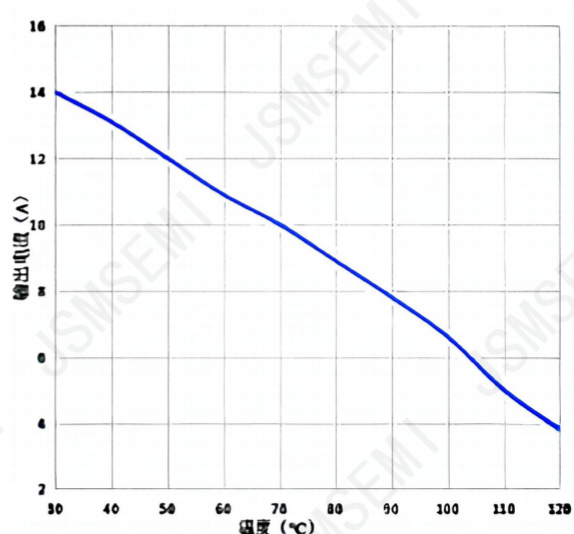
Figure 28. Four-channel Parallel Connection, CCM, 12V~5V Output Reference Derating Curve
