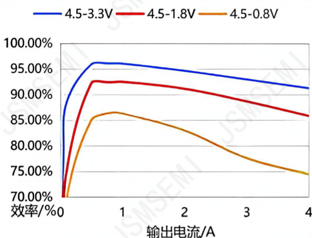
Figure 2. Efficiency curves for converting 4.5V input to 3.3V, 1.8V, and 0.8V
