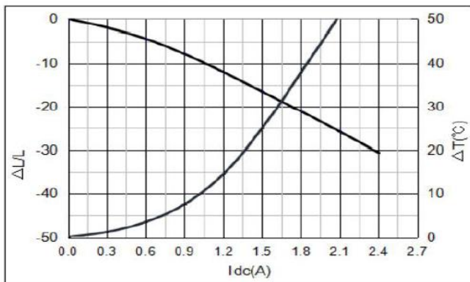
YSPI0420-100M
