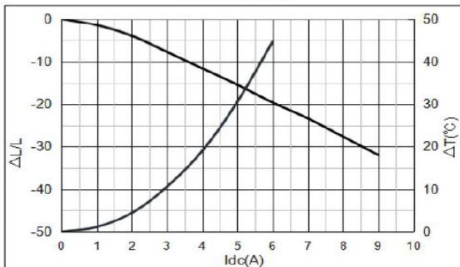
YSPI0420-R68M
