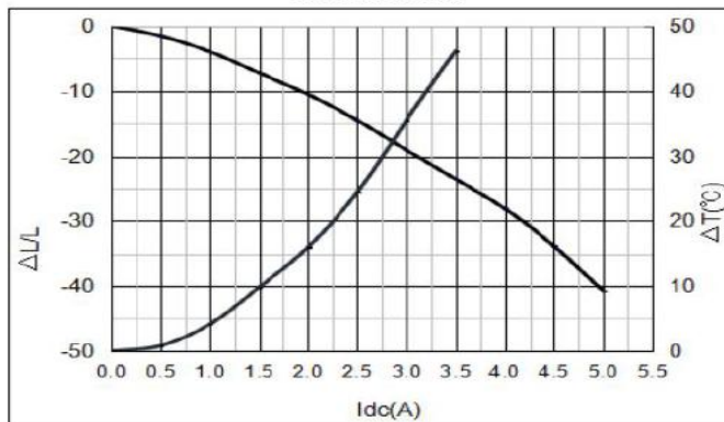
YSPI0420-3R3M
