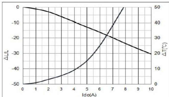
YSPI0420-R47M
