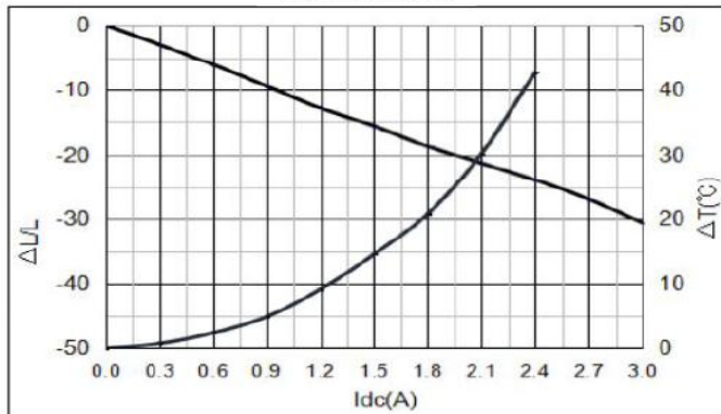
YSPI0420-100M
