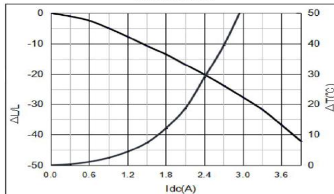
YSPI0420-5R6M
