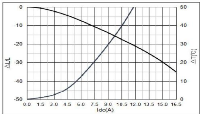
YSPI0530-R82M
