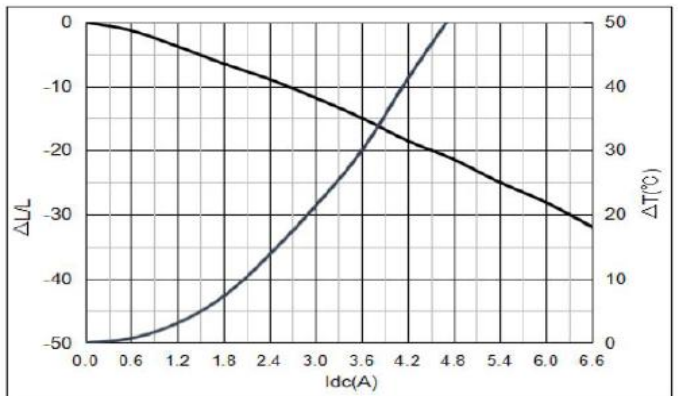
YSPI0530-4R7M
