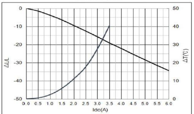
YSPI0530-100M
