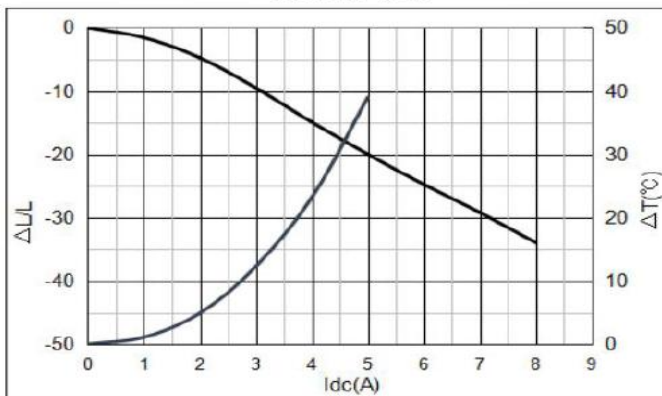
YSPI0530-3R3M
