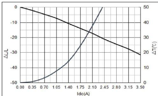
YSPI0530-150M
