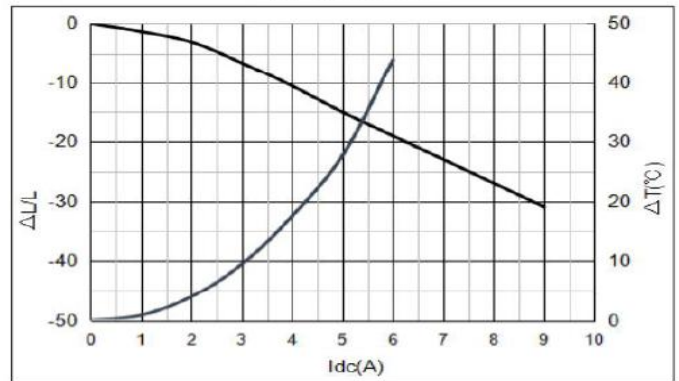
YSPI0530-4R7M
