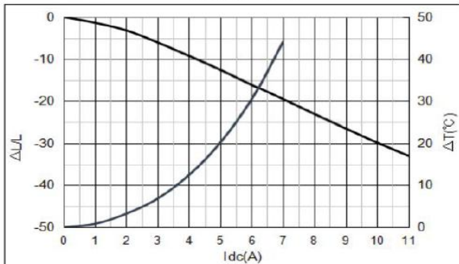
YSPI0530-3R3M
