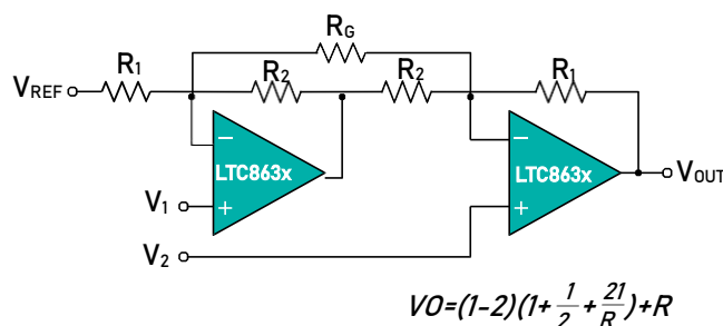
Figure 9: Instrumentation Amplifier
