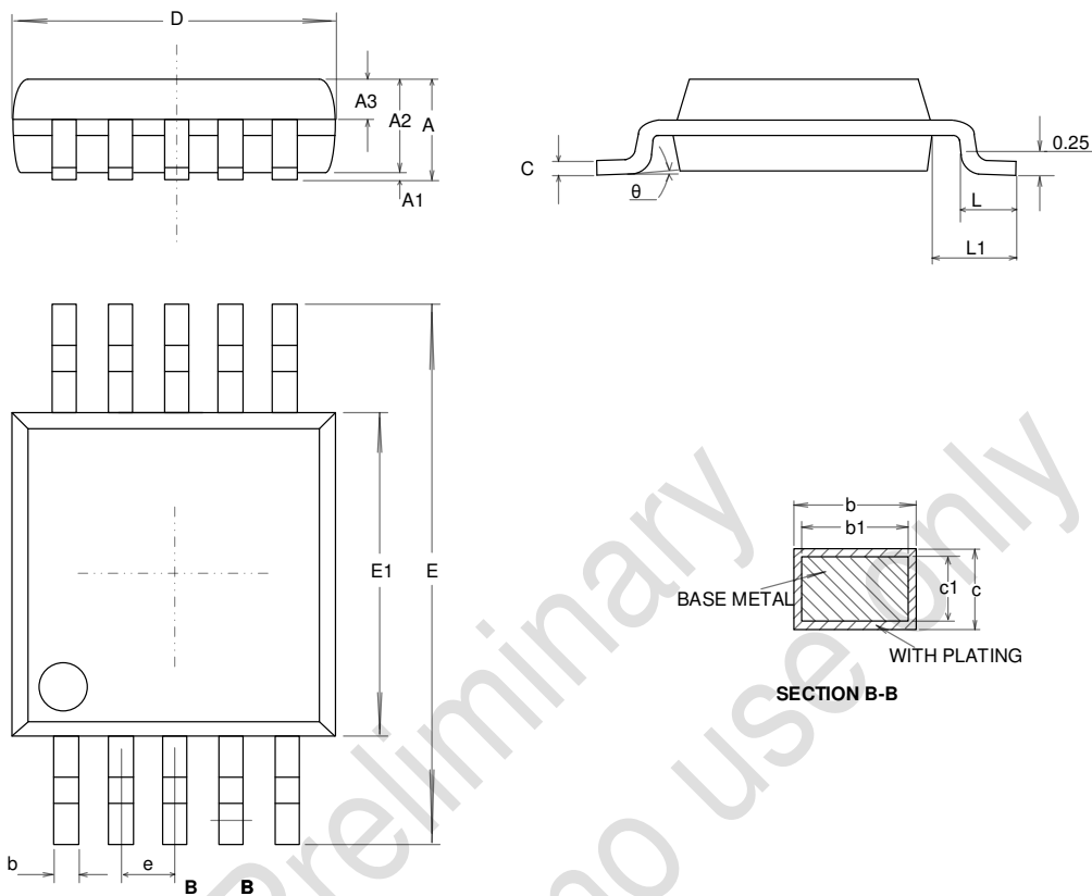
MSOP10L Package
