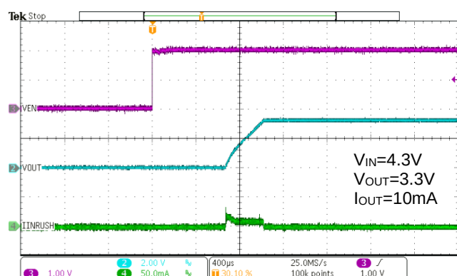
Figure 51. WR0306-33A50R Inrush Current
