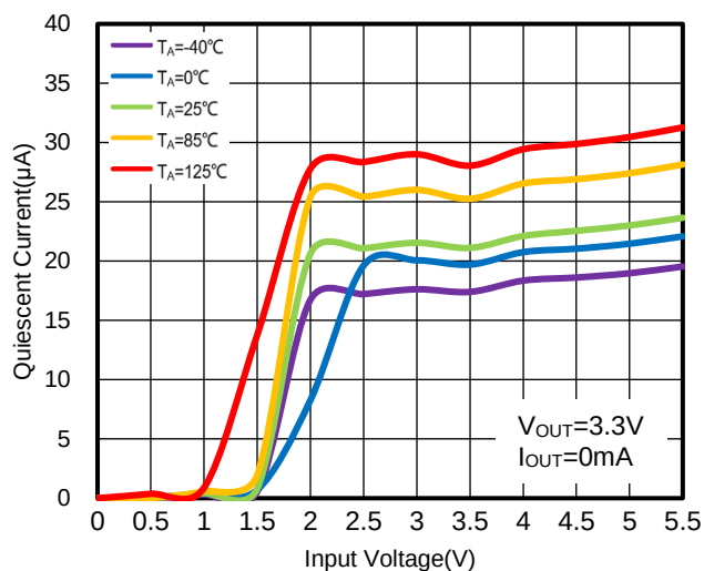
Figure 21. WR0306-33A50R Quiescent Current vs. Input Voltage
