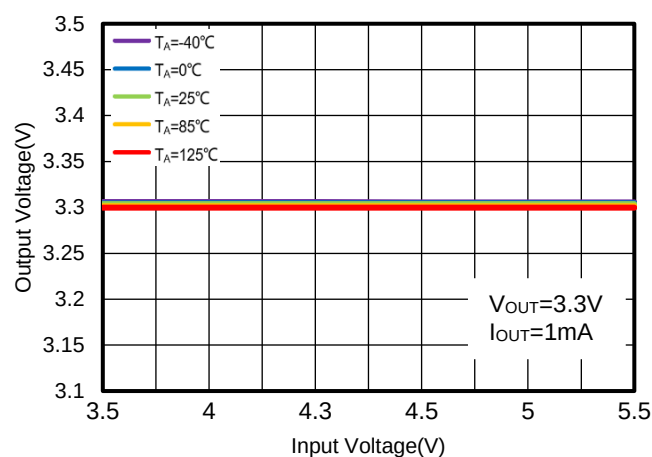
Figure 9. WR0306-33A50R Output Voltage vs. Input Voltage
