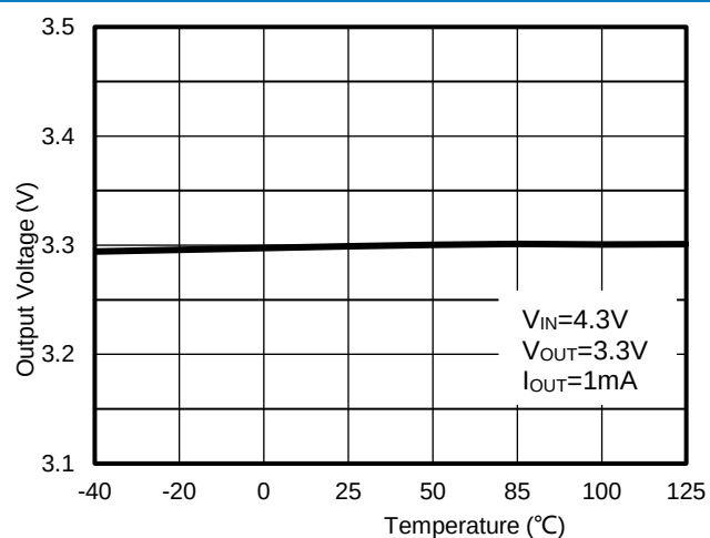
Figure 35. WR0306-33A50R Output Voltage vs. Ambient Temperature
