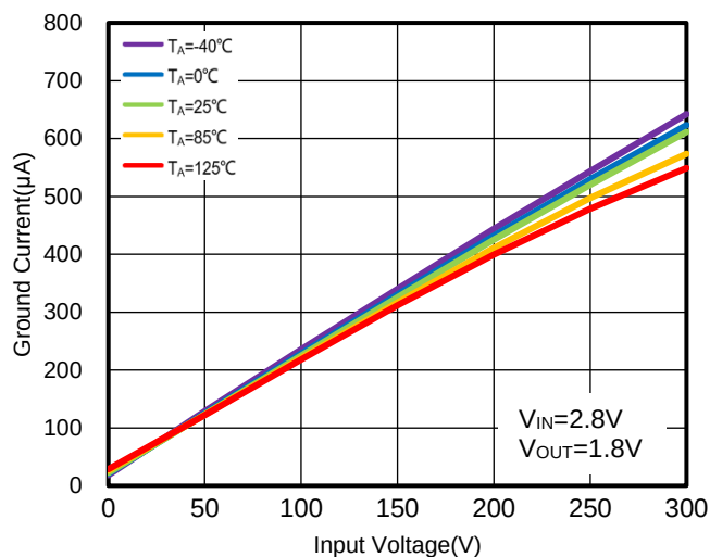
Figure 22. WR0306-18A50R Ground Current vs. Output Current
