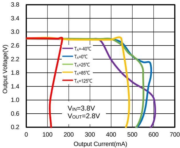
Figure 27. WR0306-28FF4R Current Limiting vs. Temperature
