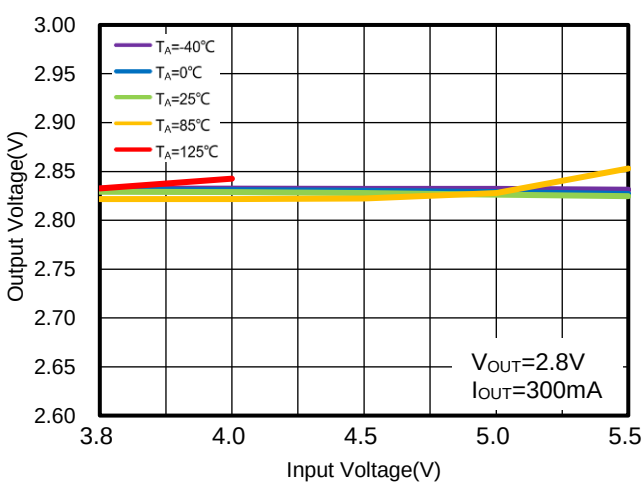
Figure 17. WR0306-28FF4R Output Voltage vs. Input Voltage
