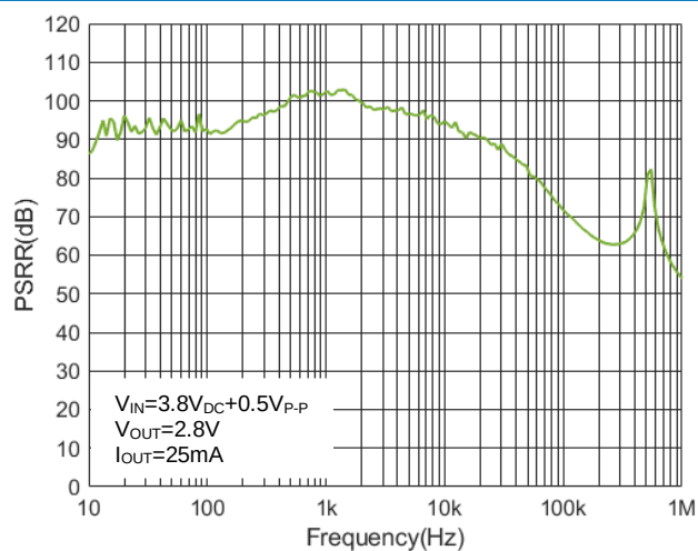
Figure 56. WR0306-28FF4R Power Supply Rejection Ratio vs. Frequency
