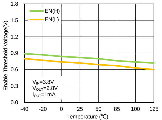
Figure 30. WR0306-28FF4R Enable Threshold Voltage vs. Temperature
