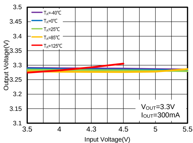
Figure 18. WR0306-33A50R Output Voltage vs. Input Voltage
