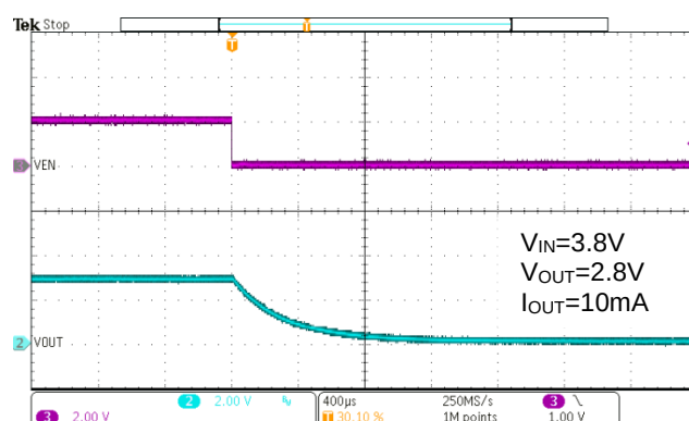
Figure 46. WR0306-28FF4R EN Shutdown
