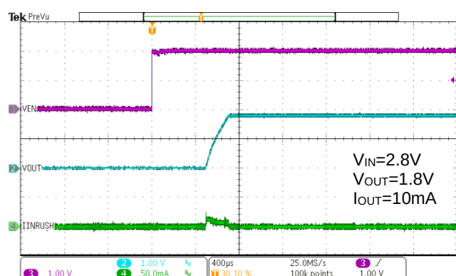
Figure 49. WR0306-18A50R Inrush Current
