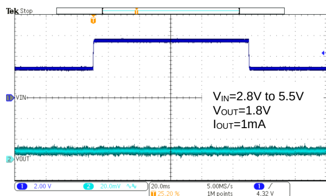
Figure 37. WR0306-18A50R Line Transient
