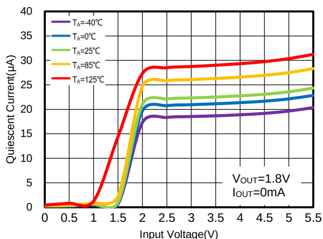
Figure 19. WR0306-18A50R Quiescent Current vs. Input Voltage
