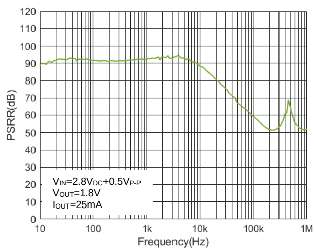
Figure 55. WR0306-18A50R Power Supply Rejection Ratio vs. Frequency
