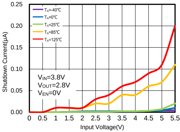
Figure 25. WR0306-28FF4R Shutdown Current vs. Input Voltage
