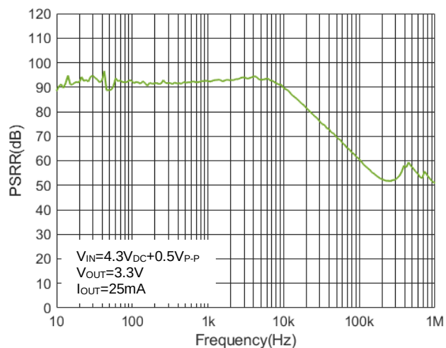
Figure 57. WR0306-33A50R Power Supply Rejection Ratio vs. Frequency
