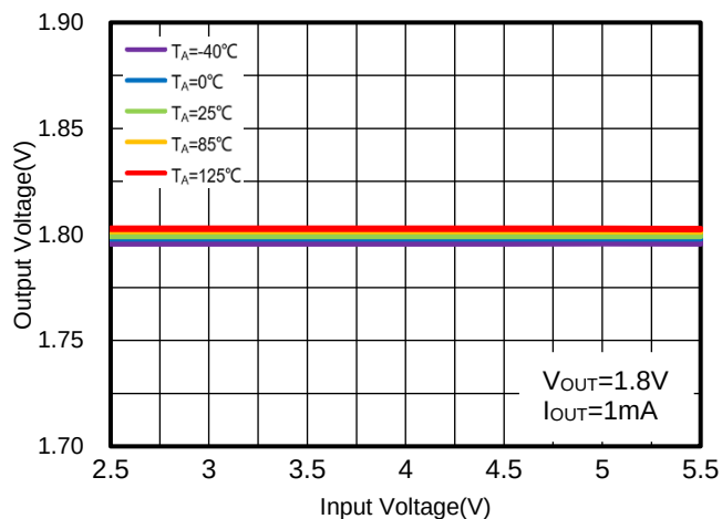
Figure 7. WR0306-18A50R Output Voltage vs. Input Voltage
