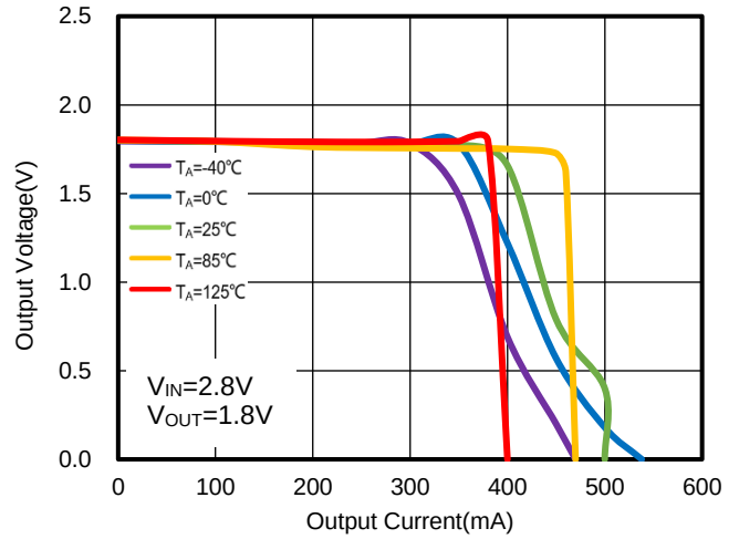
Figure 26. WR0306-18A50R Current Limiting vs. Temperature
