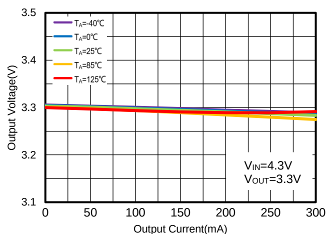
Figure 3. WR0306-33A50R Output Voltage vs. Output Current
