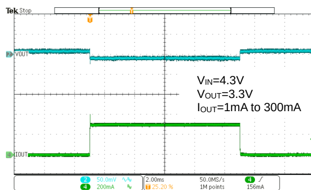
Figure 42. WR0306-33A50R Load Transient
