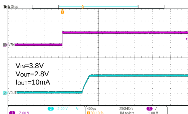
Figure 45. WR0306-28FF4R Soft Start from EN
