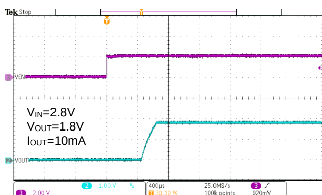
Figure 43. WR0306-18A50R Soft Start from EN
