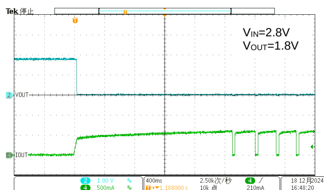
Figure 52. WR0306-18A50R Circuit Limiting and Thermal Shutdown
