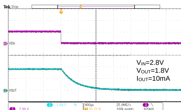
Figure 44. WR0306-18A50R EN Shutdown
