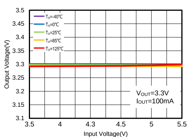
Figure 12. WR0306-33A50R Output Voltage vs. Input Voltage
