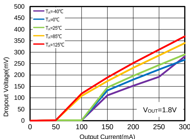
Figure 4. WR0306-18A50R Dropout Voltage vs. Output Current
