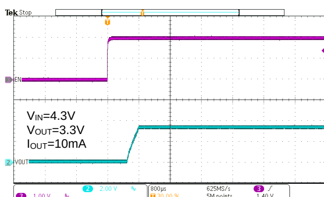
Figure 47. WR0306-33A50R Soft Start from EN
