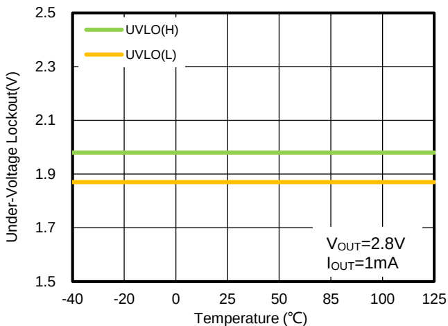
Figure 29. WR0306-28FF4R Under-Voltage Lockout Voltage vs. Temperature
