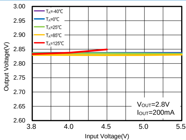
Figure 14. WR0306-28FF4R Output Voltage vs. Input Voltage
