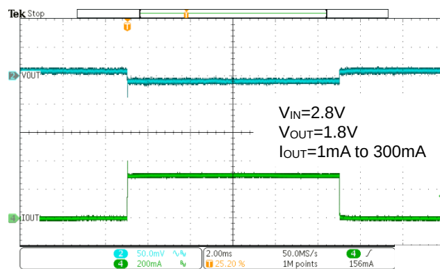
Figure 40. WR0306-18A50R Load Transient
