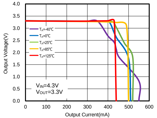
Figure 28. WR0306-33A50R Current Limiting vs. Temperature
