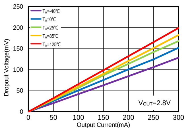
Figure 5. WR0306-28FF4R Dropout Voltage vs. Output Current
