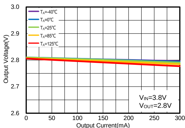
Figure 2. WR0306-28FF4R Output Voltage vs. Output Current
