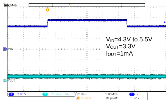
Figure 39. WR0306-33A50R Line Transient
