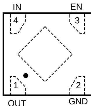
DFN1010-4
