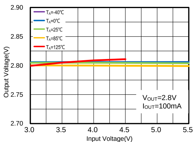
Figure 11. WR0306-28FF4R Output Voltage vs. Input Voltage
