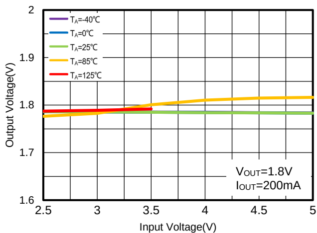
Figure 13. WR0306-18A50R Output Voltage vs. Input Voltage
