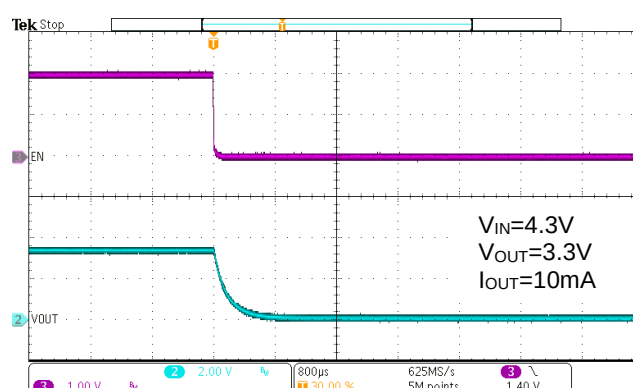
Figure 48. WR0306-33A50R EN Shutdown
