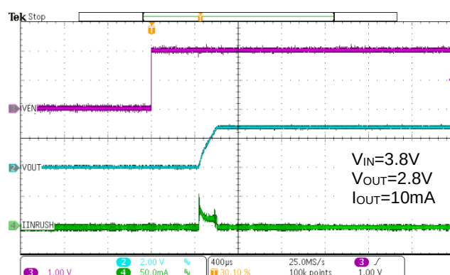
Figure 50. WR0306-28FF4R Inrush Current
