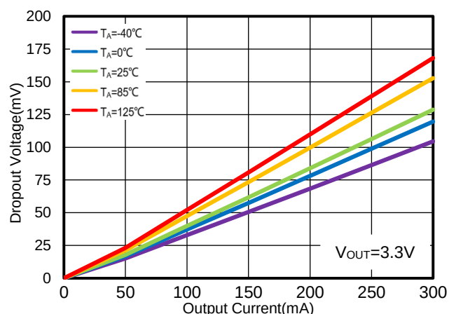
Figure 6. WR0306-33A50R Dropout Voltage vs. Output Current
