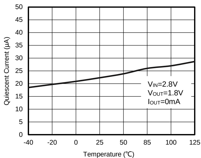
Figure 32. WR0306-18A50R Quiescent Current vs. V_{IN} & Ambient Temperature
