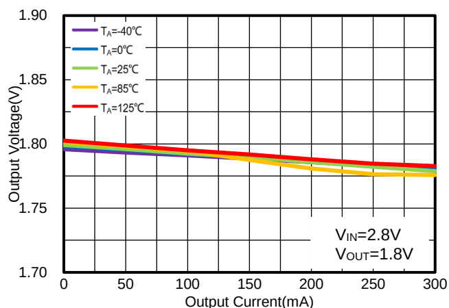
Figure 1. WR0306-18A50R Output Voltage vs. Output Current
