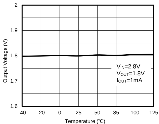
Figure 31. WR0306-18A50R Output Voltage vs. Ambient Temperature
