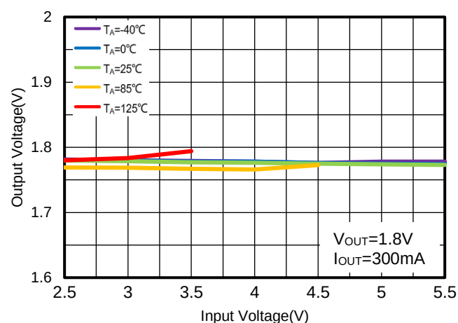
Figure 16. WR0306-18A50R Output Voltage vs. Input Voltage
