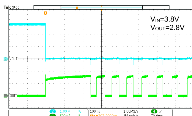
Figure 53. WR0306-28FF4R Circuit Limiting and Thermal Shutdown
