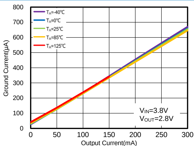
Figure 23. WR0306-28FF4R Ground Current vs. Output Current
