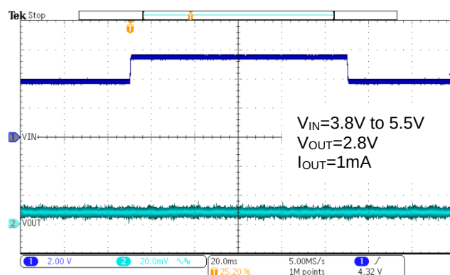
Figure 38. WR0306-28FF4R Line Transient
