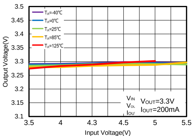
Figure 15. WR0306-33A50R Output Voltage vs. Input Voltage
