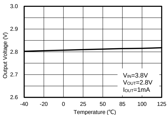
Figure 33. WR0306-28FF4R Output Voltage vs. Ambient Temperature
