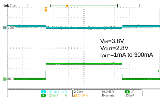
Figure 41. WR0306-28FF4R Load Transient
