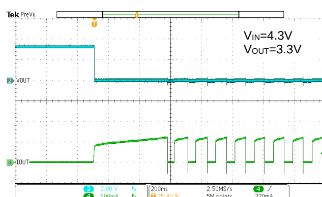
Figure 54. WR0306-33A50R Circuit Limiting and Thermal Shutdown
