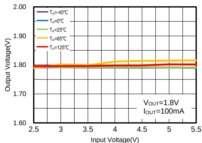
Figure 10. WR0306-18A50R Output Voltage vs. Input Voltage
