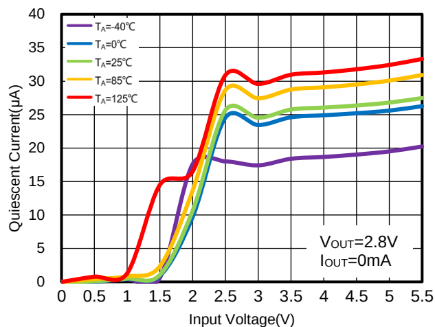
Figure 20. WR0306-28FF4R Quiescent Current vs. Input Voltage
