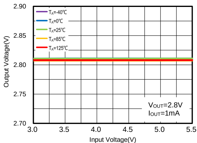
Figure 8. WR0306-28FF4R Output Voltage vs. Input Voltage
