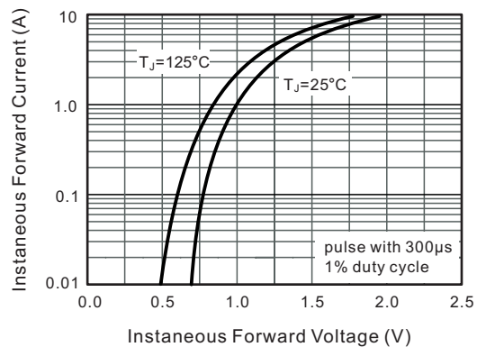
FIG.2-TYPICAL FORWARD CHARACTERISTICS
