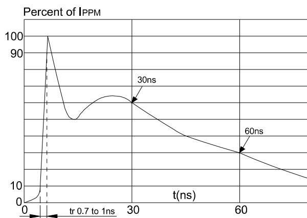
FIG.4: ESD clamping
