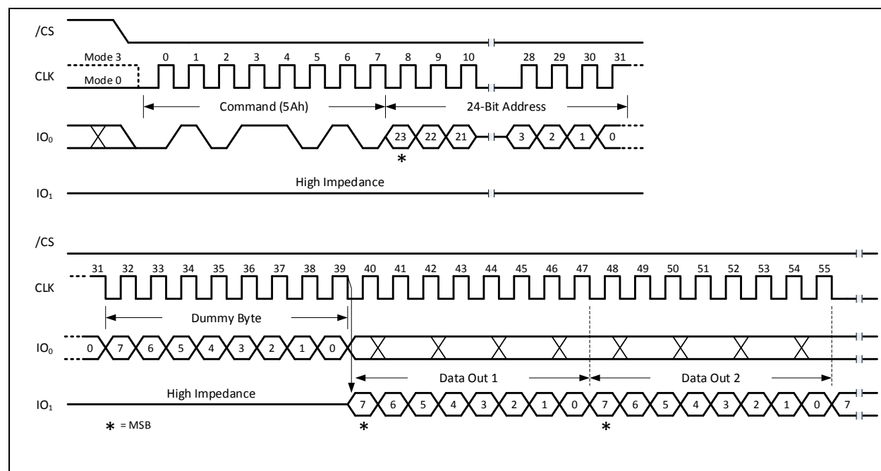
Figure 7-2a. Read SFDP Register Command Sequence (SDR Mode)
