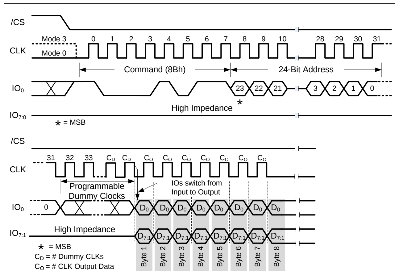
Figure 10-5. Fast Read Octal Output Command (1-1-8 SDR Mode) A 32-Bit Address is required when the device is operating in 4-Byte Address Mode
