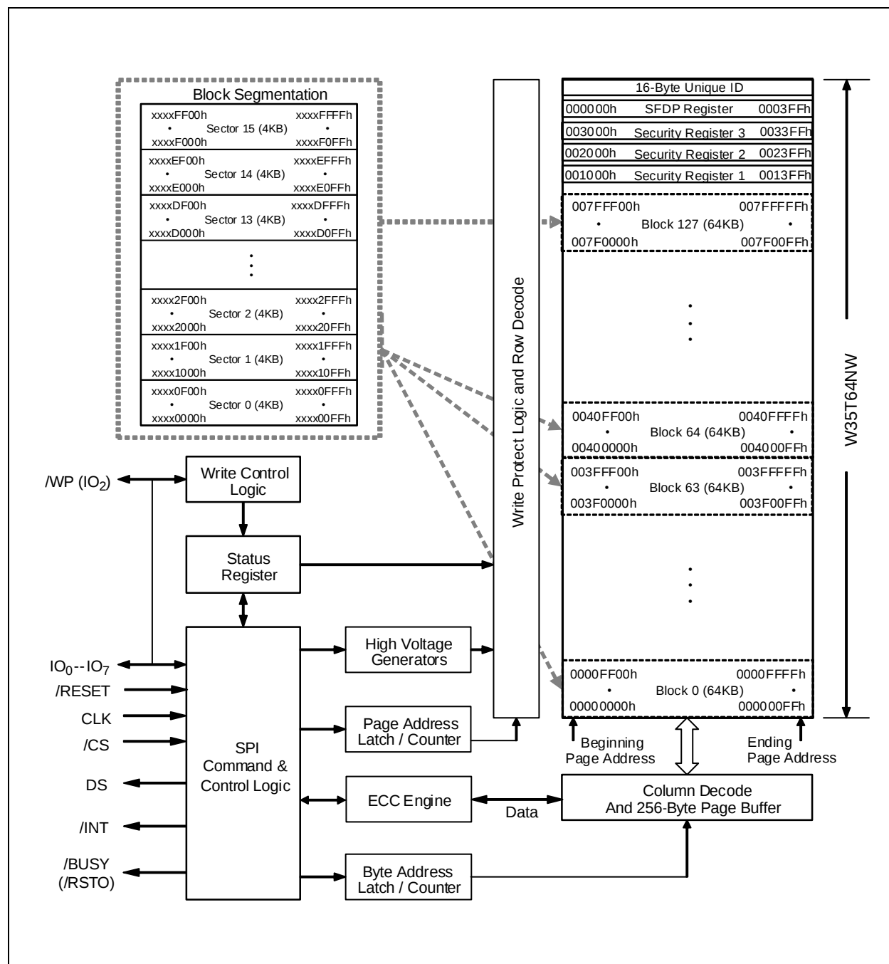
Figure 1. W35T64NW Serial Flash Memory Block Diagram
