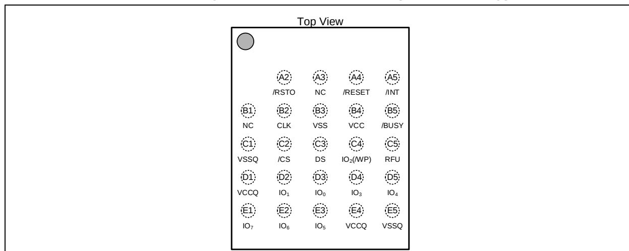
Figure 3-2. W35T64NW Ball Assignments, 24-ball (5x5 ball array) TFBGA 6x8-mm (Package Code TB)
