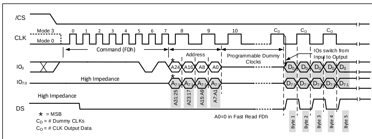
Figure 10-10. Fast Read DDR Octal I/O with 4-Byte Address (1-8d SDR Mode)
