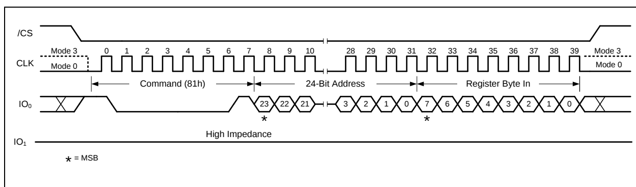
Figure 8-8a. Write Volatile Configuration Register Command (SDR Mode) A 32-Bit Address is required when the device is operating in 4-Byte Address Mode
