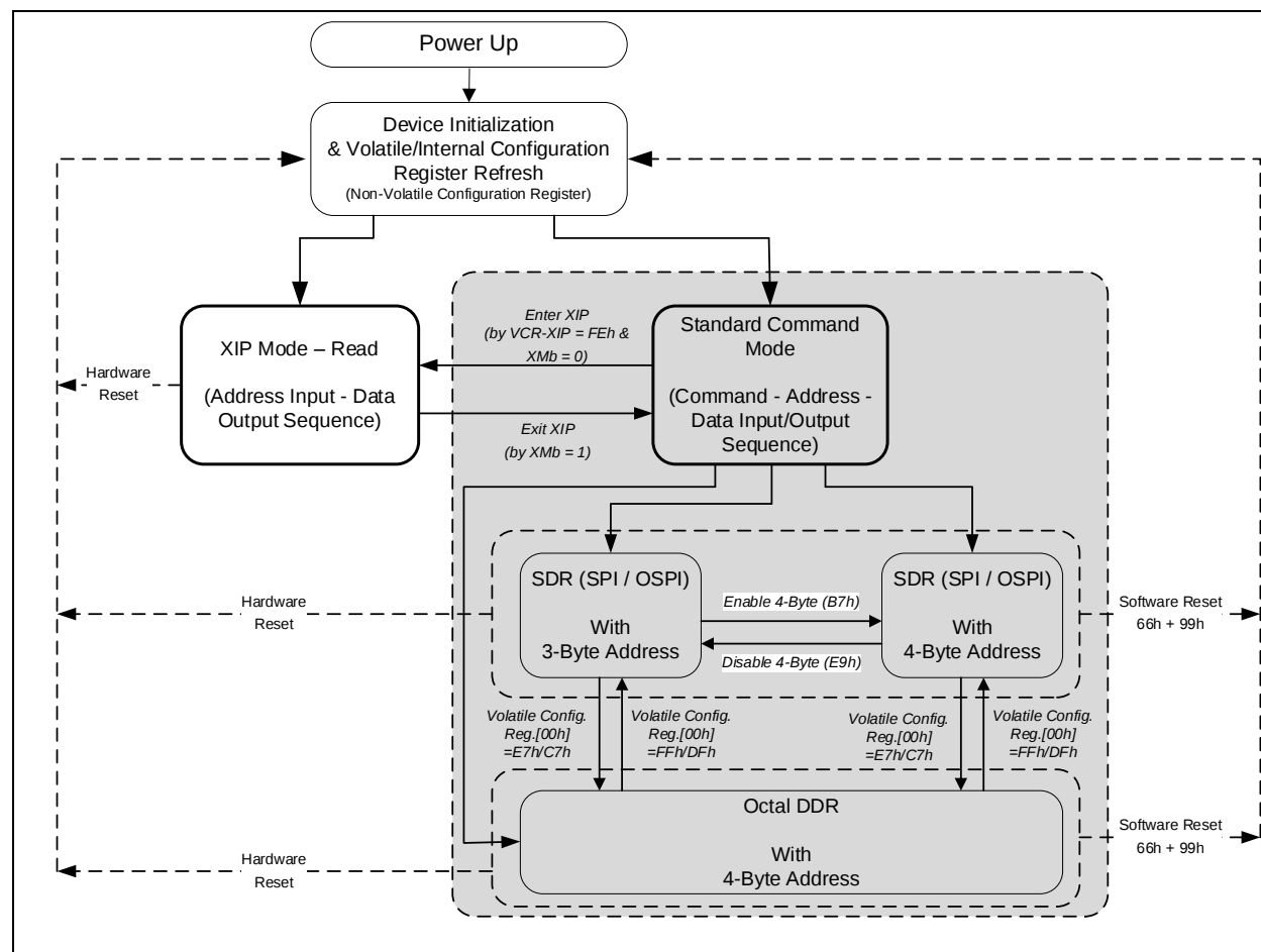
Figure 4-1. W35T64NW Serial Flash Memory Operation Diagram
