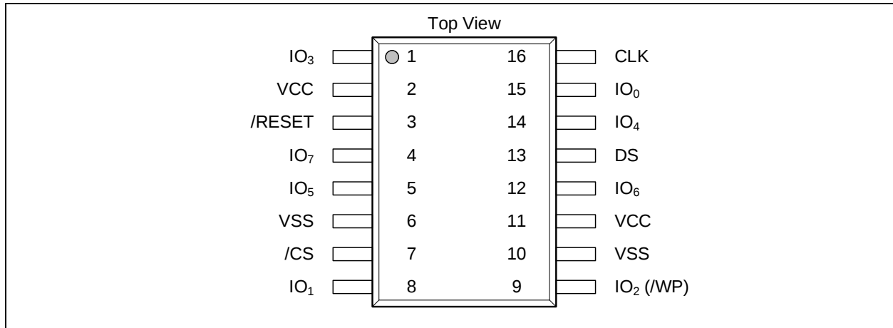
Figure 3-1. W35T64NW Industrial Grade Pin Assignments, 16-pin SOIC 300-mil (Package Code SF)
