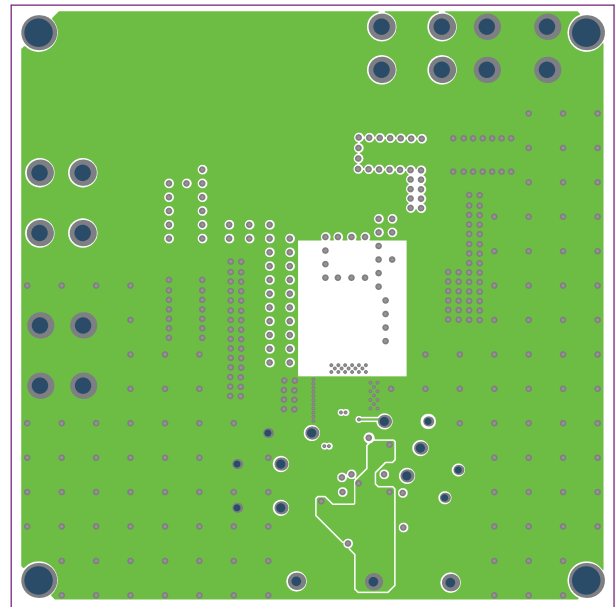
Figure 6: Mid-Layer 2
