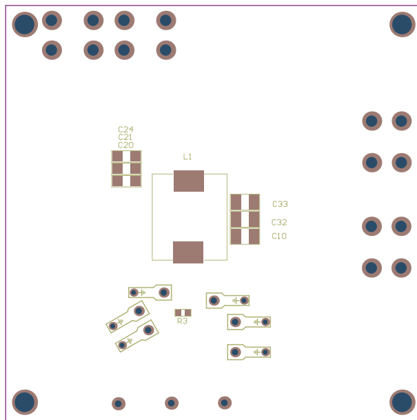
Figure 8: Bottom Silk
