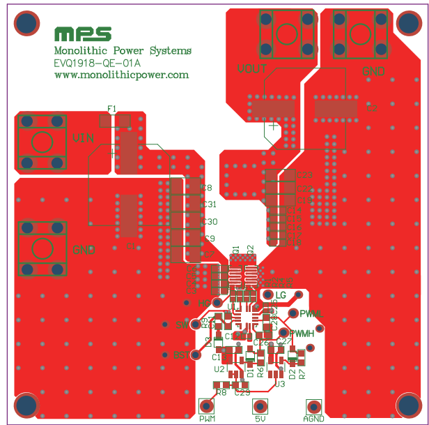
Figure 4: Top Layer
