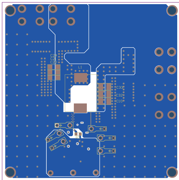
Figure 7: Bottom Layer
