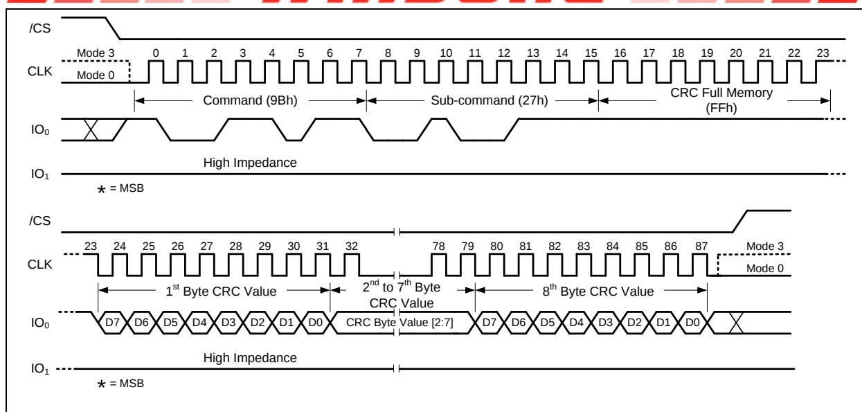
Figure 19-1a. CRC-At-Rest Full Memory Command Sequence (SDR Mode)
