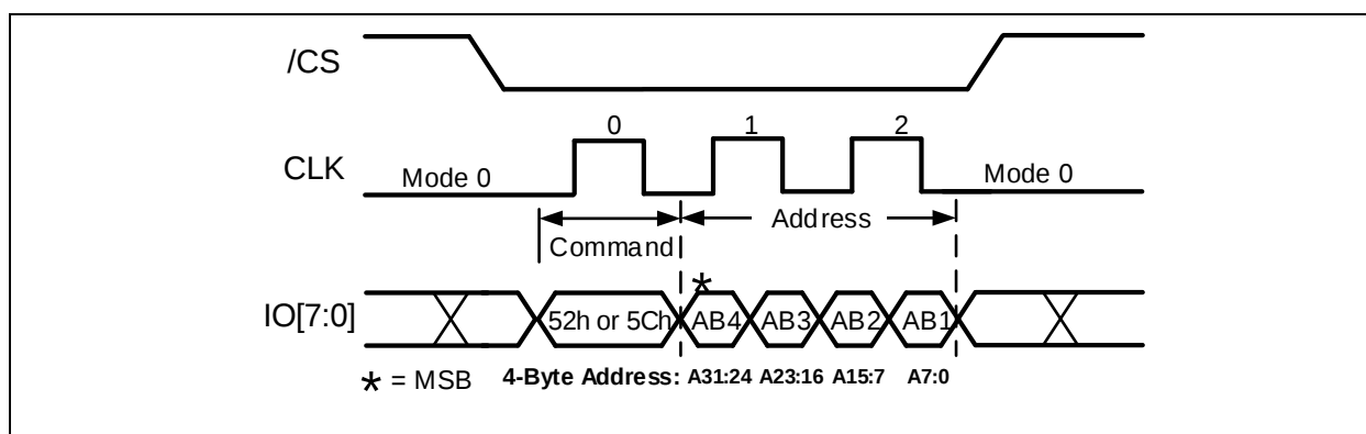
Figure 12-6. 32KB Block Erase Command (ODDR Mode)
