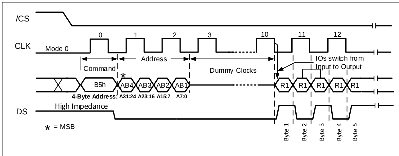
Figure 8-5b. Read Non-Volatile Configuration Register Command (ODDR Mode)
