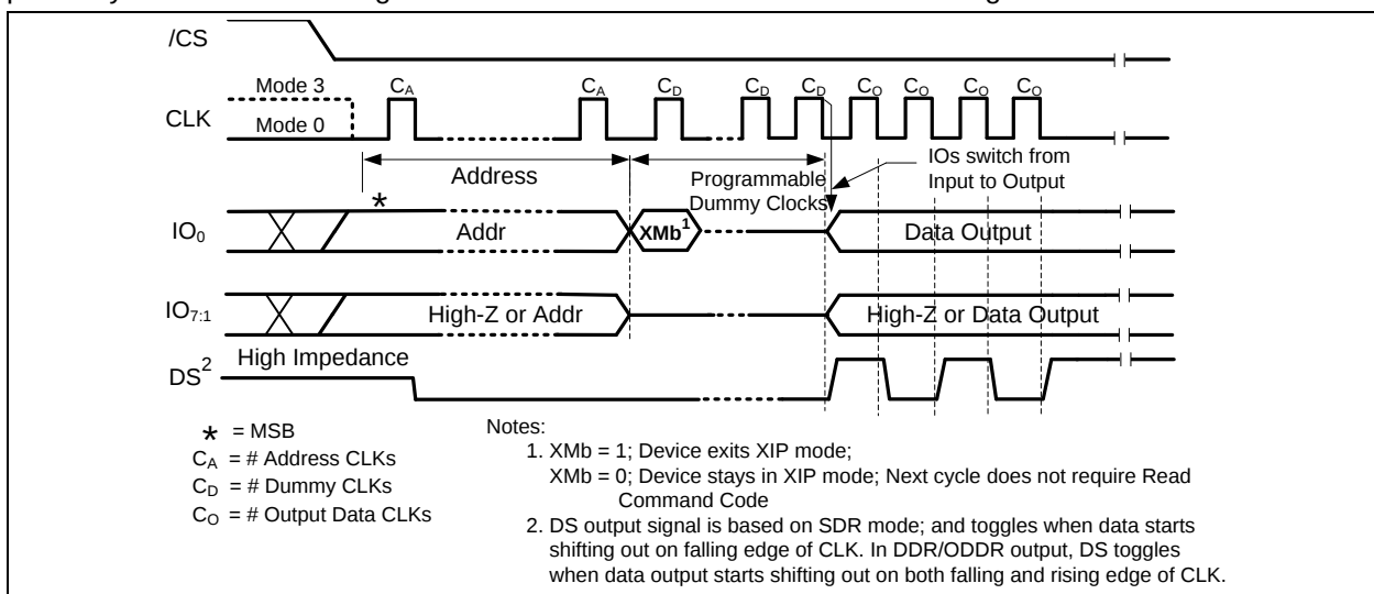
Figure 4-2. XIP Mode Entry from Non-Volatile Configuration Register Address 06h (NVCR-XIP)
