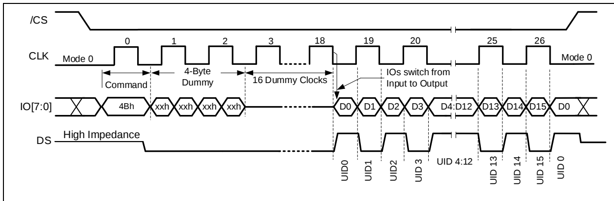
Figure 15-1b. Read Unique ID Command (ODDR Mode)
