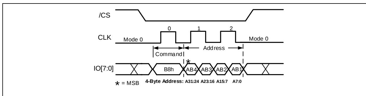
Figure 18-6b. (8d-8d-0) Erase DLP Register Command (8d-8d-0 ODDR Mode)
