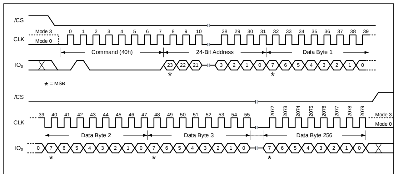
Figure 18-4. Program Tuning Data Pattern Command (1-1-1 SDR Mode) A 32-Bit Address is required when the device is operating in 4-Byte Address Mode
