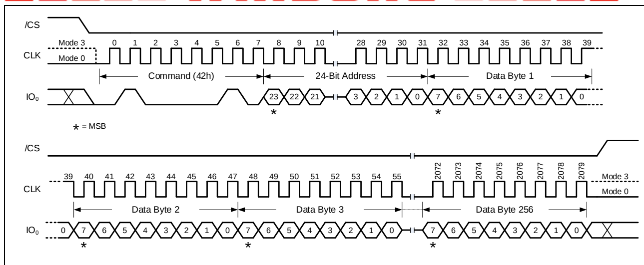
Figure 15-3a. Program Security Registers Command (SDR Mode)
