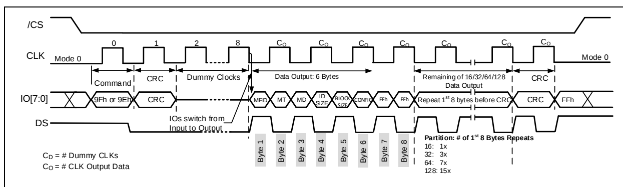
Figure 19-4f. 8d-8d-8d Read ID CRC-In-Transit Command Protocol (ODDR Mode)
