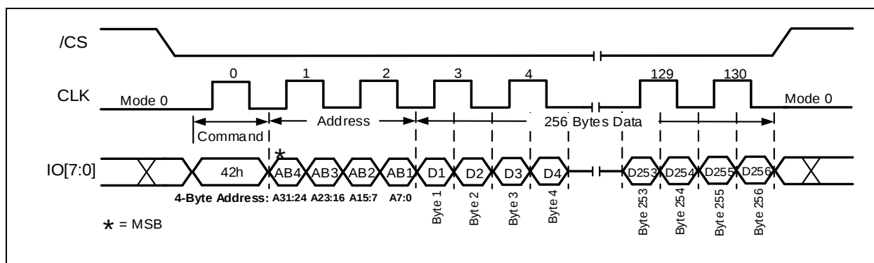
Figure 15-3b. Program Security Registers Command (ODDR Mode)
