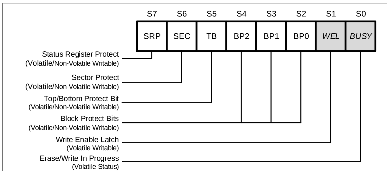
Figure 5-1. Status Register
