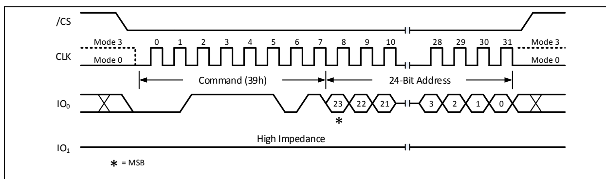
Figure 14-5a. Individual Block/Sector Unlock Command (SDR Mode)
