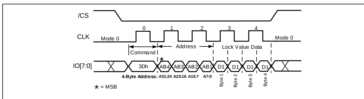
Figure 14-3b. Read Block/Sector Lock Command (ODDR Mode)
