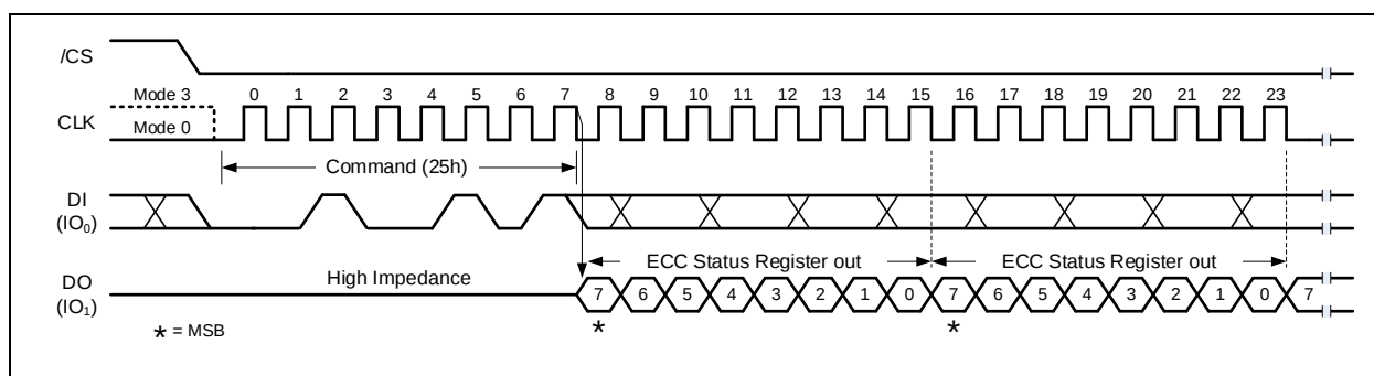
Figure 17-1a. Read ECC Status Register Command (SDR Mode)
