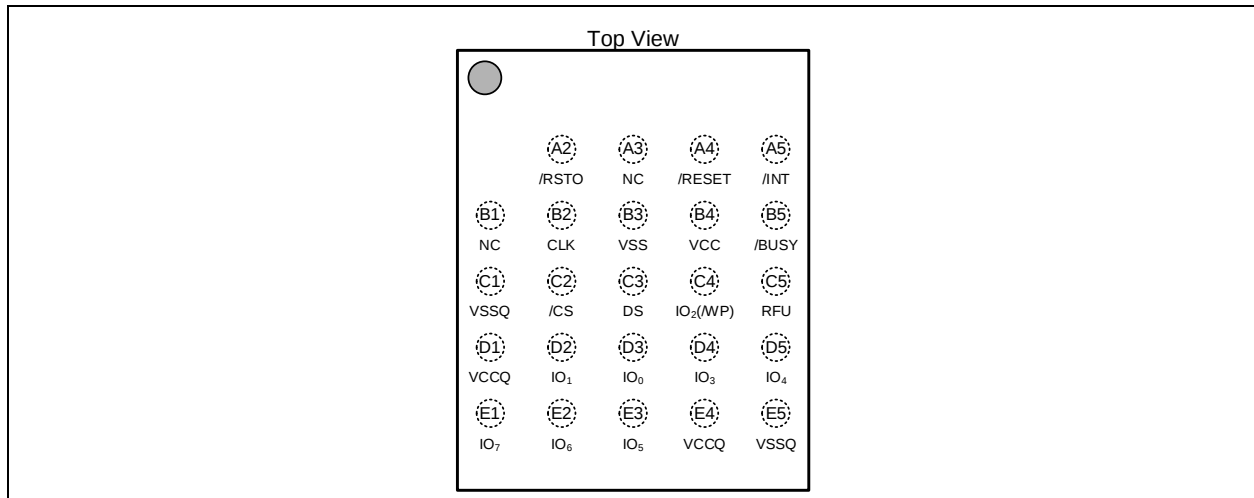
Figure 3-2. W35T12NW Ball Assignments, 24-ball (5x5 ball array) TFBGA 6x8-mm (Package Code TB)
