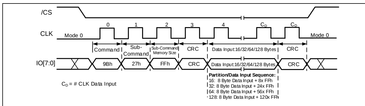
Figure 19-4i. CRC-In-Transit 8d-8d-8d CRC-At-Rest Full Memory Command Protocol (ODDR Mode)
