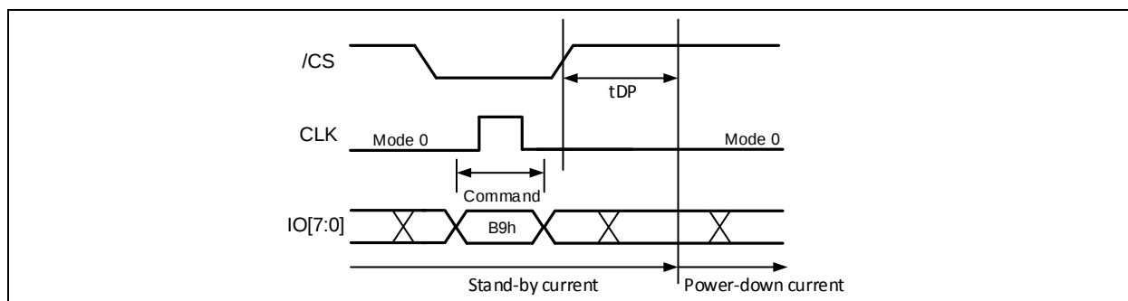
Figure 16-1b. Deep Power-down Command (ODDR Mode)
