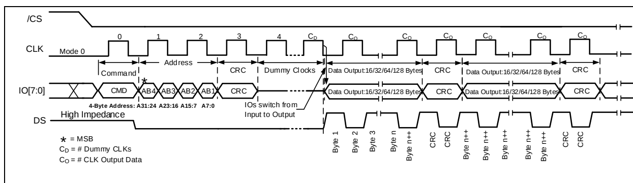
Figure 19-4g. CRC-In-Transit 8d-8d-8d Read SFDP Command Protocol (ODDR Mode)
