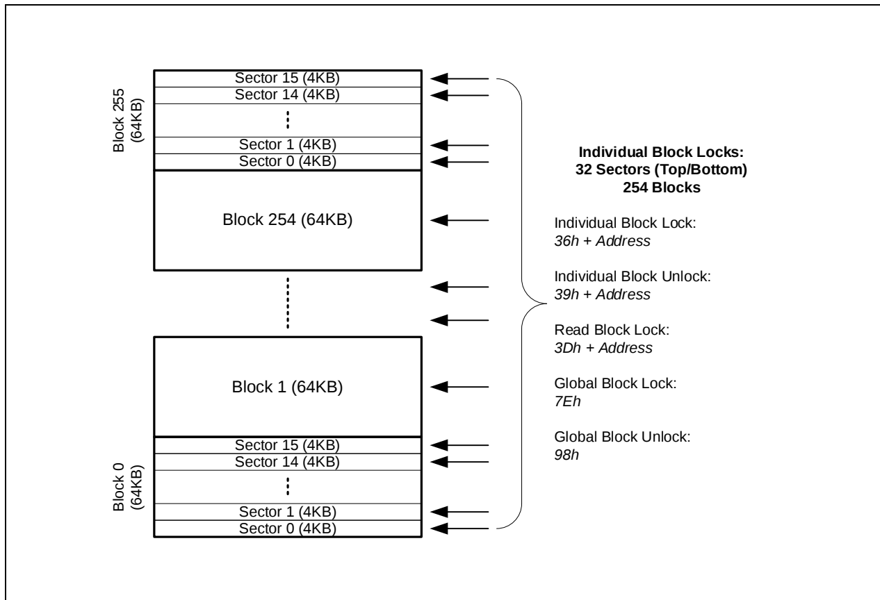
Figure 5-2. Individual Block/Sector Locks
