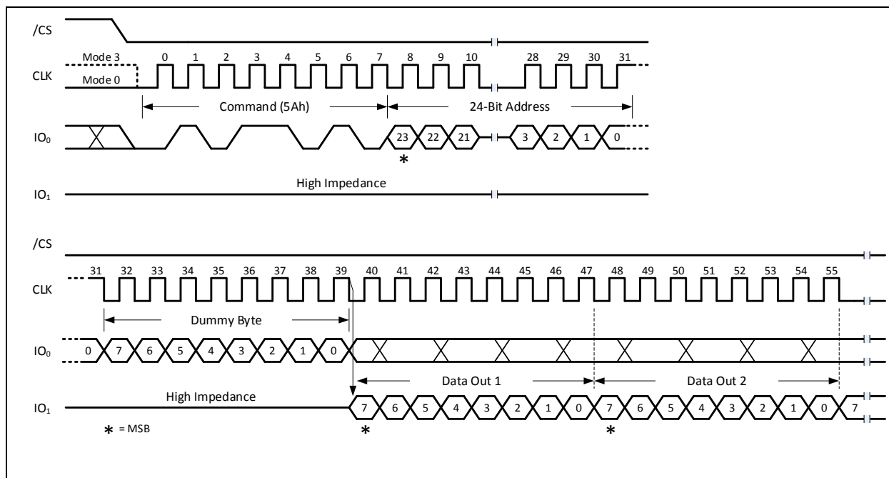
Figure 7-2a. Read SFDP Register Command Sequence (SDR Mode) A 24-Bit Address input only even when device is operating in 4-Byte Address Mode
