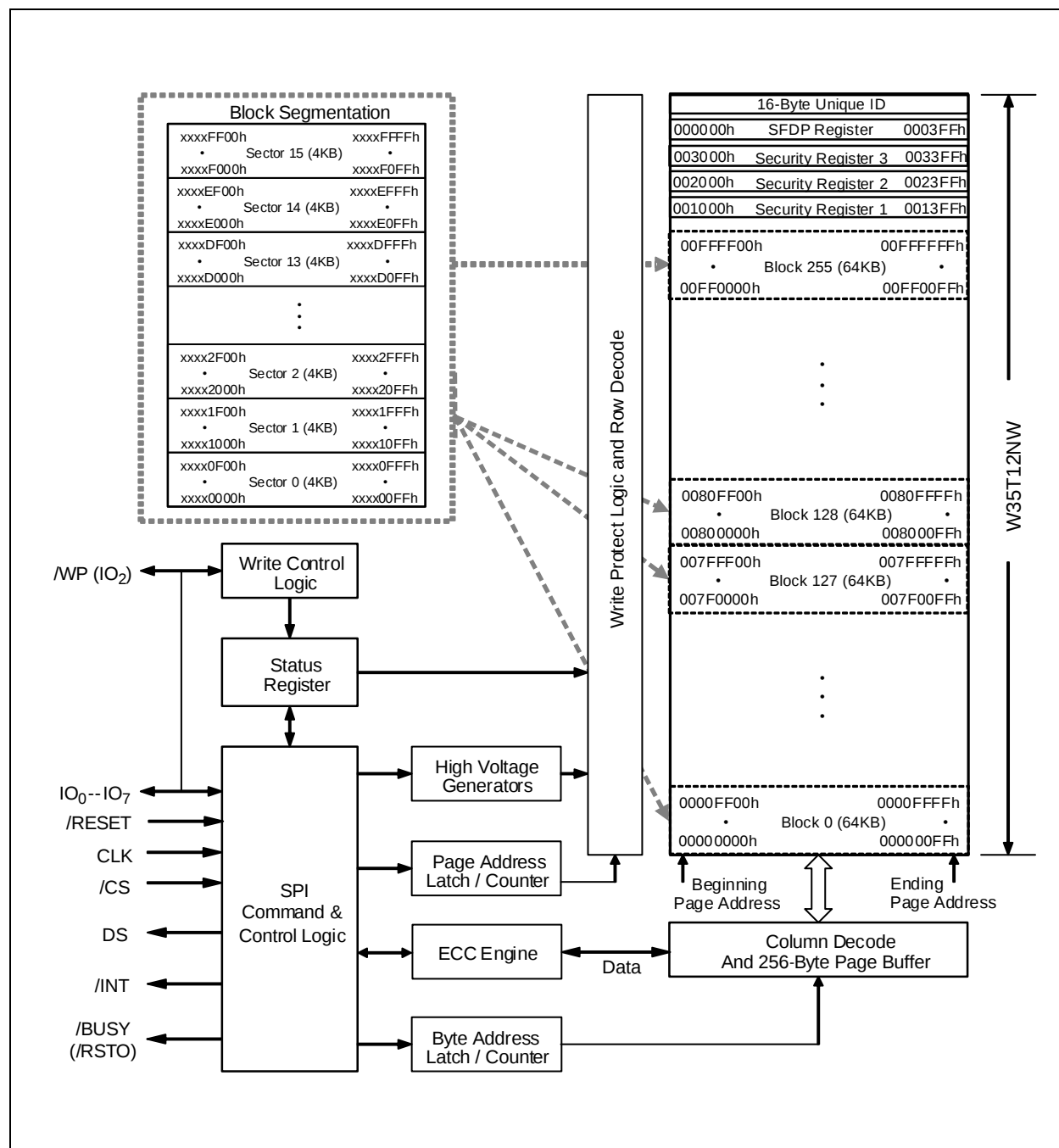
Figure 1. W35T12NW Serial Flash Memory Block Diagram
