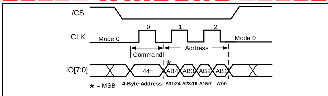
Figure 15-2b. Erase Security Registers Command (ODDR Mode)
