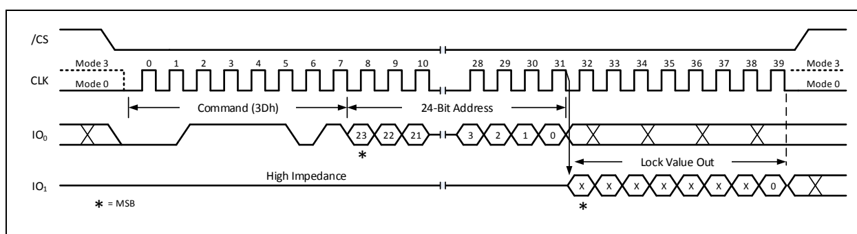
Figure 14-3a. Read Block/Sector Lock Command (SDR Mode)
