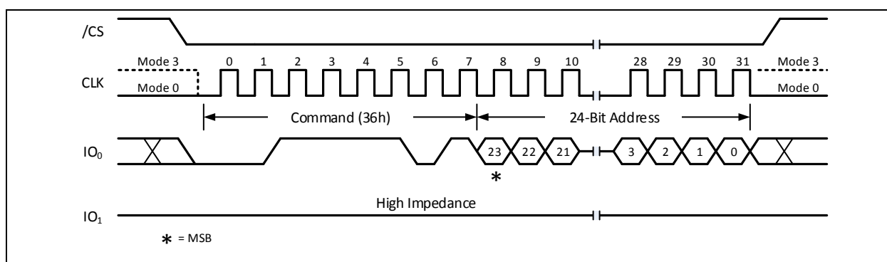
Figure 14-4a. Individual Block/Sector Lock Command (SDR Mode)
