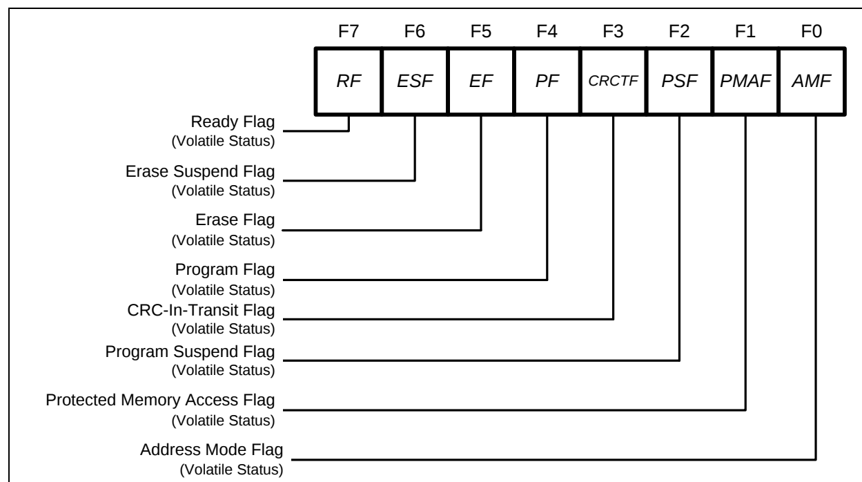
Figure 5-3. Flag Register
