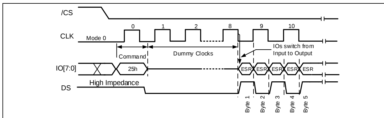
Figure 17-1b. Read ECC Status Register Command (ODDR Mode)
