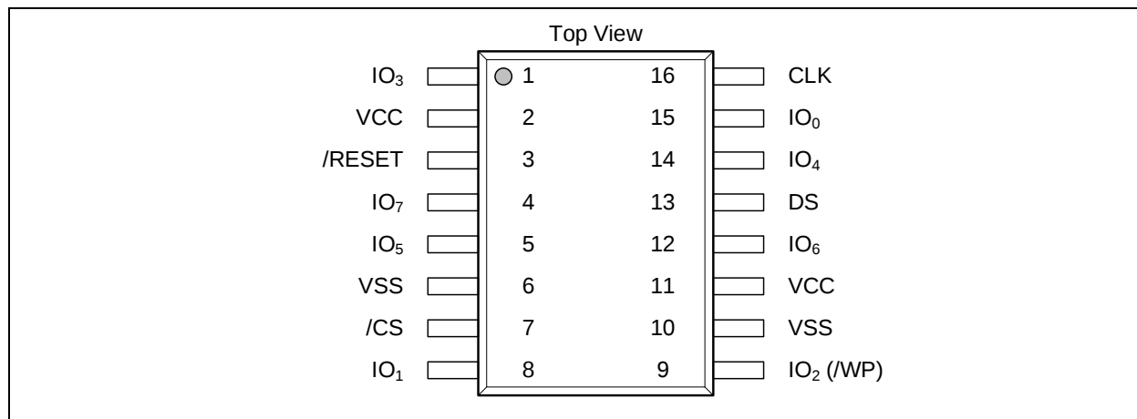
Figure 3-1. W35T12NW Industrial Grade Pin Assignments, 16-pin SOIC 300-mil (Package Code SF)
