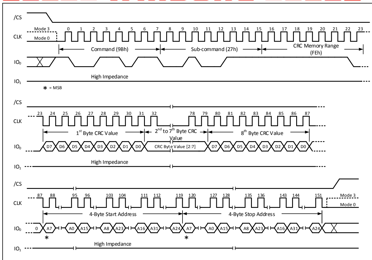
Figure 19-2a. CRC-At-Rest Memory Range Command Sequence (SDR Mode)
