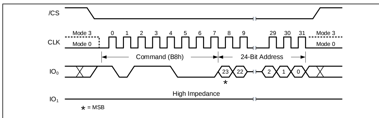
Figure 18-6a. (1-1-0) Erase DLP Register Command (1-1-0 SDR Mode) A 32-Bit Address is required when the device is operating in 4-Byte Address Mode
