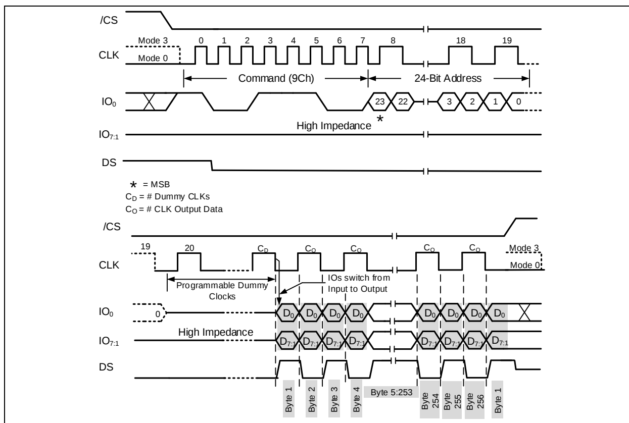
Figure 18-3a. (1-1d-8d) Read DLP Command (1-1d-8d SDR Mode)
