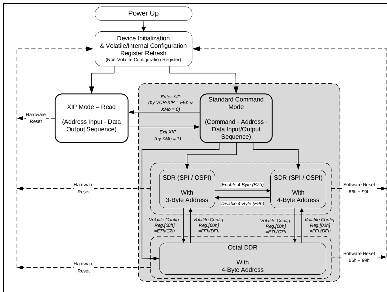
Figure 4-1. W35T12NW Serial Flash Memory Operation Diagram
