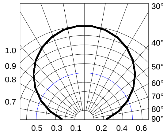
Fig.6-Radiation Diagram T a =25°C
