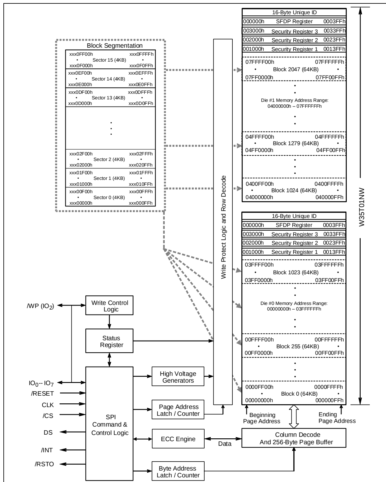
Figure 1. W35T01NW Serial Flash Memory Block Diagram
