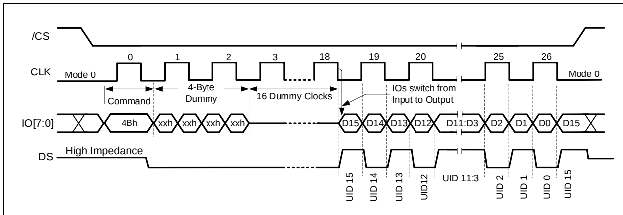
Figure 14-1b. Read Unique ID Command (ODOR Mode)
