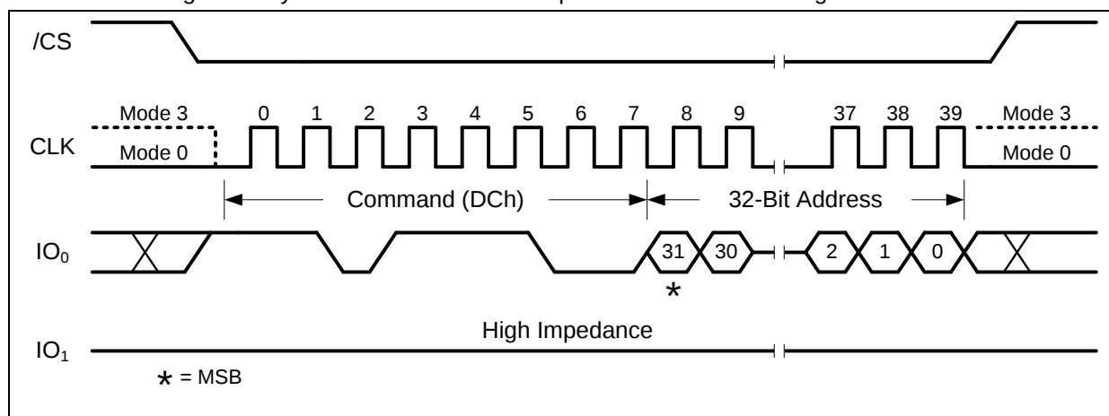
Figure 12-8. 64KB Block Erase using 4-Byte Address Command (SDR Mode)
