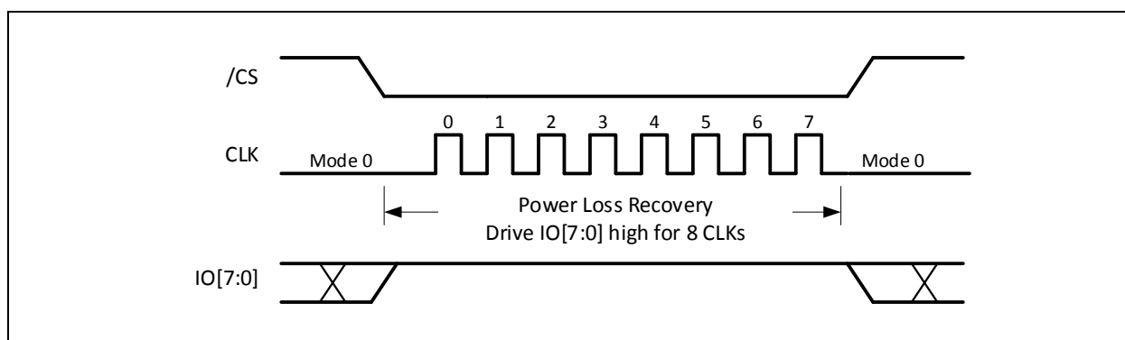
Figure 4-6. Power Loss Interface Recovery
