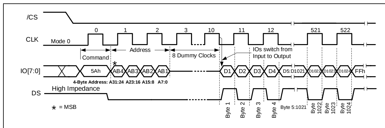
Figure 7-2b. Read SFD Register Command Sequence (ODDR Mode)
