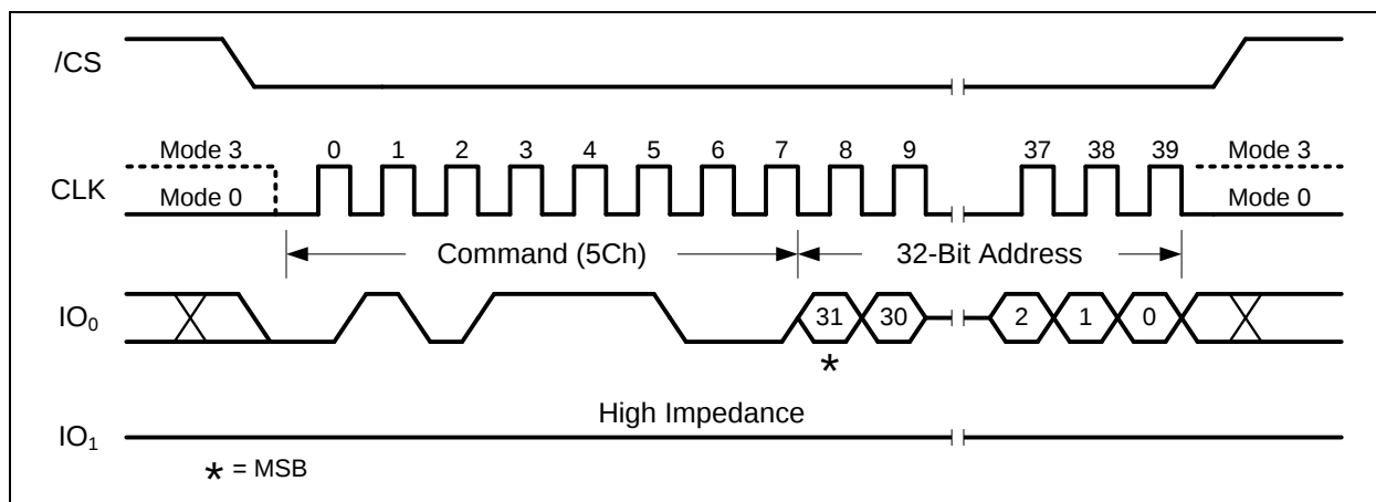
Figure 12-5. 32KB Block Erase using 4-Byte Address Command (SDR Mode)
