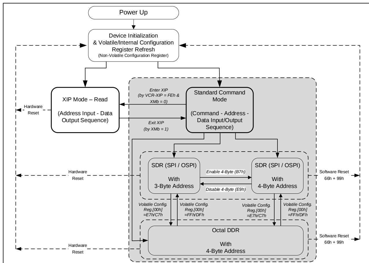
Figure 4-1. W35T01NW Serial Flash Memory Operation Diagram
