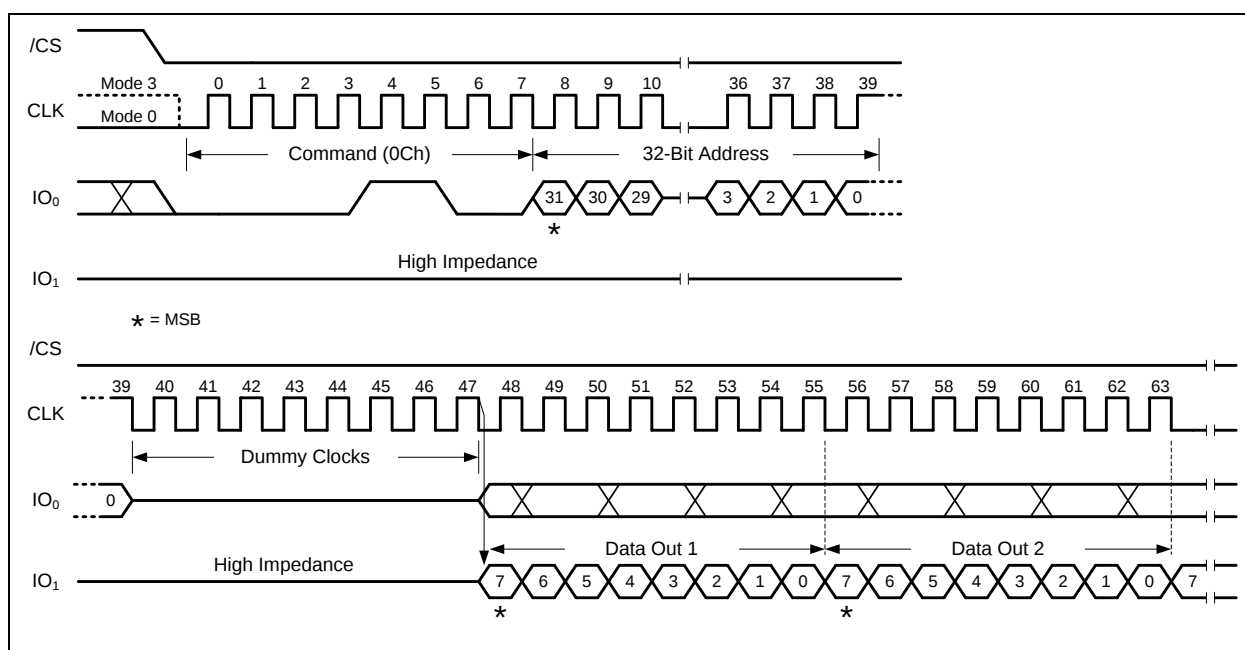
Figure 10-4. Fast Read using 4-Byte Address Command (1-1-1 SDR Mode)
