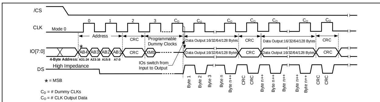
Figure 18-40. 0-8d-8d XIP Read Memory CRC-In-Transit Command Protocol (ODDR Mode)
