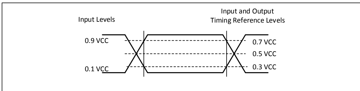
Figure 19-4. AC Measurement I/O Waveform
