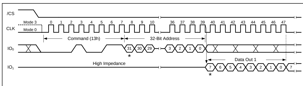
Figure 10-2. Read Data using 4-Byte Address Command (SDR Mode only)
