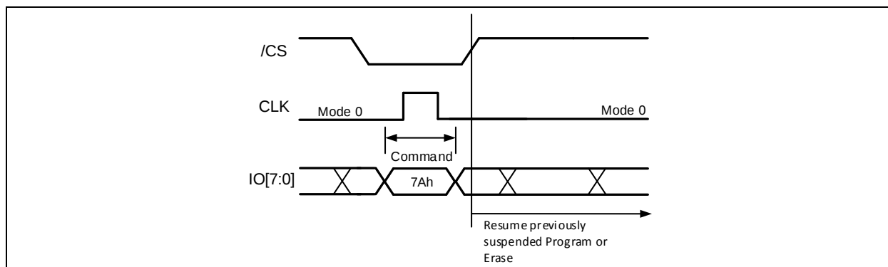
Figure 13-2b. Erase/Program Resume Command (ODDR Mode)
