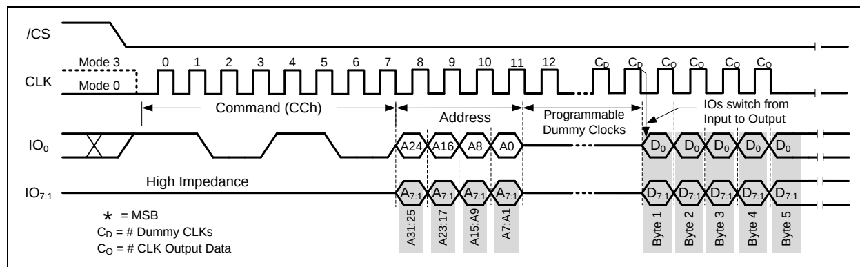
Figure 10-8. Fast Read Octal I/O Command using 4-Byte Address (1-8-8 SDR)
