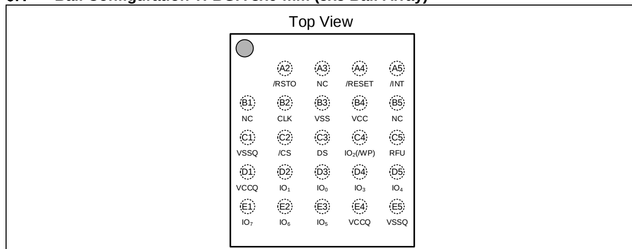
Figure 3-1. W35T01NW Ball Assignments, 24-ball (5x5 ball array) TFBGA 6x8-mm (Package Code TB)
