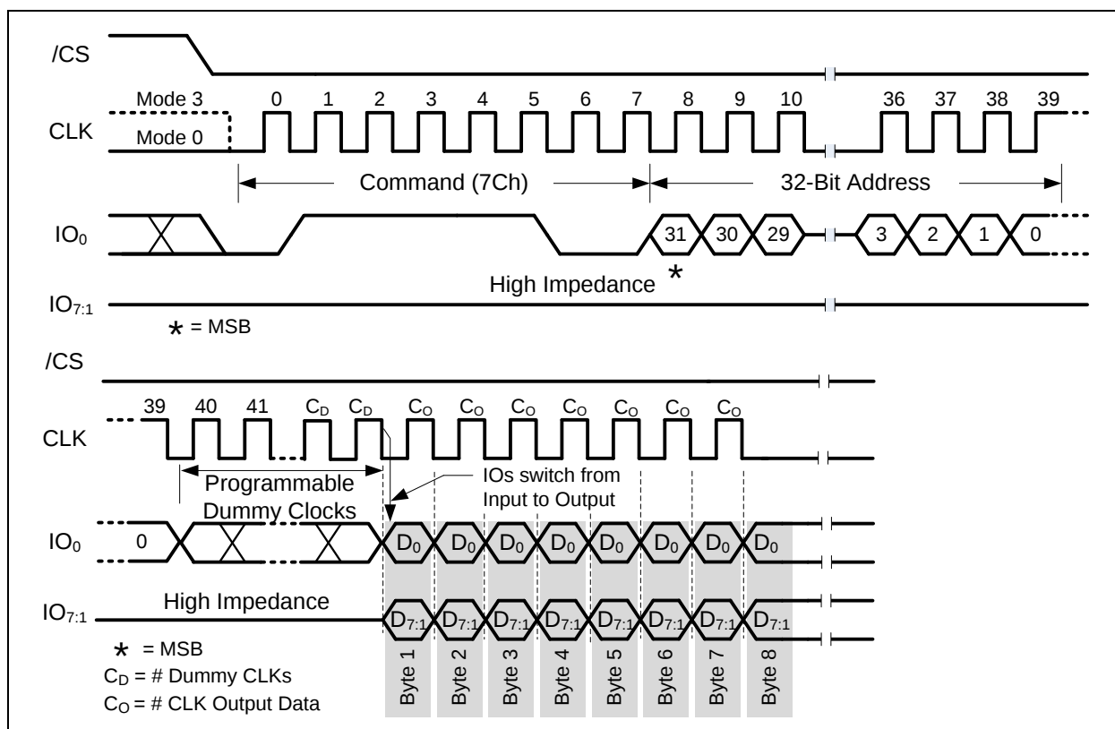
Figure 10-6. Fast Read Octal Output using 4-Byte Address Command (1-1-8 SDR Mode)
