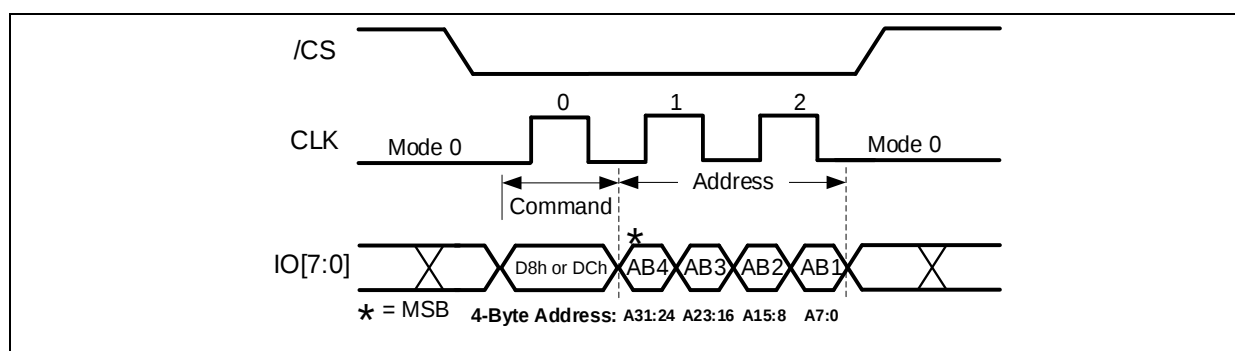
Figure 12-9. 64KB Block Erase Command (ODDR Mode)
