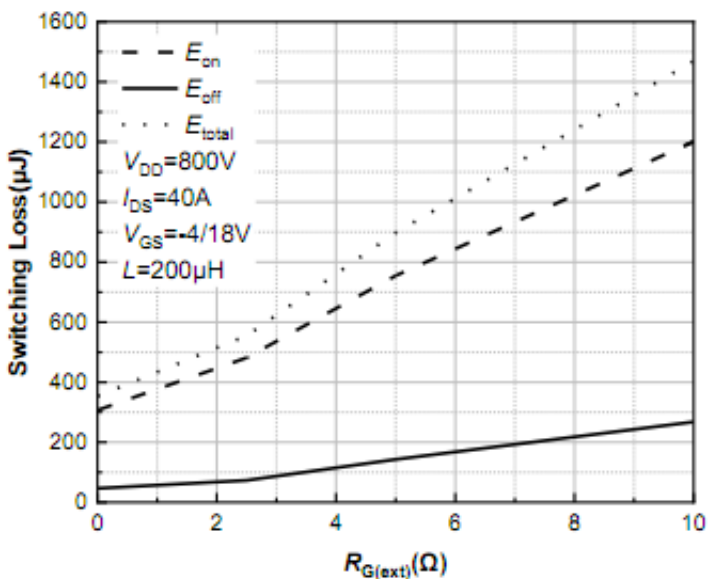
Figure 22. Clamped Inductive Switching Energy vs. R_{G(ext)}
