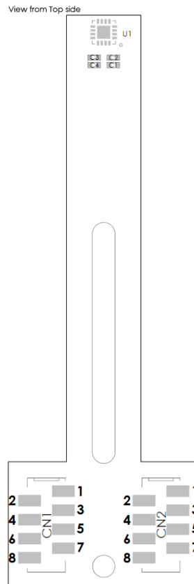
Figure 7: Type 1 Board Connector Pinout
