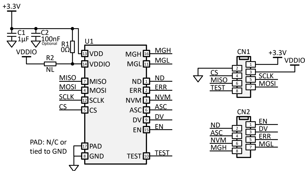
Figure 14: Type 3 Board Schematic
