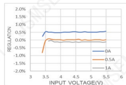
Line Regulation
