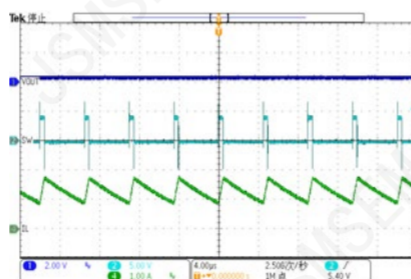
Output Short
