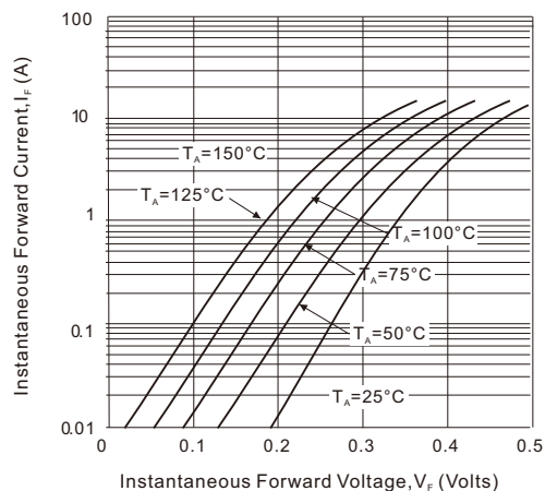
FIG.2-TYPICAL FORWARD CHARACTERISTICS
