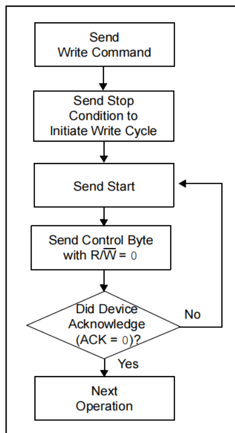
FIGURE8: ACKNOWLEDGE POLLING FLOW
