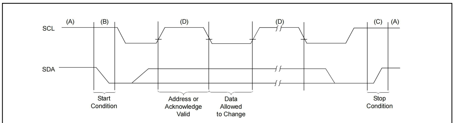
FIGURE 2: DATA TRANSFER SEQUENCE ON THE SERIAL BUS
