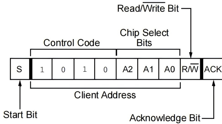
FIGURE 4: CONTROL BYTE FORMAT
