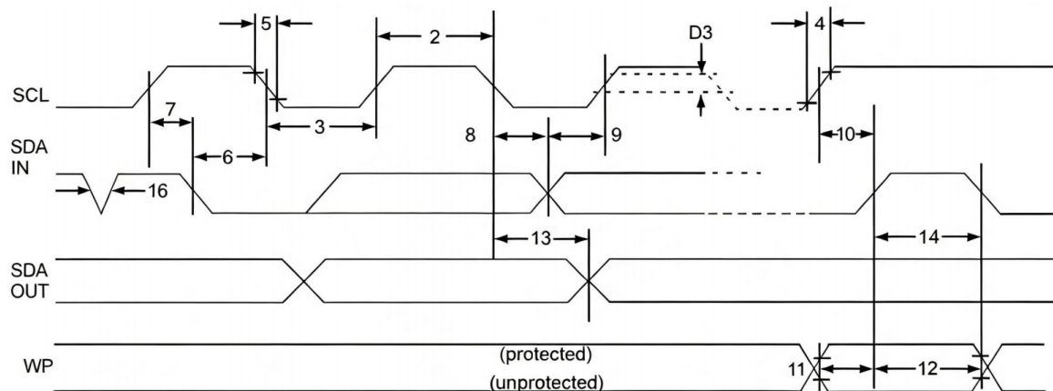
FIGURE 1: BUS TIMING DATA
