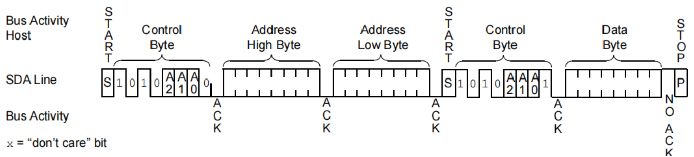
FIGURE10: RANDOM READ
