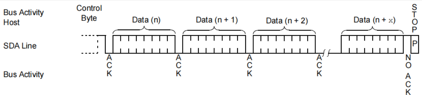
FIGURE 11: SEQUENTIAL READ
