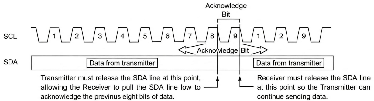
FIGURE 3: ACKNOWLEDGE TIMING
