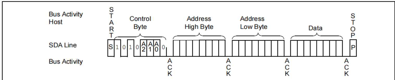
FIGURE 6: BYTE WRITE
