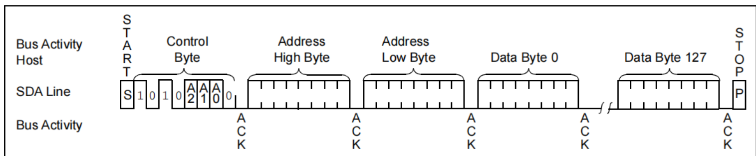
FIGURE 7: PAGE WRITE
