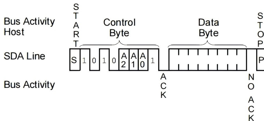
FIGURE9: CURRENT ADDRESS READ
