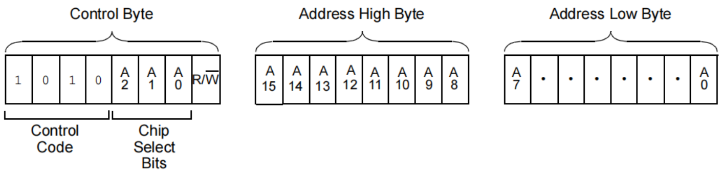
FIGURE 5: ADDRESS SEQUENCE BIT ASSIGNMENTS
