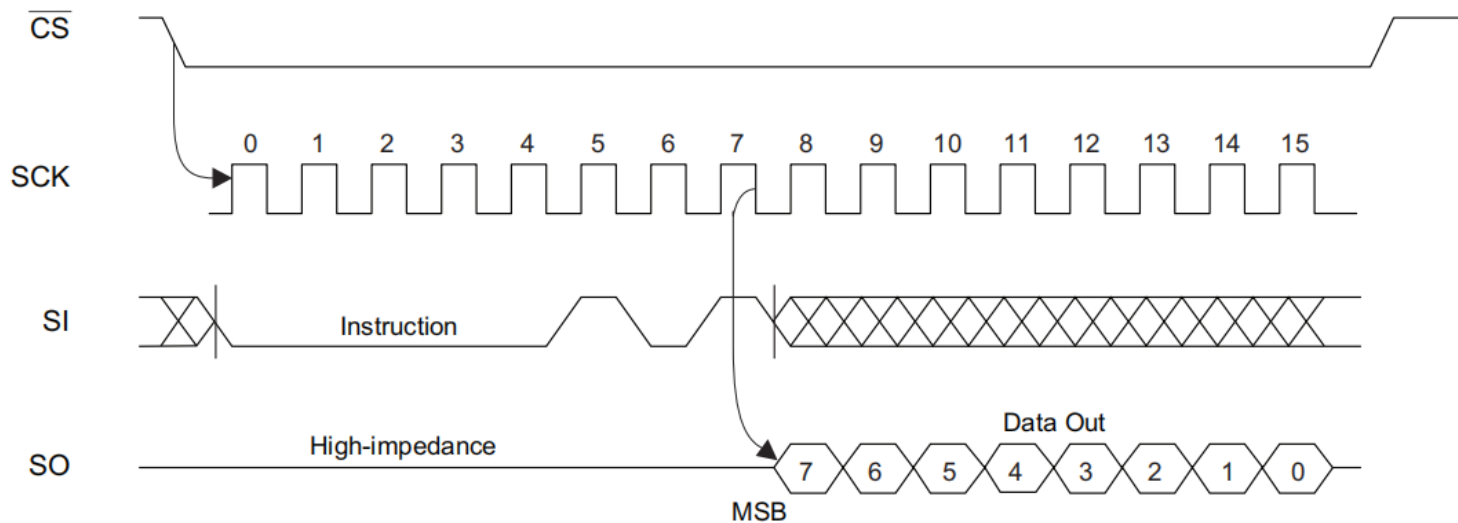
Figure 6. RDSR Timing
