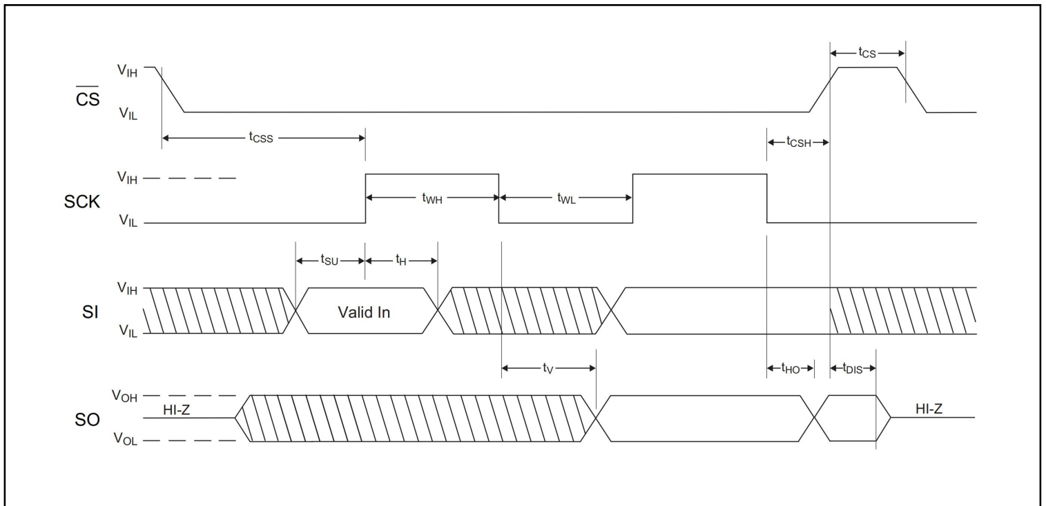
Figure 3. Synchronous Data Timing
