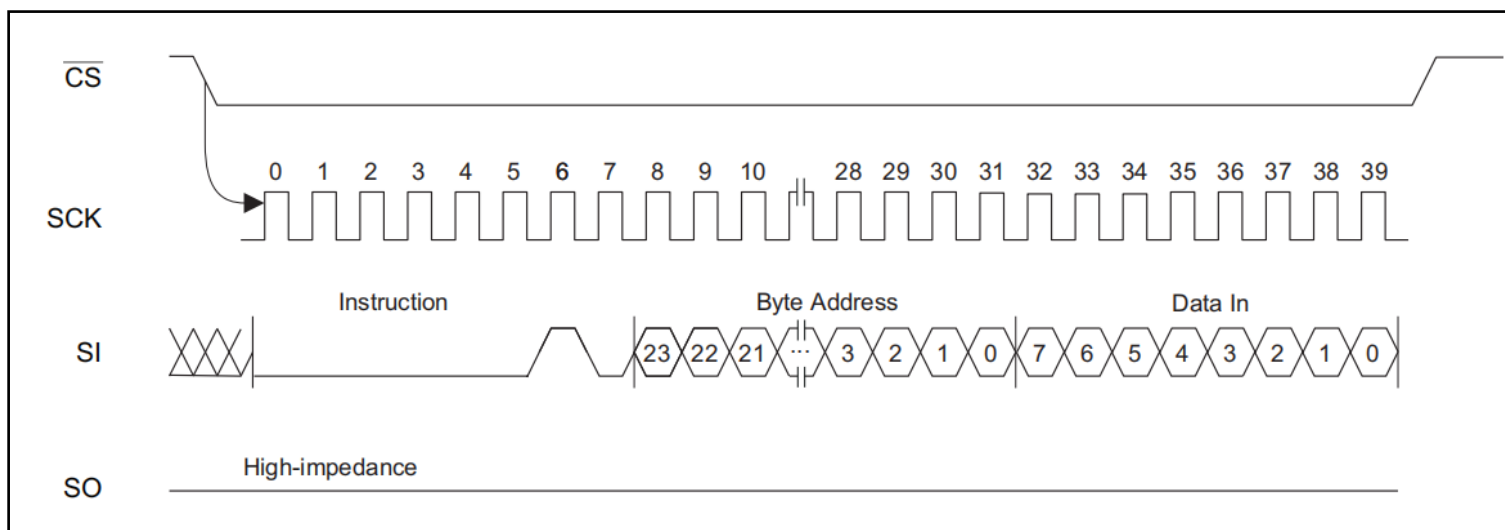
Figure 9. Write Timing
