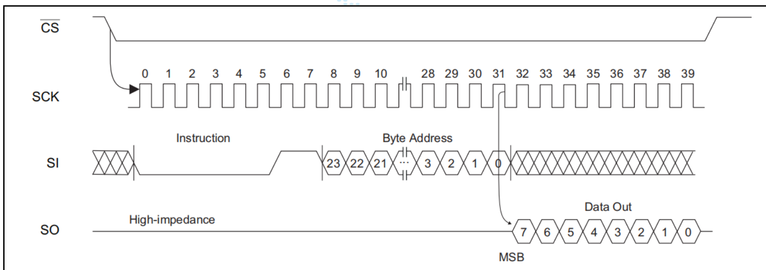
Figure 8. READ Timing
