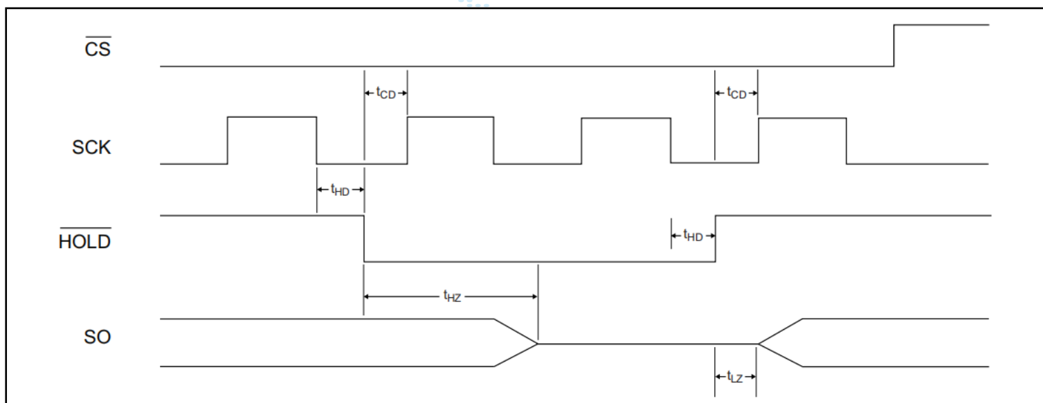
Figure 10. Hold Timing
