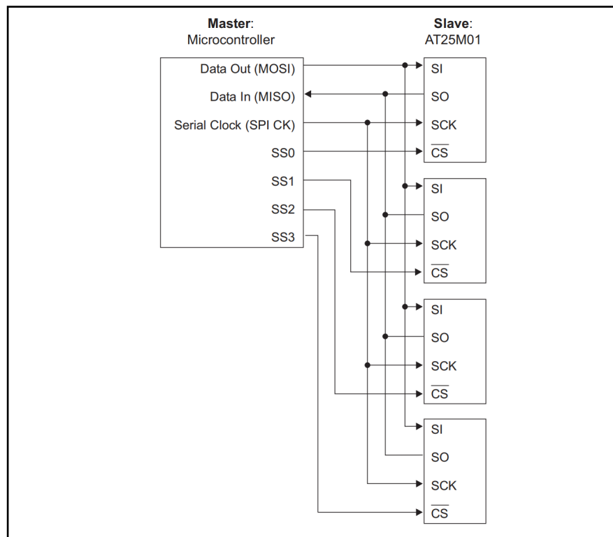
Figure 2. SPI Serial Interface
