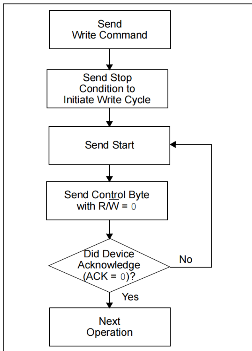
FIGURE 8: ACKNOWLEDGE POLLING FLOW
