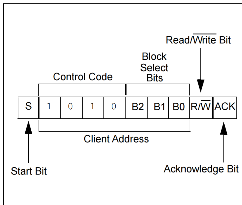
FIGURE 4: CONTROL BYTE ALLOCATION
