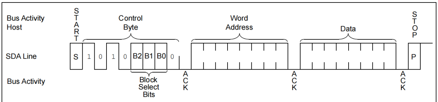
FIGURE 6: BYTE WRITE
