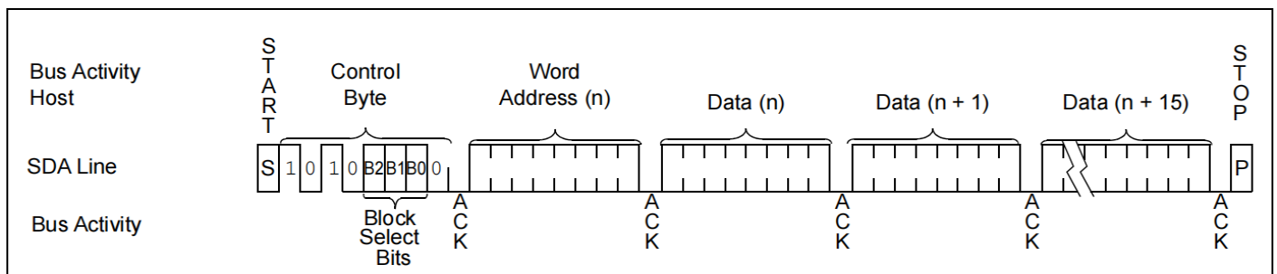
FIGURE 7: PAGE WRITE
