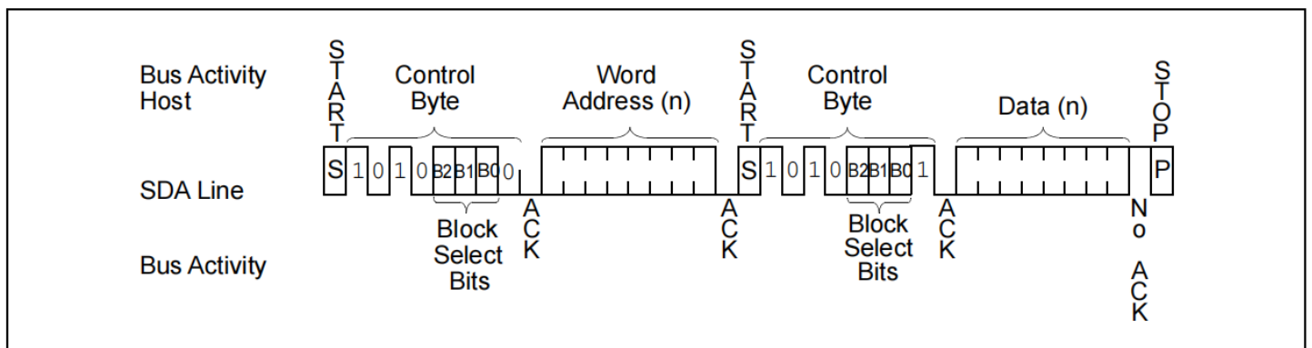
FIGURE 10: RANDOM READ
