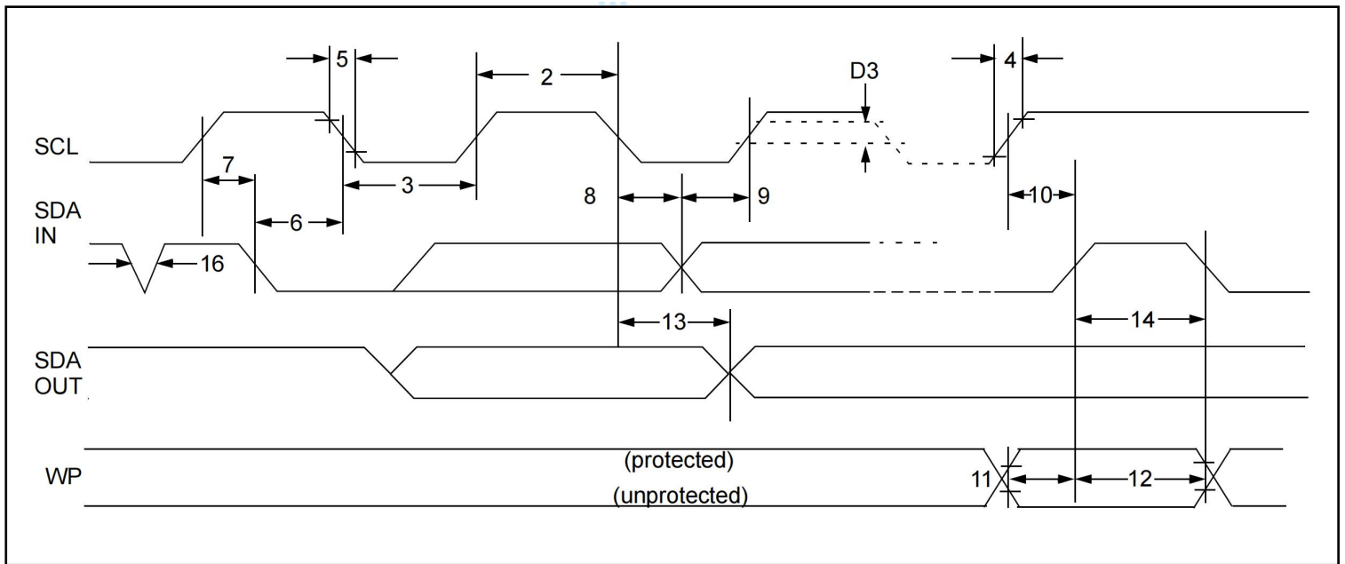
FIGURE 1: BUS TIMING DATA
