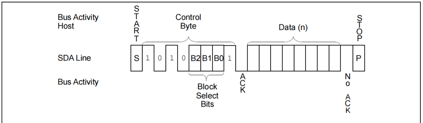
FIGURE 9: CURRENT ADDRESS READ
