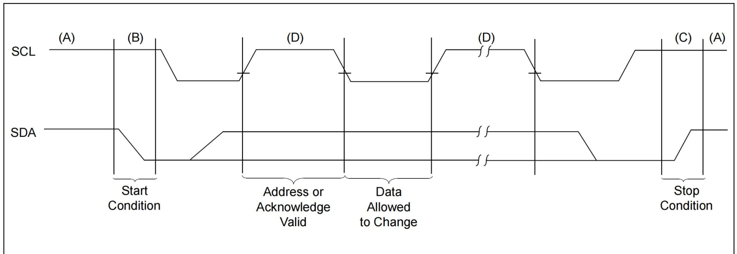
FIGURE 3: DATA TRANSFER SEQUENCE ON THE SERIAL BUS
