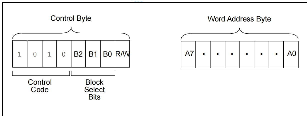
FIGURE 5: ADDRESS SEQUENCE BIT ASSIGNMENTS
