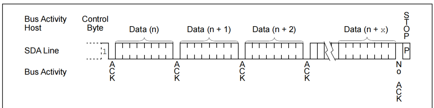
FIGURE 11: SEQUENTIAL READ
