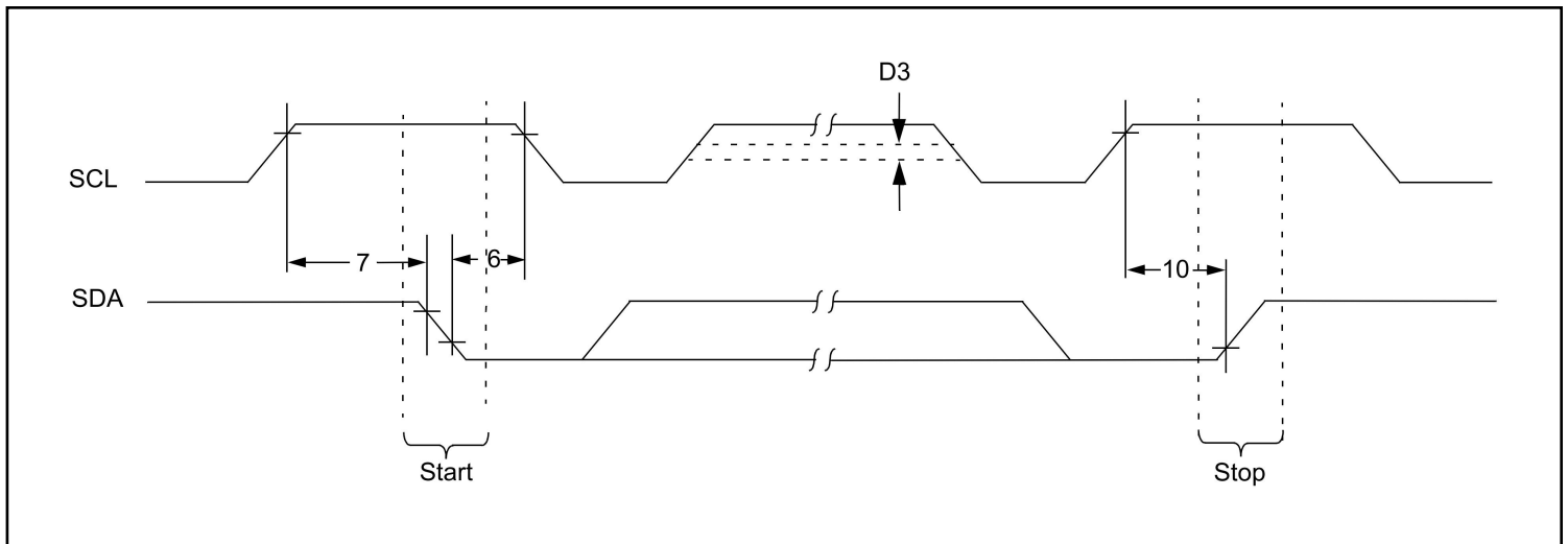
FIGURE 2: BUS TIMING START/STOP
