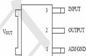
TO-252
