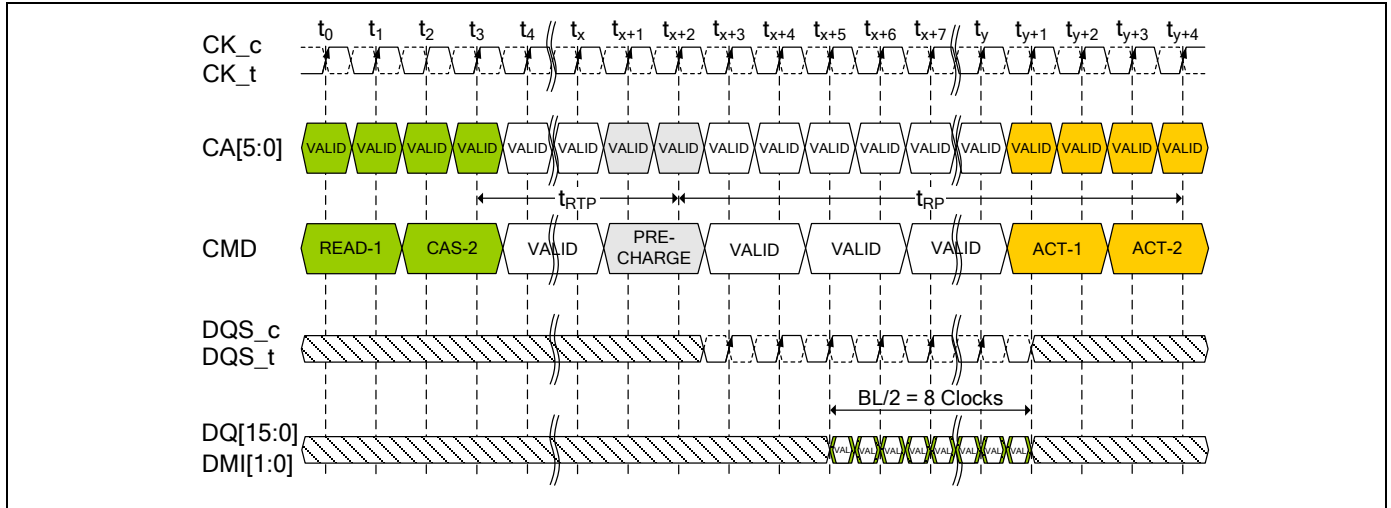
Figure 56 - Burst READ followed by PRECHARGE (Shown with BL16, 2tCK pre-ambles)
