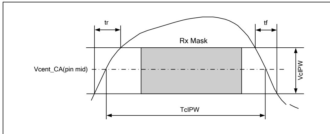
Figure 169 - CA TclPW and SRIN_clVW definition (for each input pulse)
