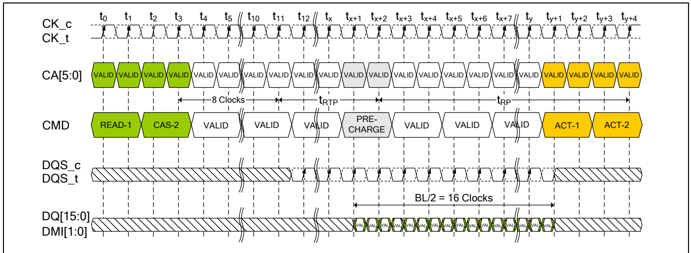
Figure 57 - Burst READ followed by PRECHARGE (Shown with BL32, 2tCK pre-ambles)
