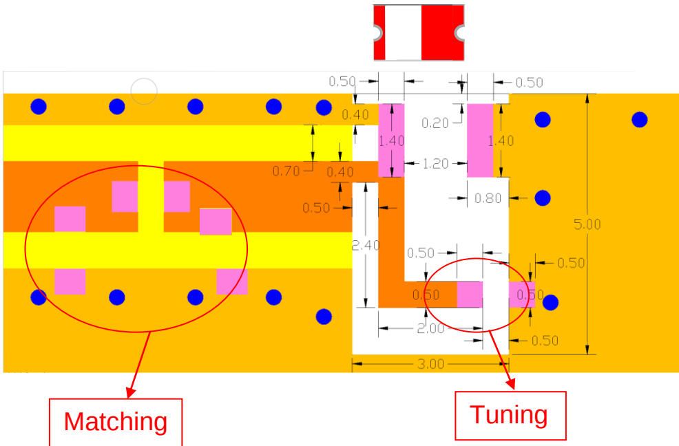
Layout Dimensions in Clearance area( Size=3.0*5.0mm)
