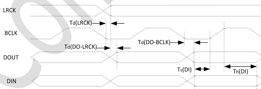
Figure 7-7. I2S Master Mode Timing
