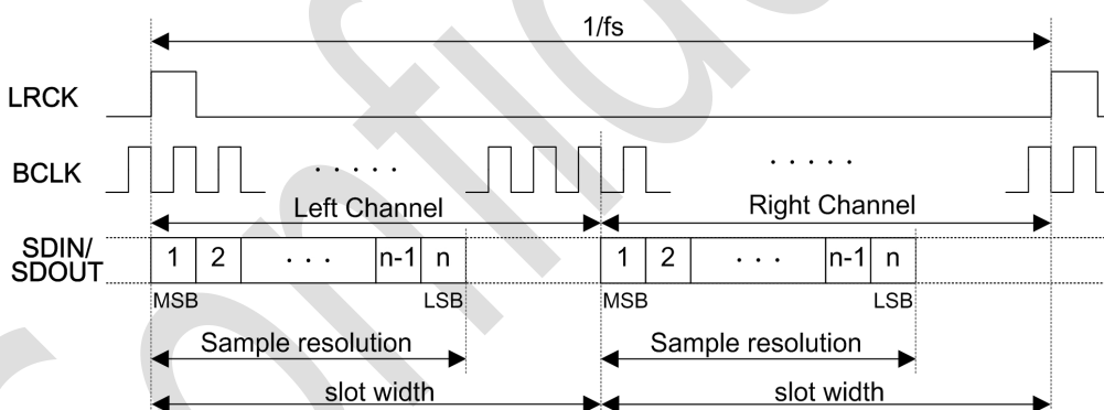
Figure 7-13. PCM mode B(Offset=0)
