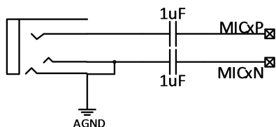
Figure 7-20. Suggested Single-Ended Line-in
