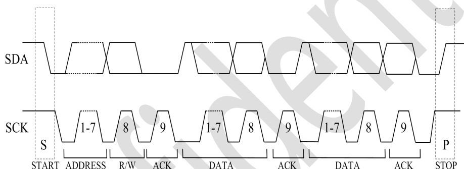
Figure 7-5. TWI Interface
