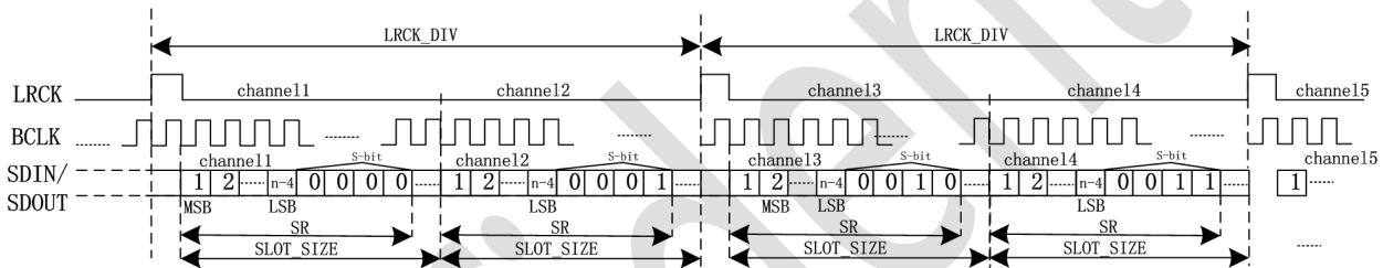
Figure 7-17. PCM Encoding mode
