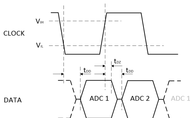
Figure 7-25. PDM Timing Diagram
