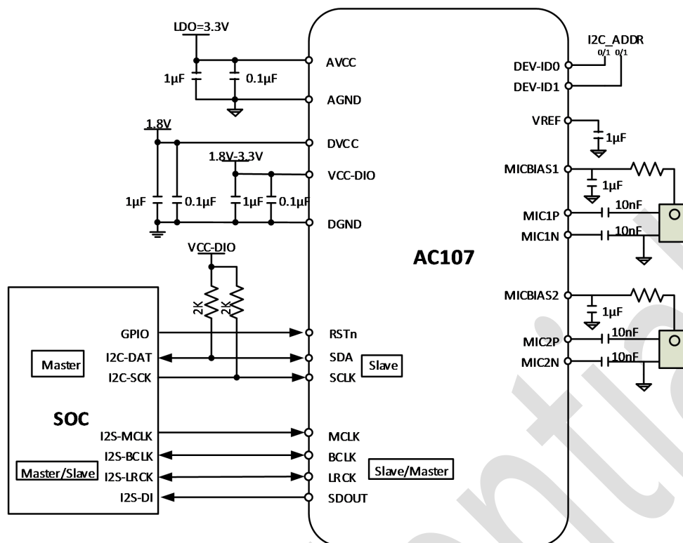
Figure 8-1. Typical Application Diagram
