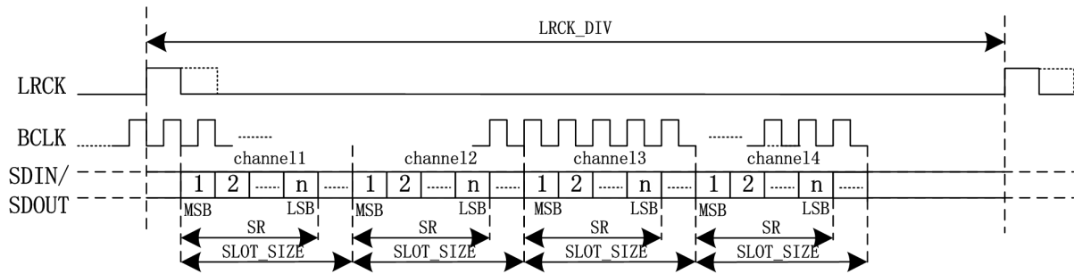
Figure 7-15. PCM TDM mode
