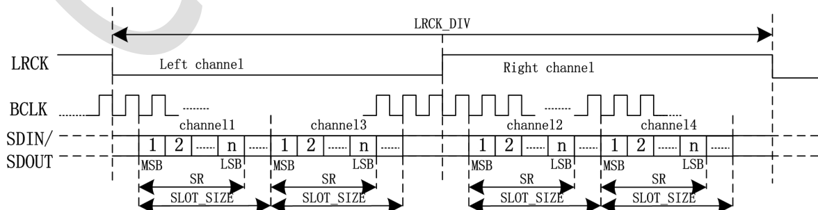
Figure 7-14. I2S TDM mode
