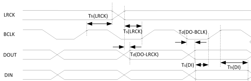
Figure 7-8. I2S Slave Mode Timing Table 7-5. I2S Timing in Slave Mode
