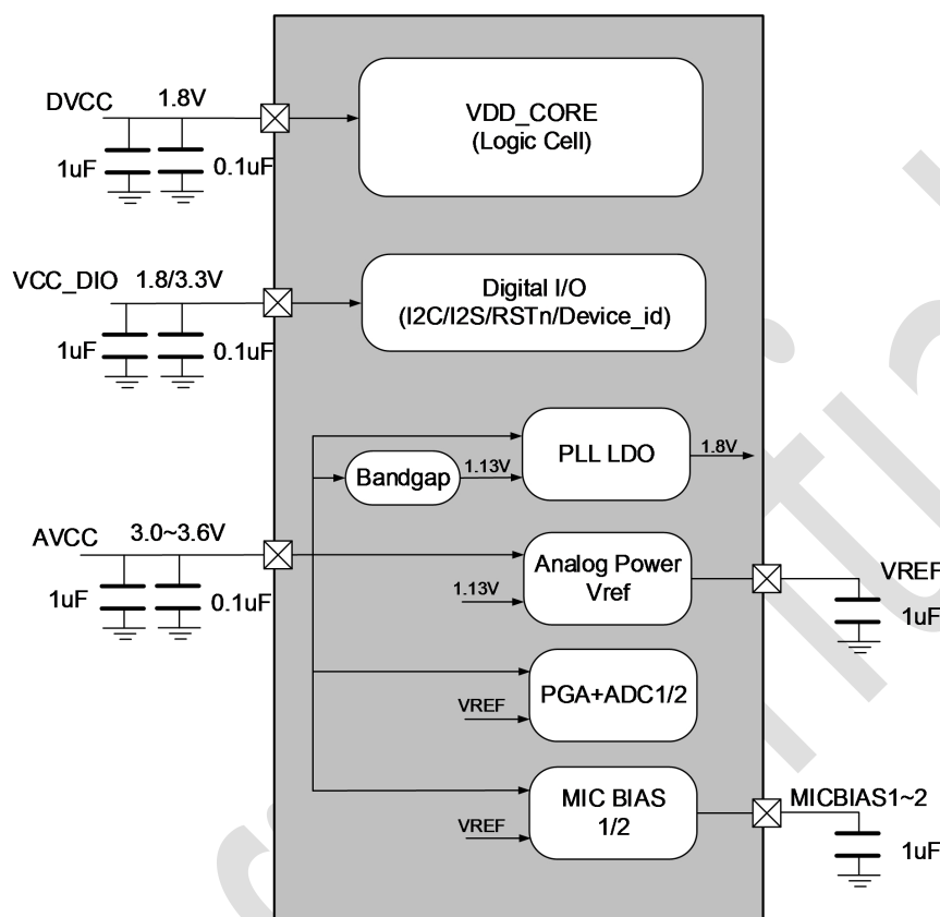
Figure 7-2. Power Management
