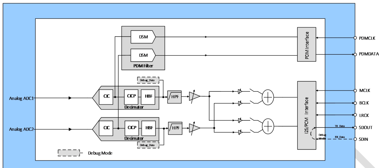
Figure 7-22. Digital Data Path
