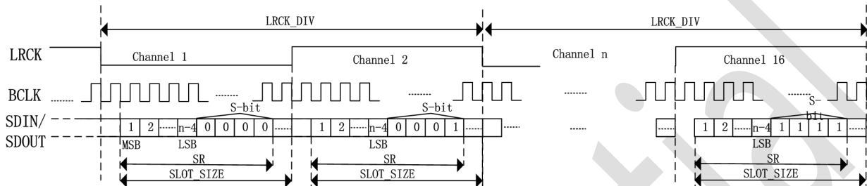
Figure 7-16. I2S Encoding mode
