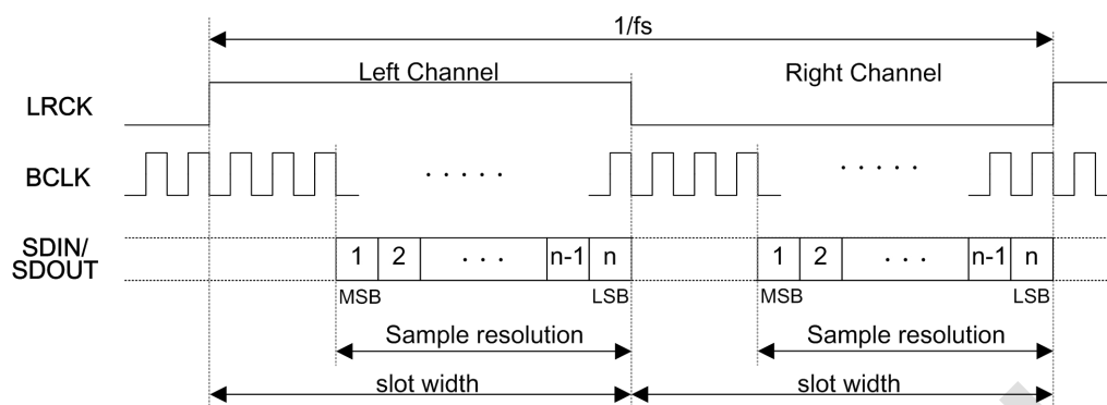
Figure 7-11. Right Justified mode
