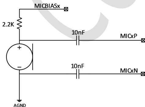
Figure 7-18. Suggested Single-Ended Mic Input
