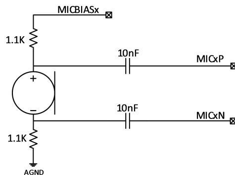
Figure 7-19. Suggested Differential Mic Input
