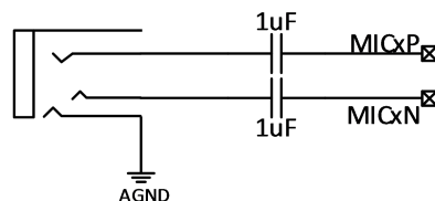
Figure 7-21. Suggested Differential Line-in
