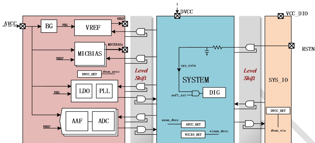
Figure 7-3. Reset Management
