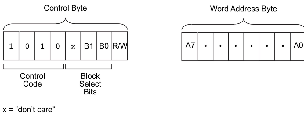
FIGURE 5: ADDRESS SEQUENCE BIT ASSIGNMENTS
