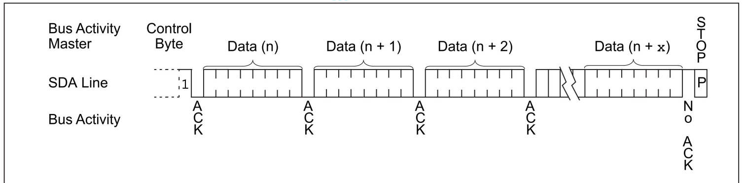
FIGURE 11: SEQUENTIAL READ
