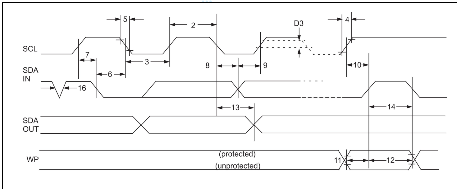
FIGURE 1: BUS TIMING DATA
