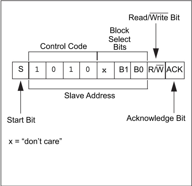
FIGURE 4: CONTROL BYTE ALLOCATION
