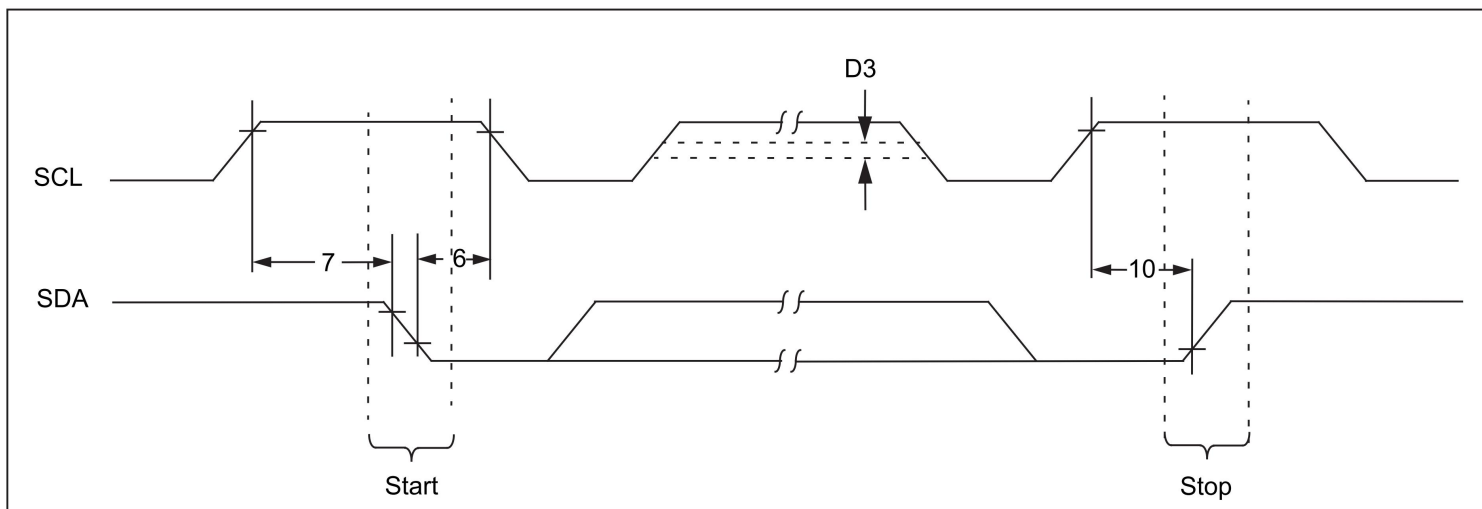
FIGURE 2: BUS TIMING START/STOP
