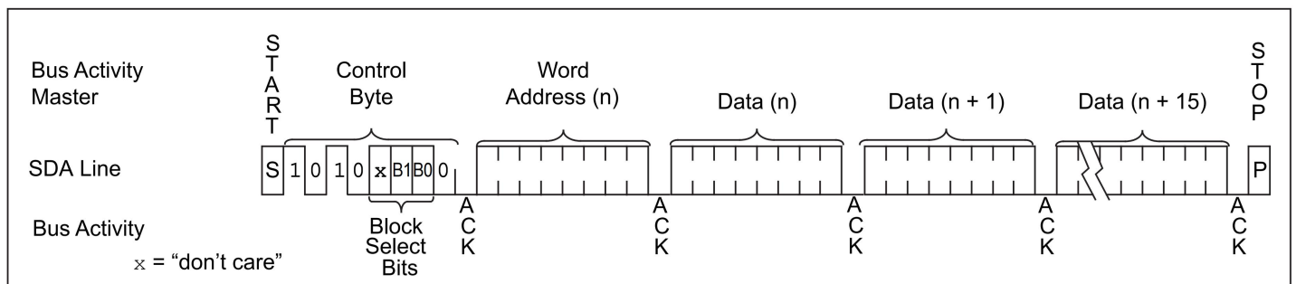
FIGURE 7: PAGE WRITE
