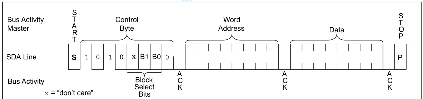
FIGURE 6: BYTE WRITE
