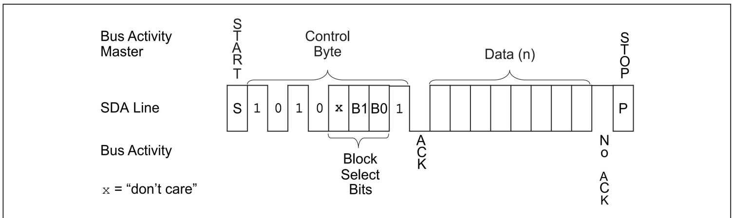
FIGURE 9: CURRENT ADDRESS READ
