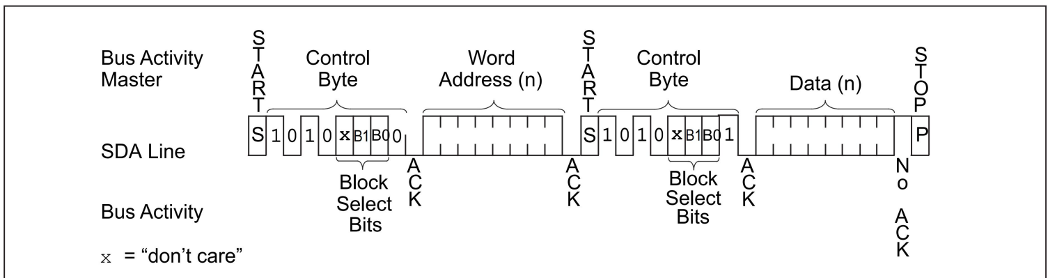
FIGURE 10: RANDOM READ
