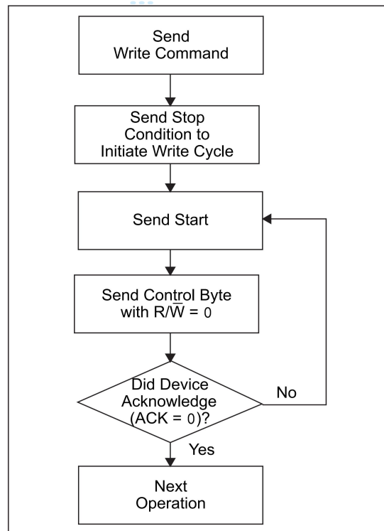
FIGURE 8.ACKNOWLEDGE POLLING FLOW
