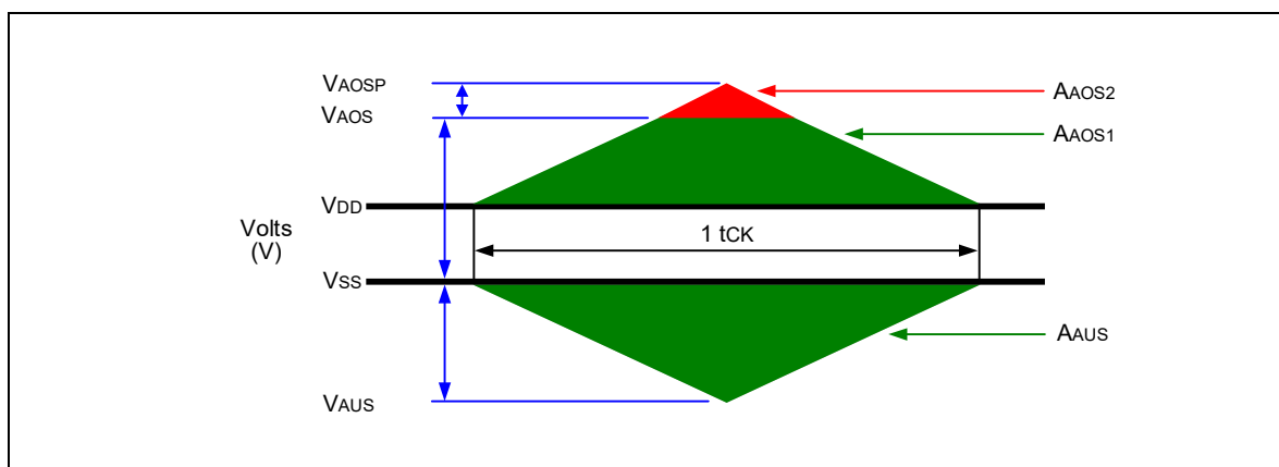
Figure 184 – Address, Command and Control Overshoot and Undershoot Definition
