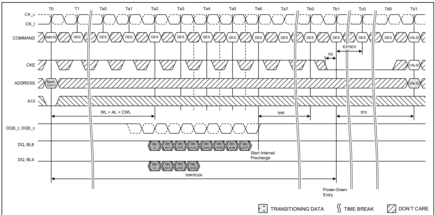
Figure 147 – Power-Down Entry after Write
