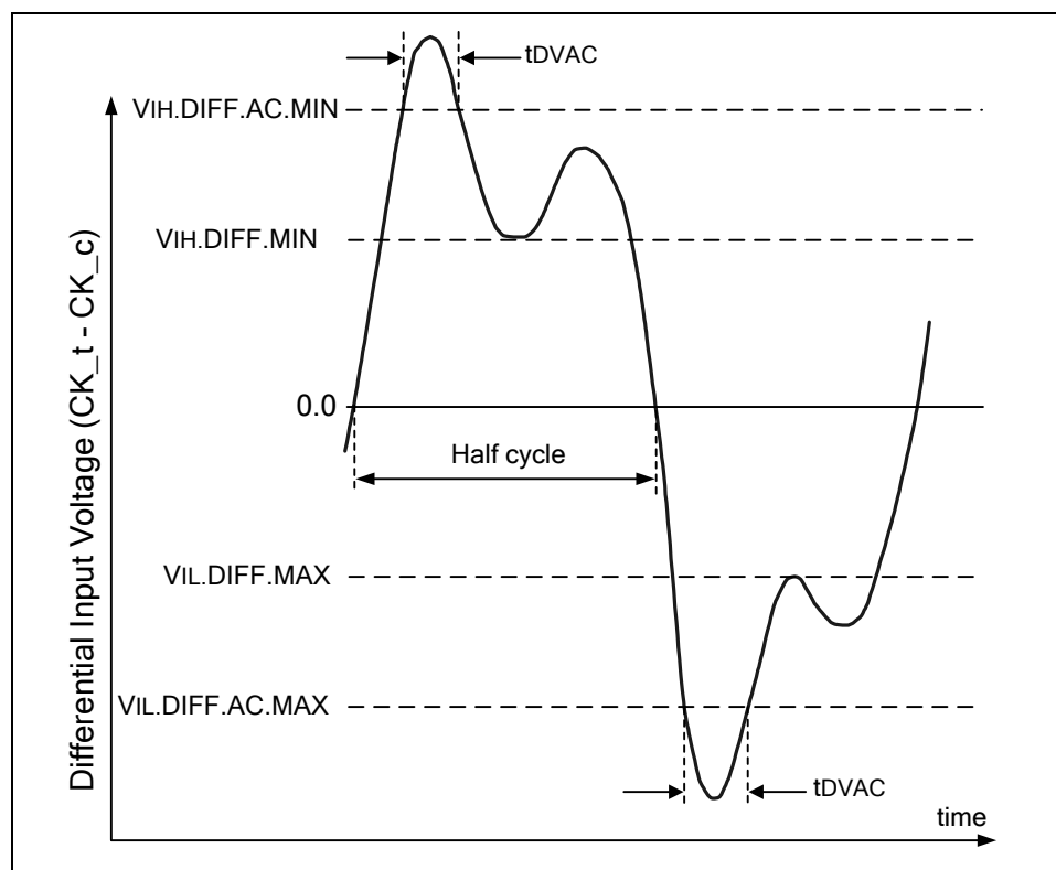
Figure 182 – Definition of differential ac-swing and “time above ac-level” tdVAC
