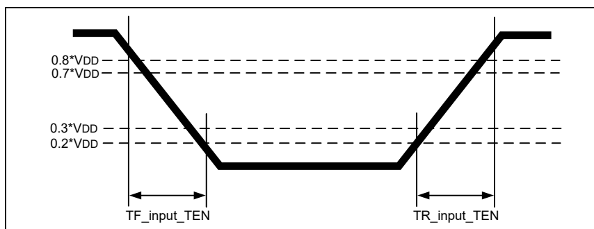
Figure 160 – TEN Input Slew Rate Definition
