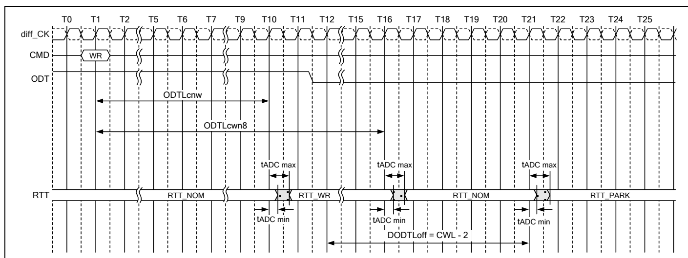
Figure 173 – Dynamic ODT overlapped with RTT_{NOM} (CL=14, CWL=11, BL=8, AL=0, CRC Disabled)
