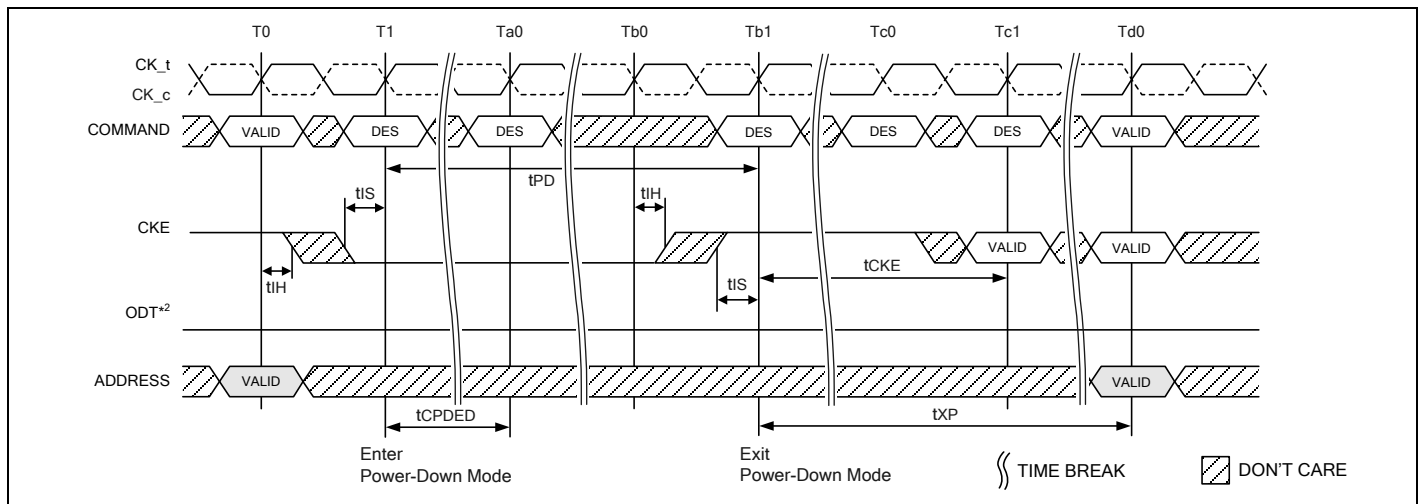
Figure 143 – Active Power-Down Entry and Exit Timing Diagram MR5 bit A5 = 0
