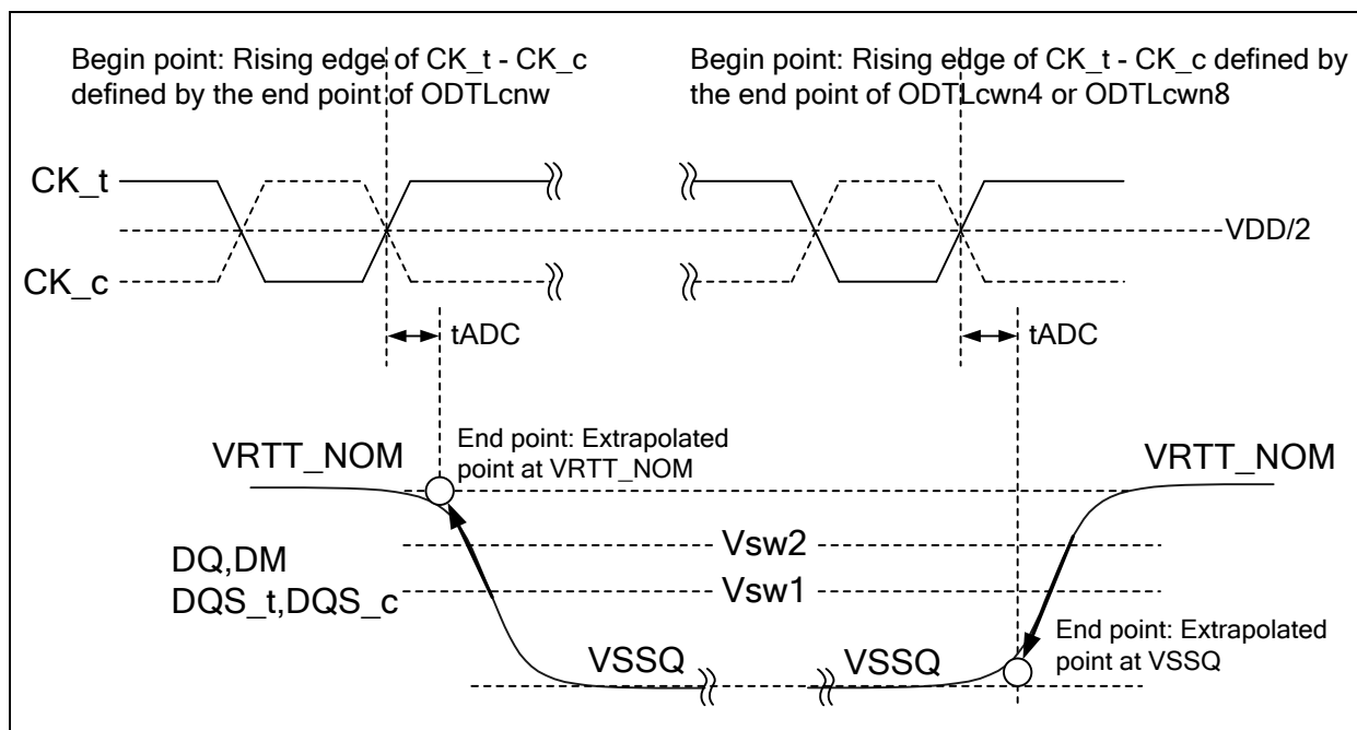
Figure 179 – Definition of t_{ADC} at Dynamic ODT Control
