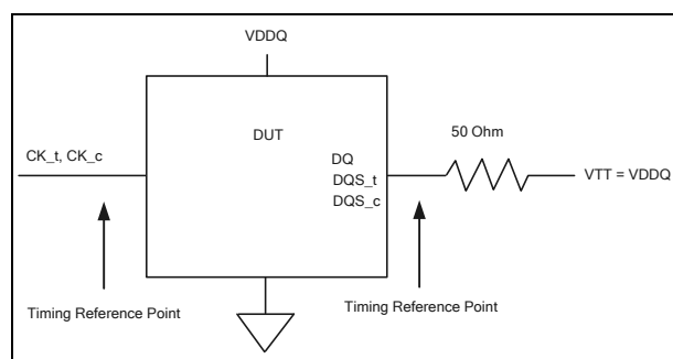
Figure 202 – Reference Load for AC Timing and Output Slew Rate
