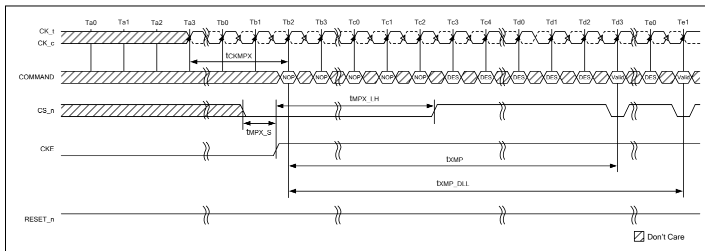
Figure 158 – Maximum Power Saving Mode Exit Sequence
