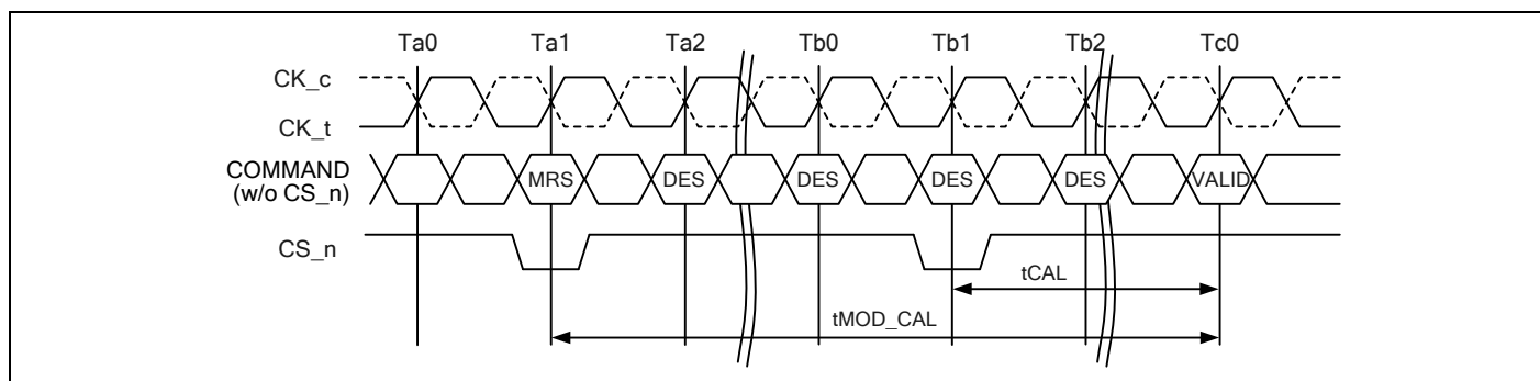
Figure 35 – CAL Enable timing - tMOD_CAL
