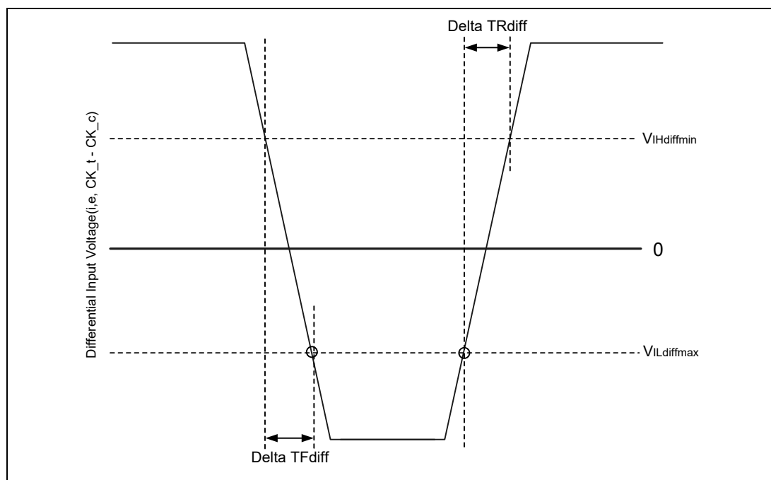
Figure 187 – Differential Input Slew Rate Definition for CK t , CK c
