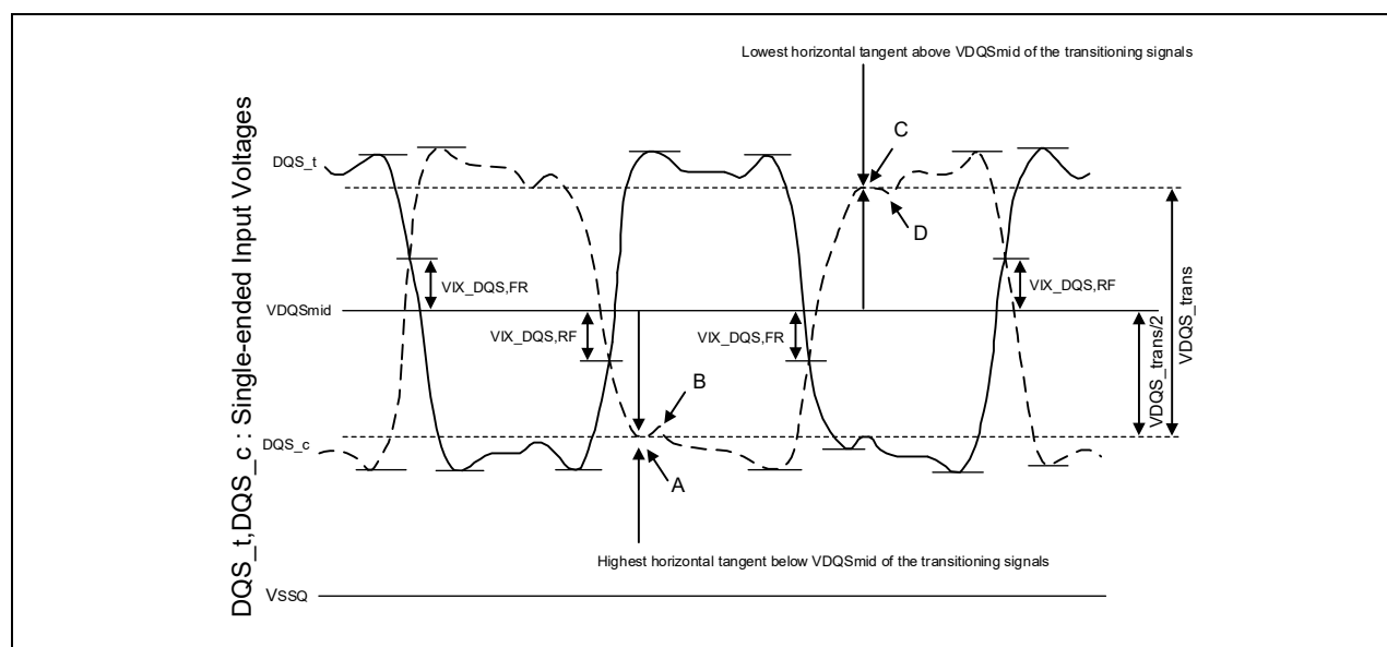
Figure 193 – Vix Definition (DQS)
