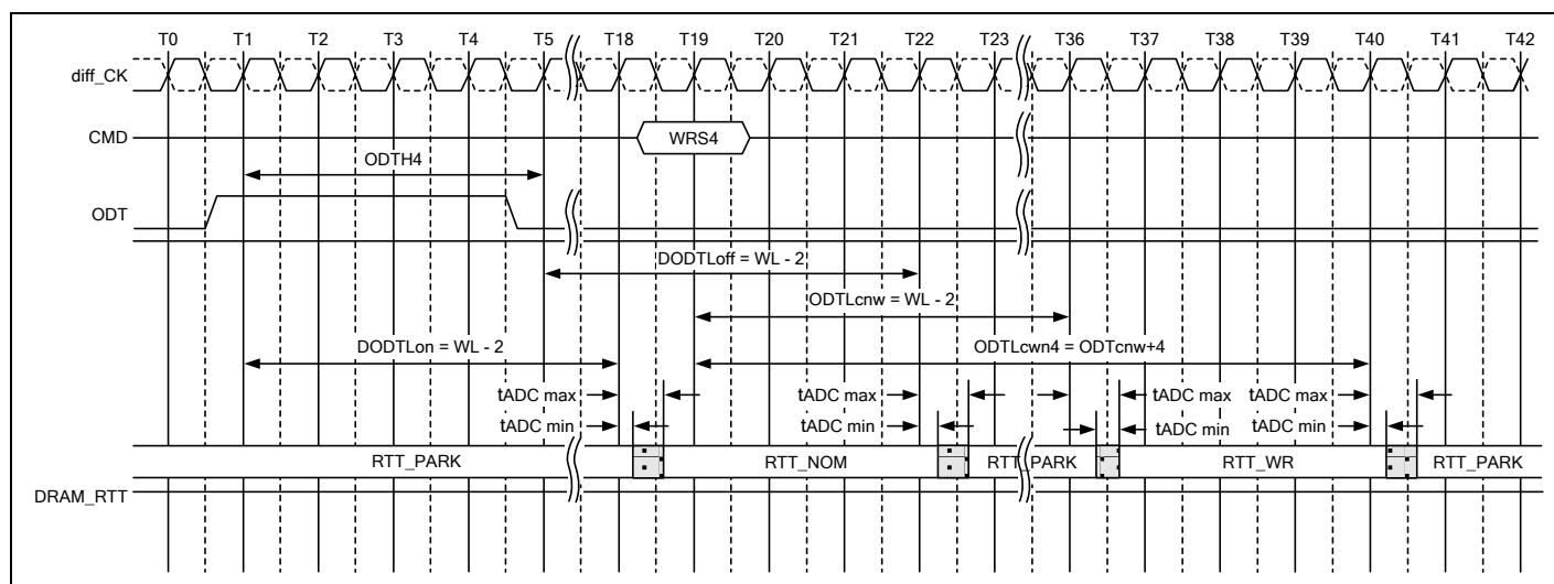
Figure 169 – Synchronous ODT example with BL=4, CWL=9, AL=10, PL=0; DODTLon/off=WL-2=17, ODTcnw=WL-2=17
