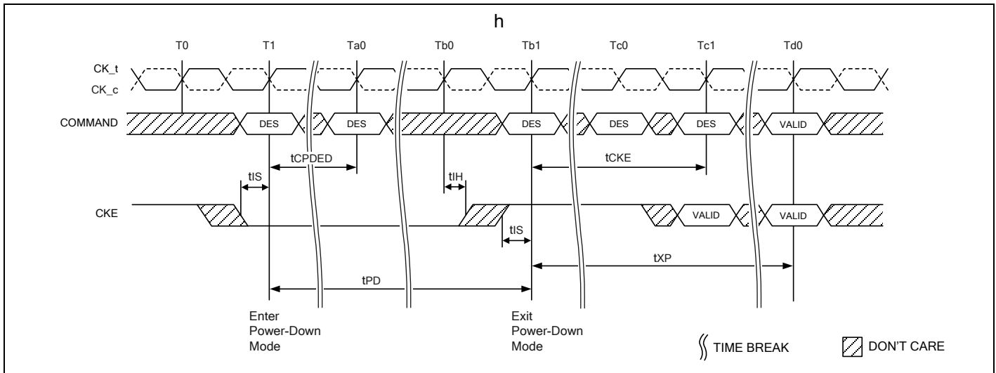
Figure 148 – Precharge Power-Down Entry and Exit
