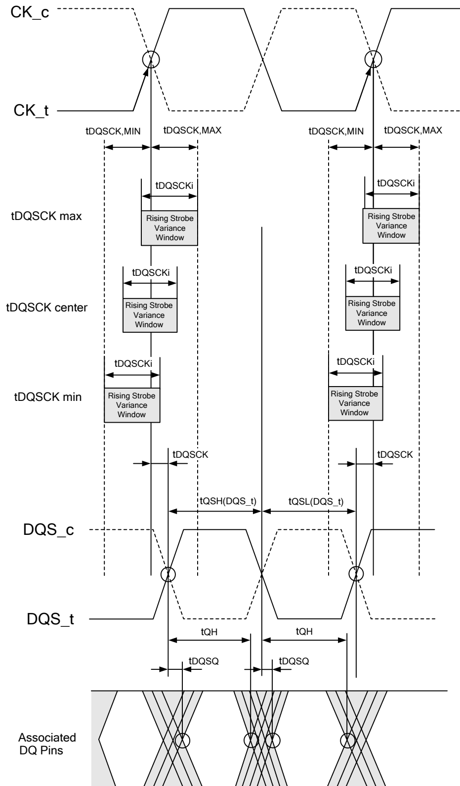
Figure 64 – READ Timing Definition
