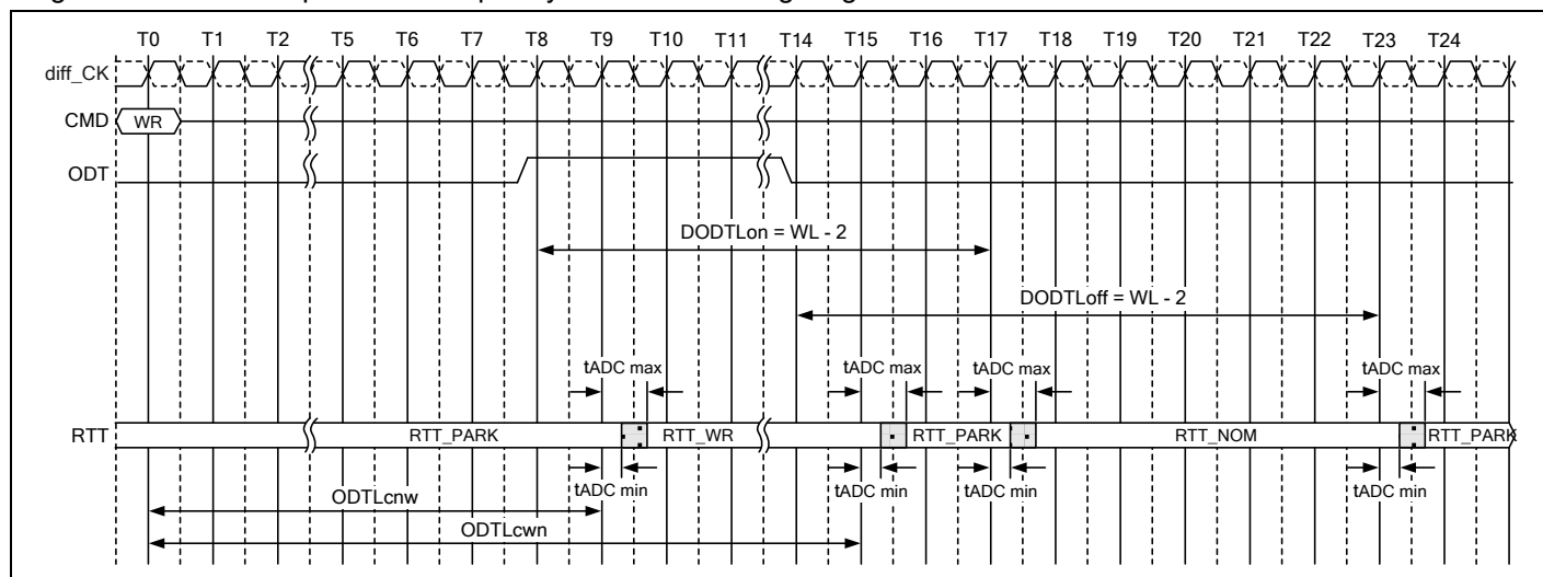
Figure 172 – ODT timing (Dynamic ODT, 1tCK preamble, CL=14, CWL=11, BL=8, AL=0, CRC Disabled)
