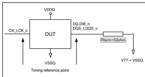
Figure 177 – ODT Timing Reference Load
