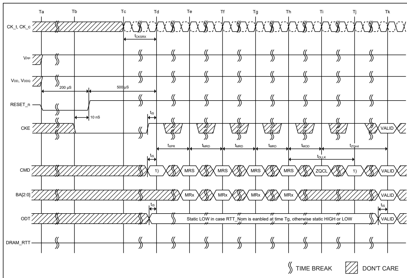
Figure 1 – RESET_n and Initialization Sequence at Power-on Ramping
