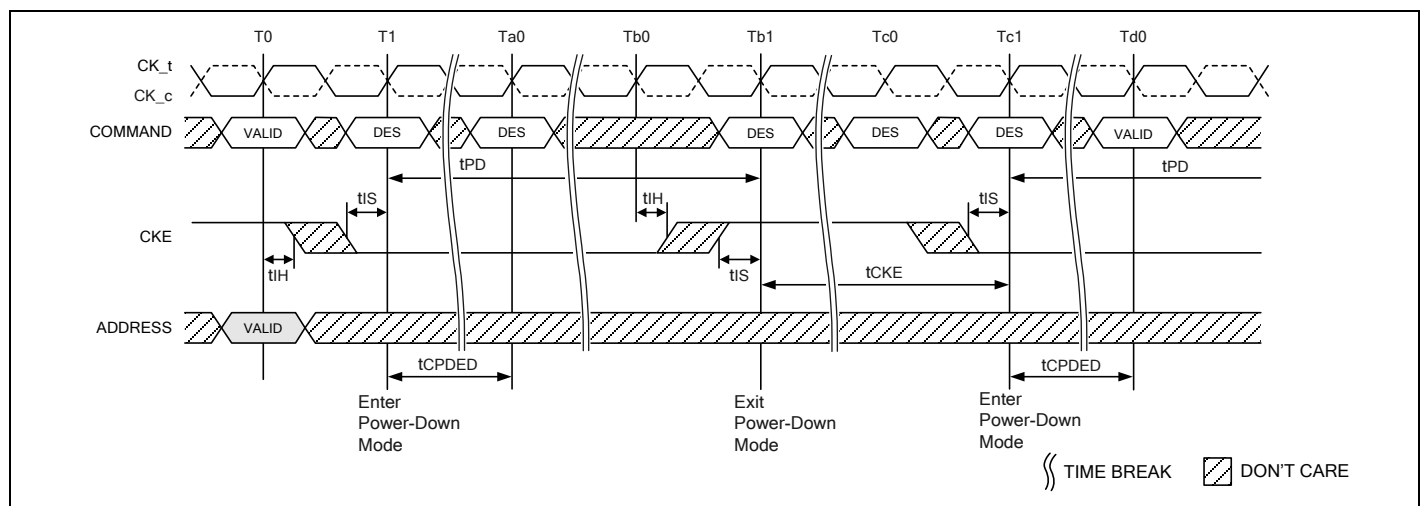
Figure 153 – Power-Down Entry/Exit Clarification
