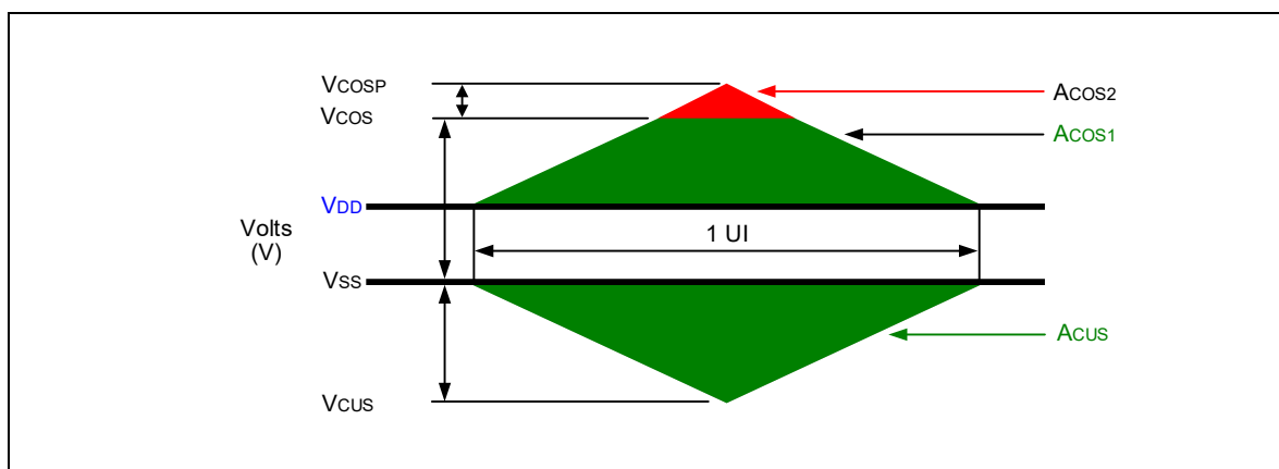
Figure 185 – Clock Overshoot and Undershoot Definition
