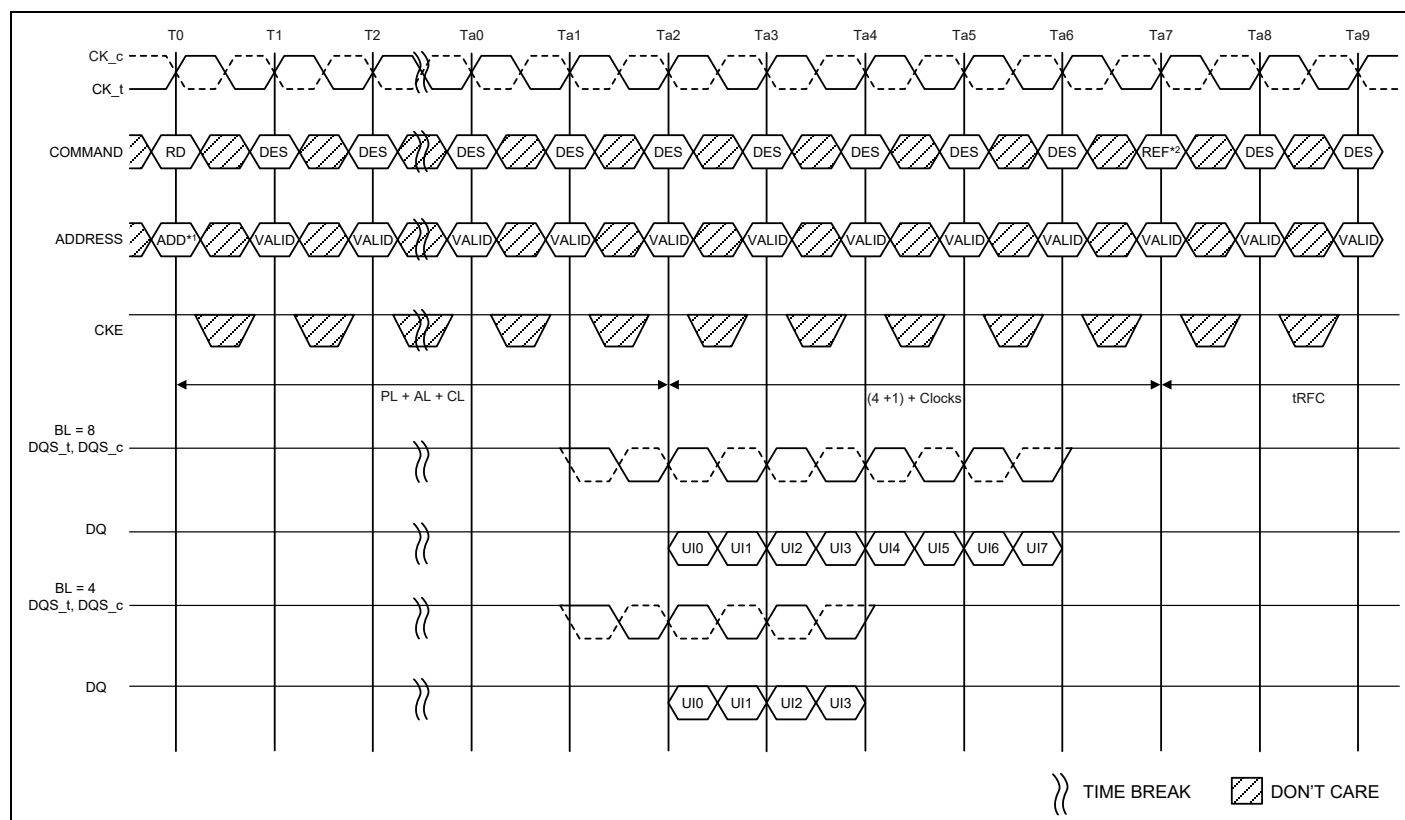
Figure 18 – Refresh Command Timing
