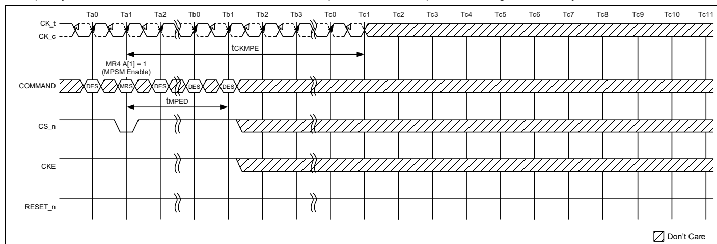
Figure 155 – Maximum Power Saving mode Entry
