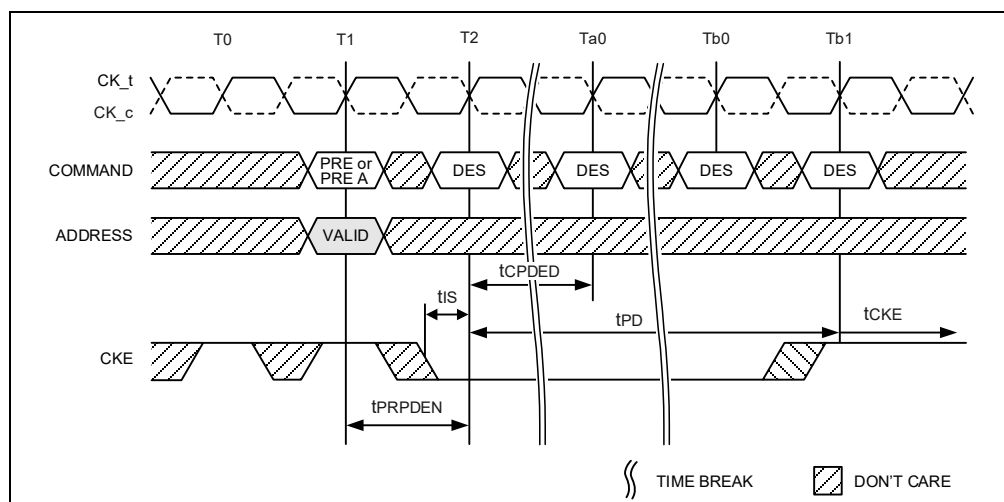
Figure 151 – Precharge/Precharge all Command to Power-Down Entry
