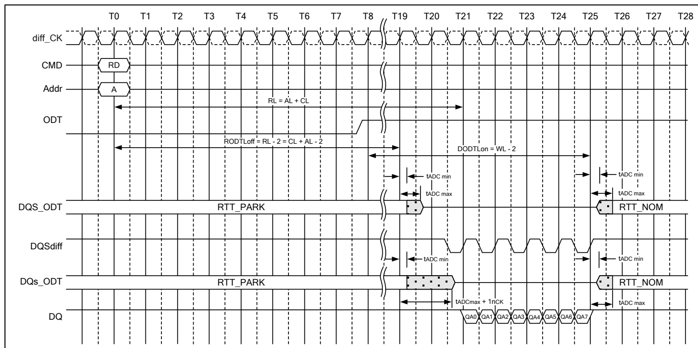
Figure 170 – Example: CL=11, PL=0; AL=CL-1=10; RL=AL+PL+CL=21; CWL=9; DODTLon=AL+CWL-2=17; RODTLoft=CL+AL-2=19; 1tCK preamble
