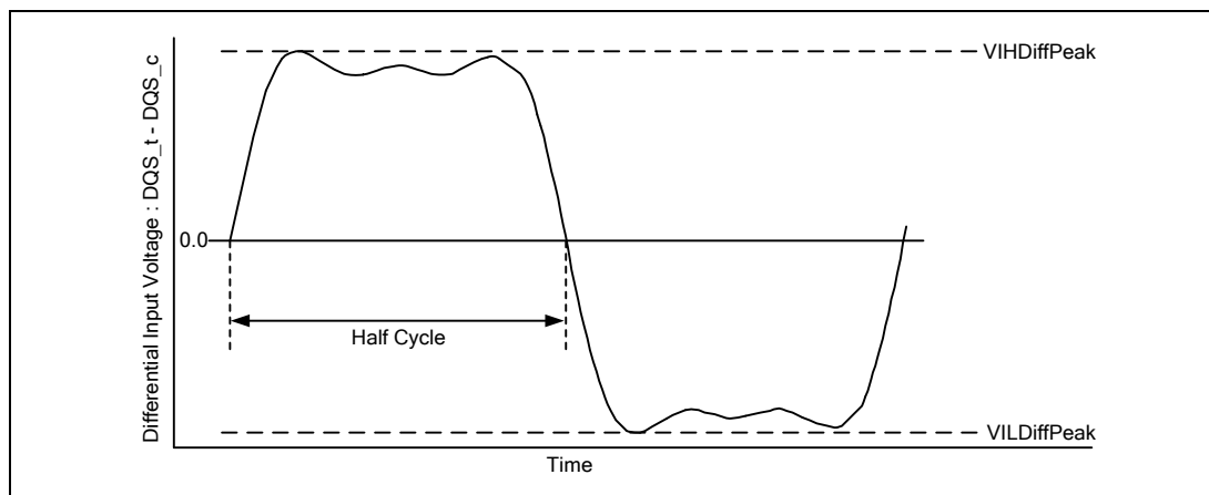
Figure 191 – Definition of differential DQS Signal AC-swing Level
