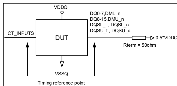
Figure 199 – Connectivity Test Mode Timing Reference Load
