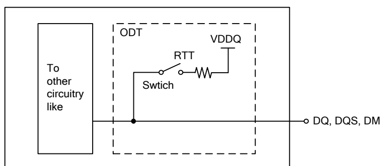
Figure 166 – Functional Representation of ODT
