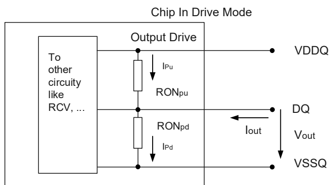
Figure 195 – Output driver
