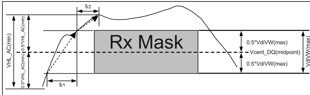
Figure 206 – Slew Rate Conditions for Rising Transition
