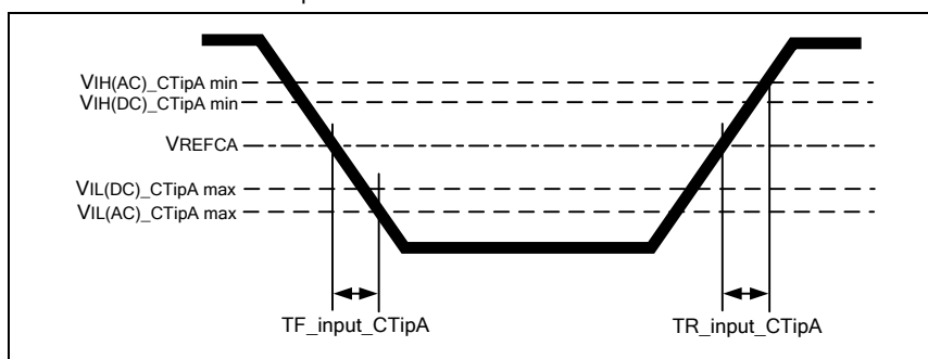
Figure 161 – CS_n and Input A Slew Rate Definition
