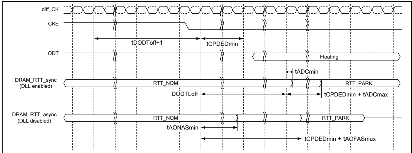
Figure 175 – ODT timing for power down entry with ODT buffer disable mode
