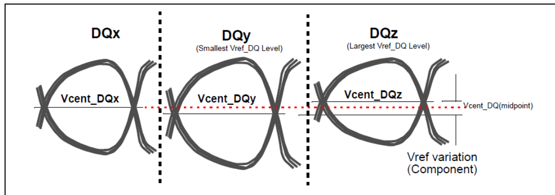
Figure 204 – Vcent_DQ Variation to Vcent_DQ(midpoint)
