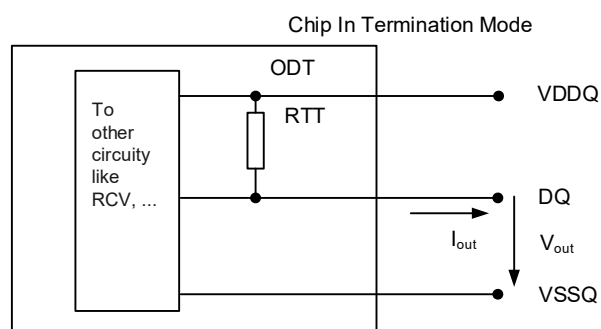
Figure 167 – On Die Termination
