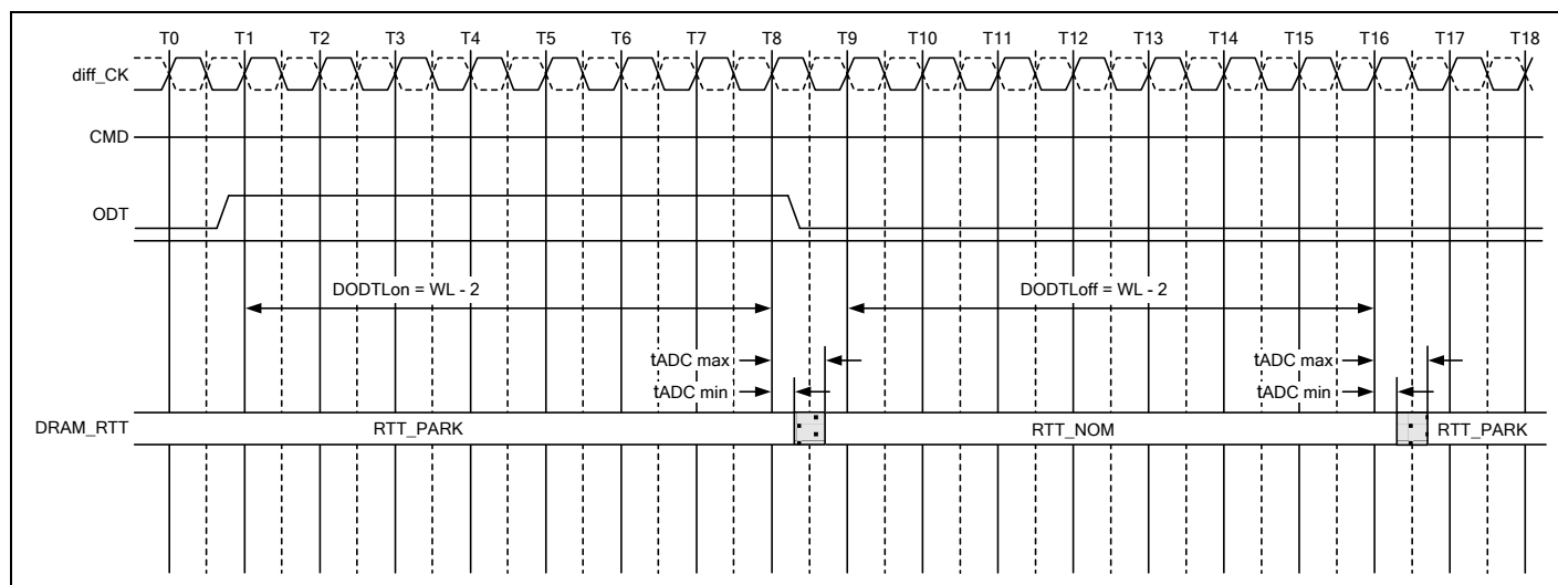
Figure 168 – Synchronous ODT Timing Example for CWL=9, AL=0, PL=0; DODTLon=WL-2=7; DODTLoff=WL-2=7
