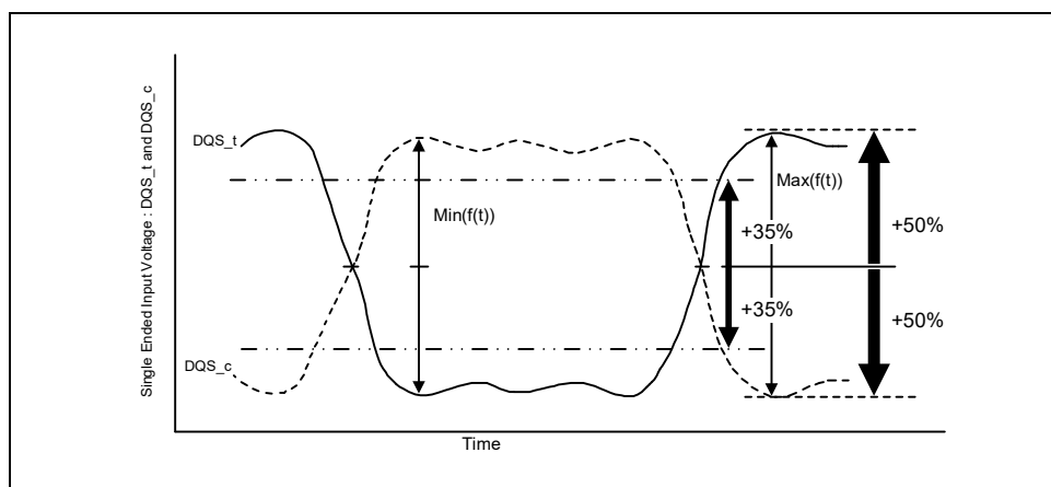
Figure 192 – Definition of differential DQS Peak Voltage and rage of exempt non-monotonic signaling
