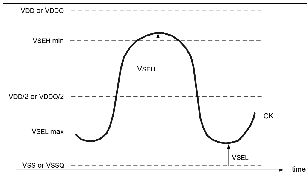
Figure 183 – Single-ended requirement for differential signals
