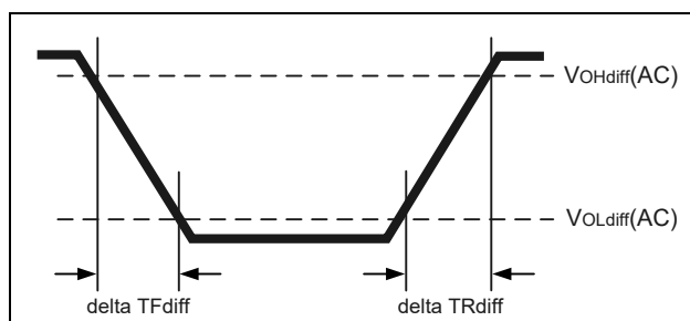
Figure 197 – Differential Output Slew Rate Definition
