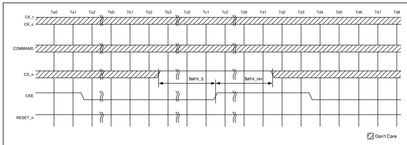
Figure 157 – CKE Transition Limitation to hold Maximum Power Saving Mode
