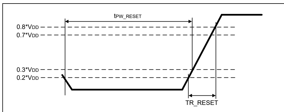
Figure 190 – RESET_n Input Slew Rate Definition
