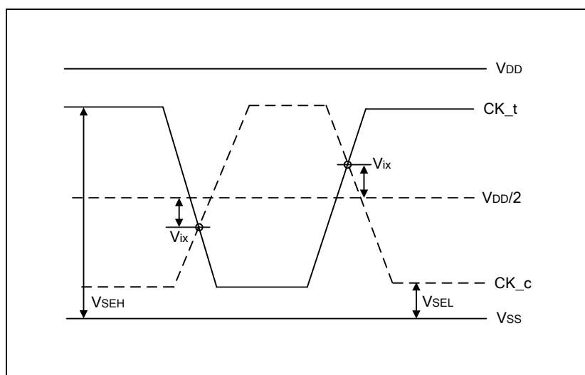
Figure 189 – Vix Definition (CK)
