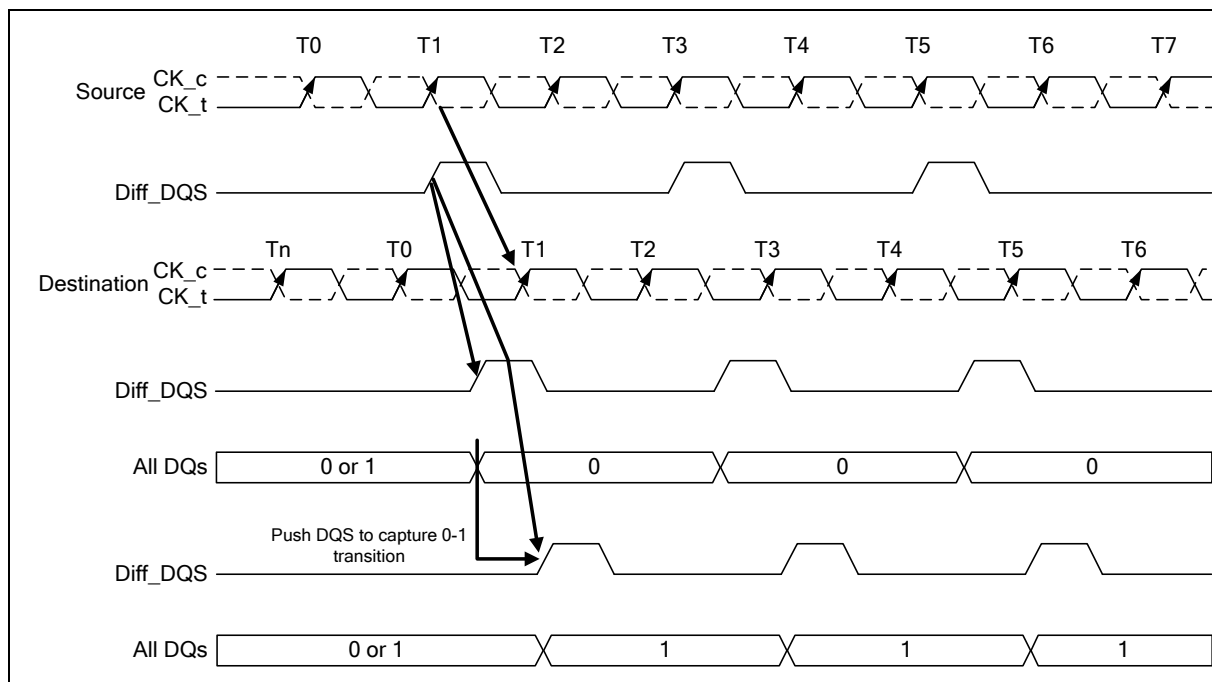
Figure 9 – Write Leveling Concept
