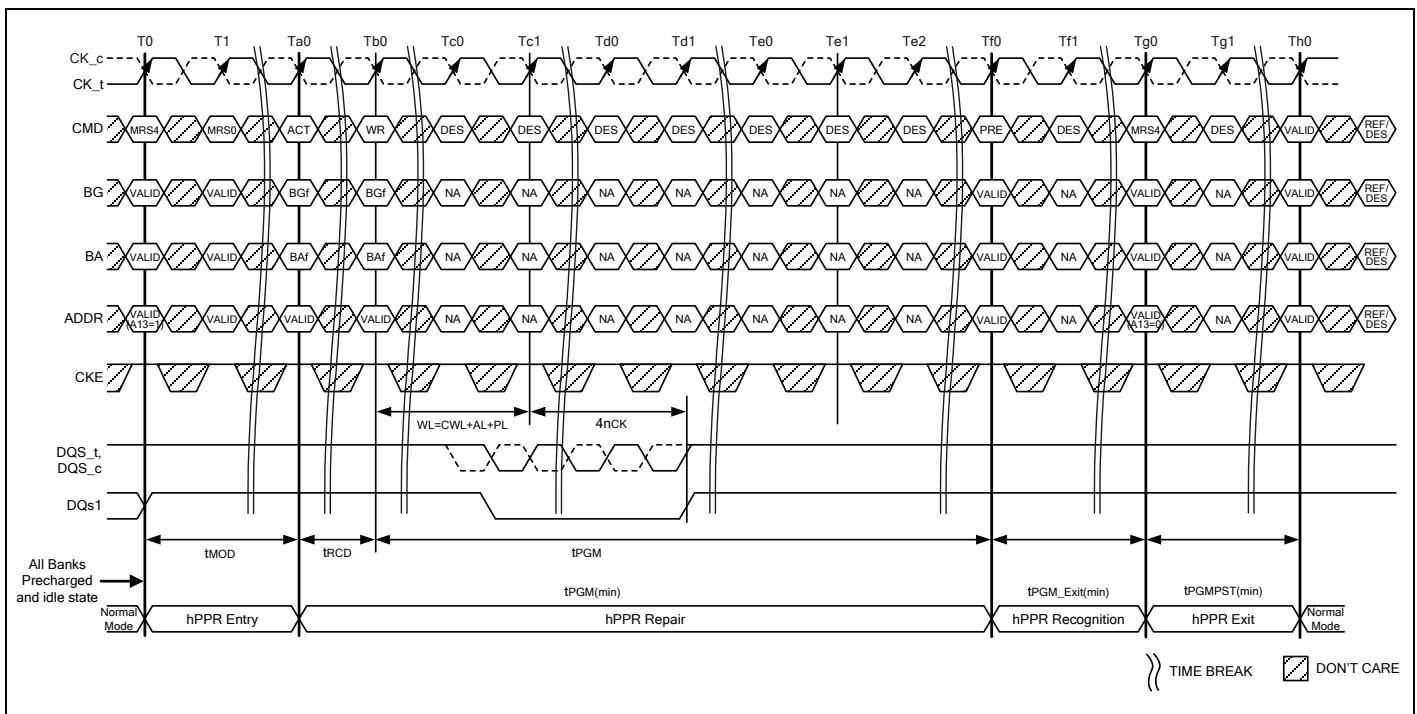
Figure 164 – Hard Fail Row Repair (WR Case)
