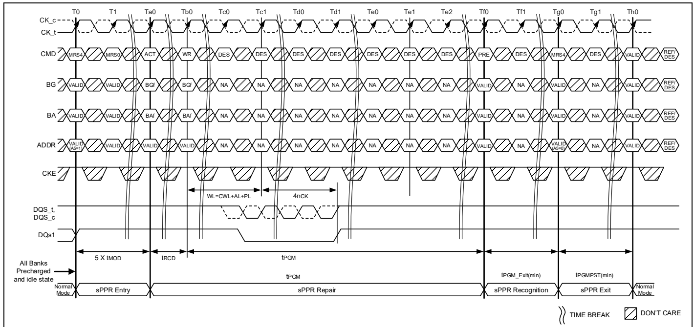
Figure 165 – Fail Row Soft PPR (WR Case)
