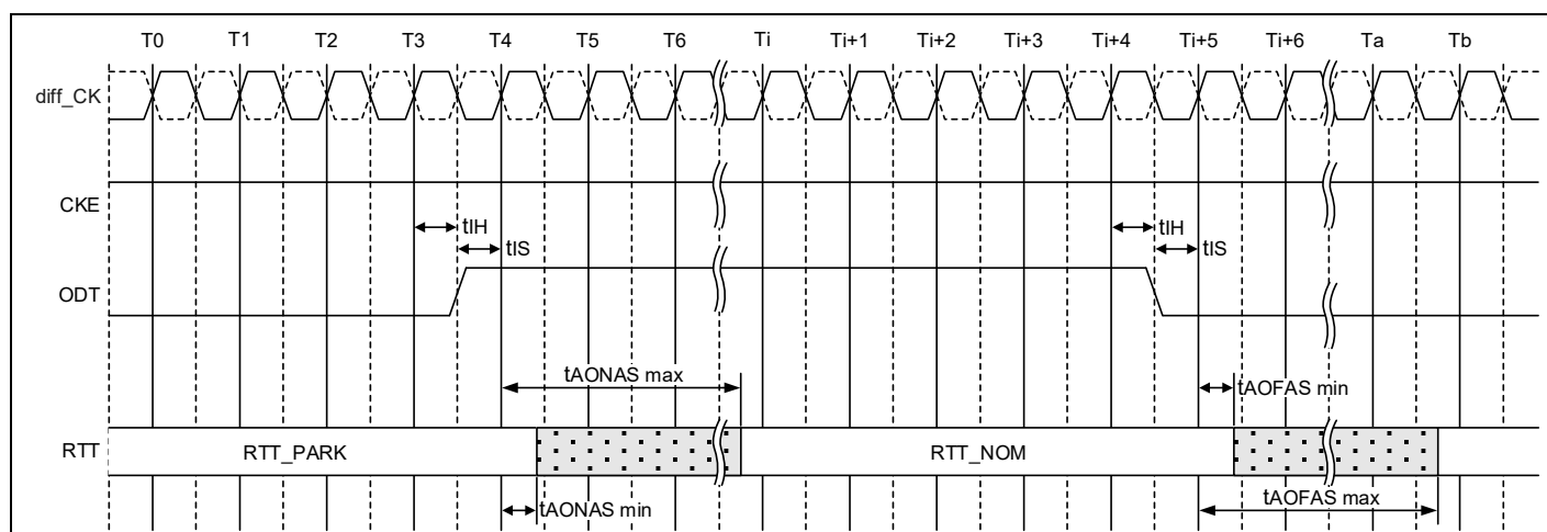
Figure 174 – Asynchronous ODT Timing on DDR4 SDRAM with DLL-off
