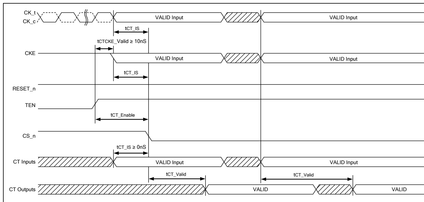
Figure 159 – Timing Diagram for Connectivity Test (CT) Mode
