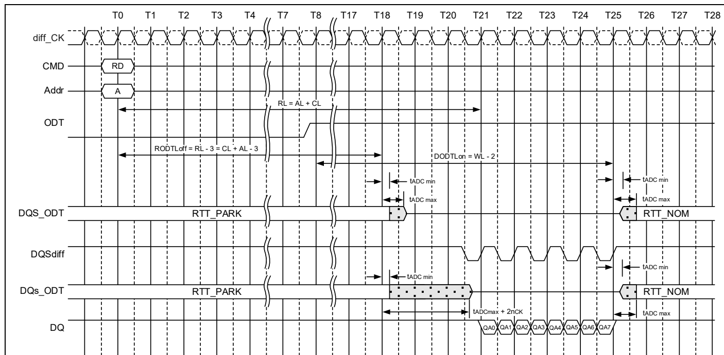
Figure 171 – Example: CL=11, PL=0; AL=CL-1=10; RL=AL+PL+CL=21; CWL=9; DODTLon=AL+CWL-2=17; RODTLoft=CL+AL-3=18; 2tCK preamble
