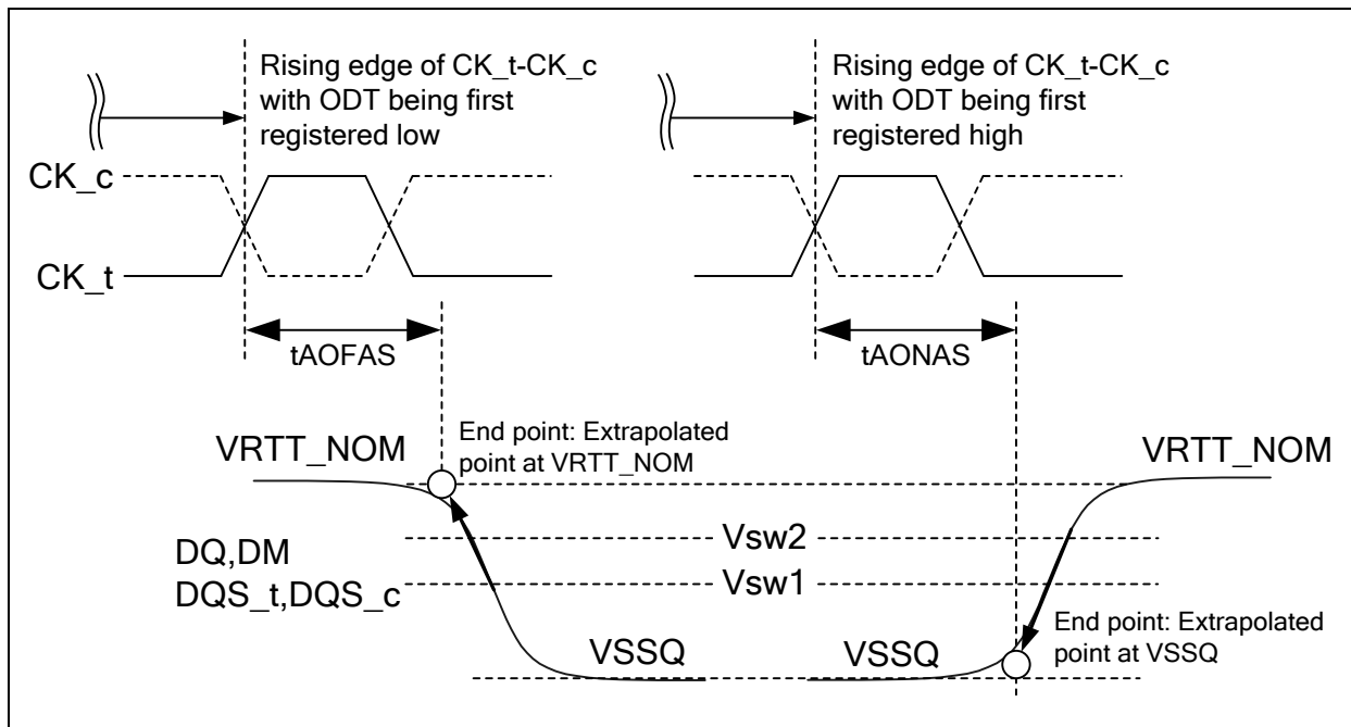
Figure 180 – Definition of tAOFAS and tAONAS
