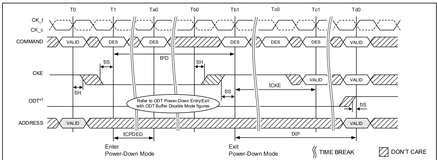
Figure 143 – Active Power-Down Entry and Exit Timing Diagram MR5 bit A5 = 0
