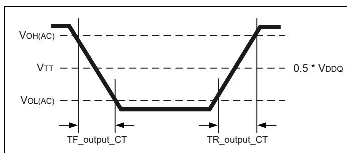
Figure 198 – Output Slew Rate Definition of Connectivity Test Mode
