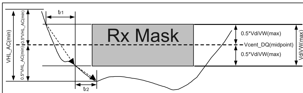
Figure 207 – Slew Rate Conditions for Falling Transition
