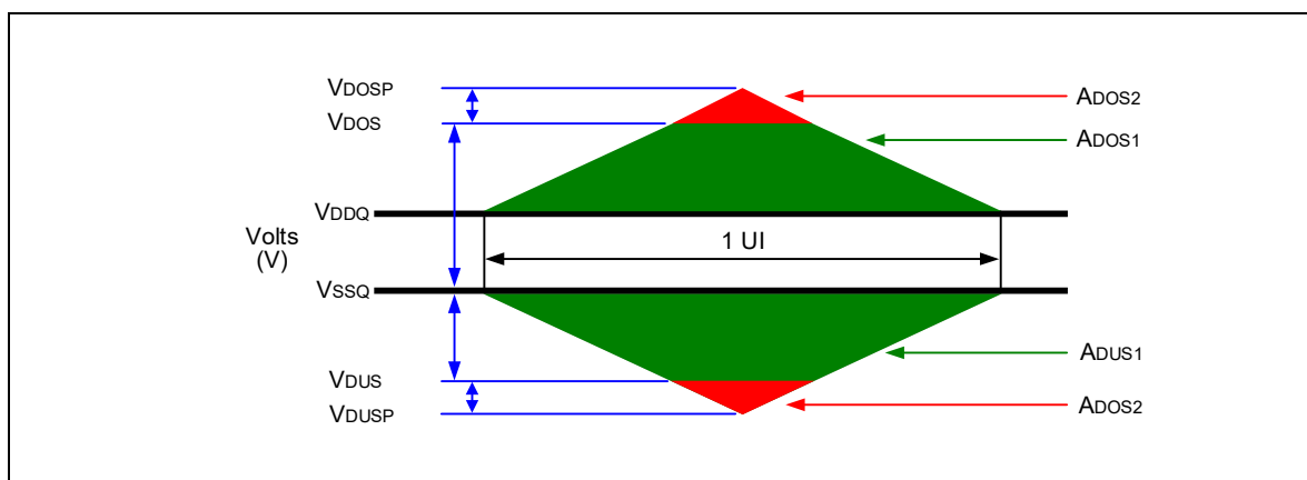
Figure 186 – Data, Strobe and Mask Overshoot and Undershoot Definition
