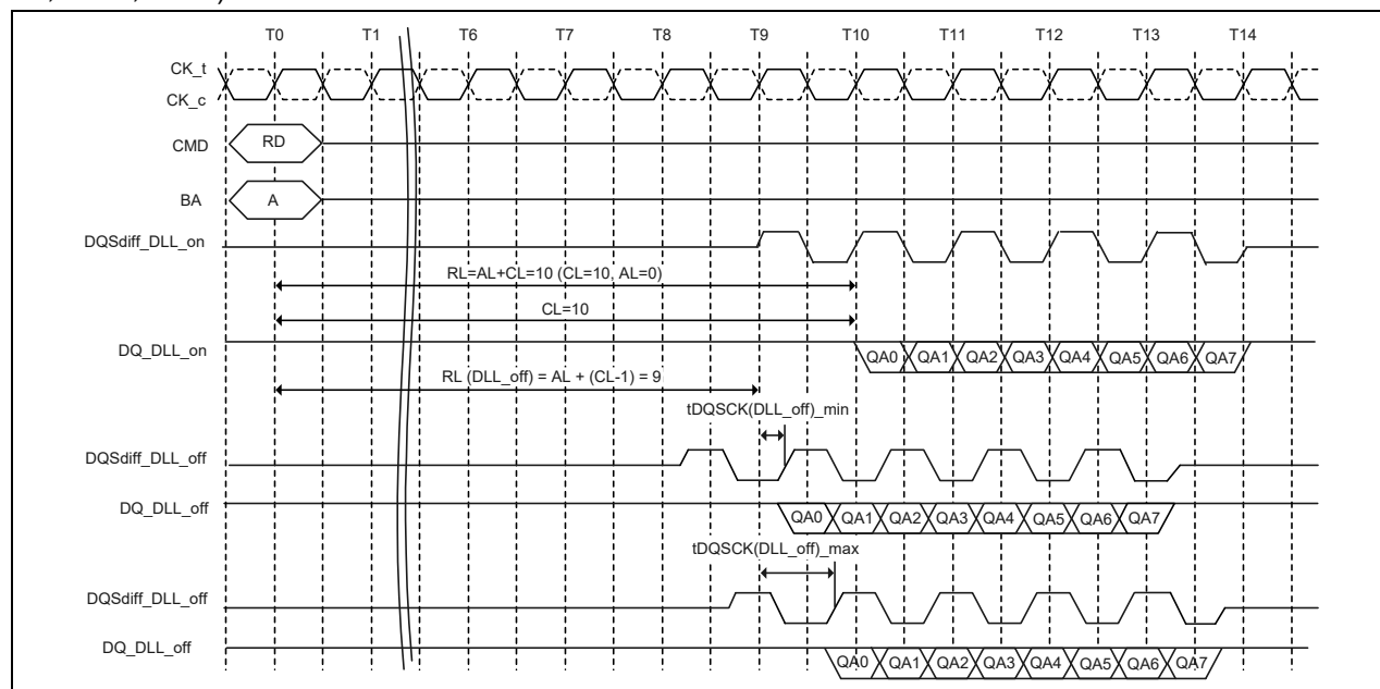
Figure 8 – READ operation at DLL-off mode
