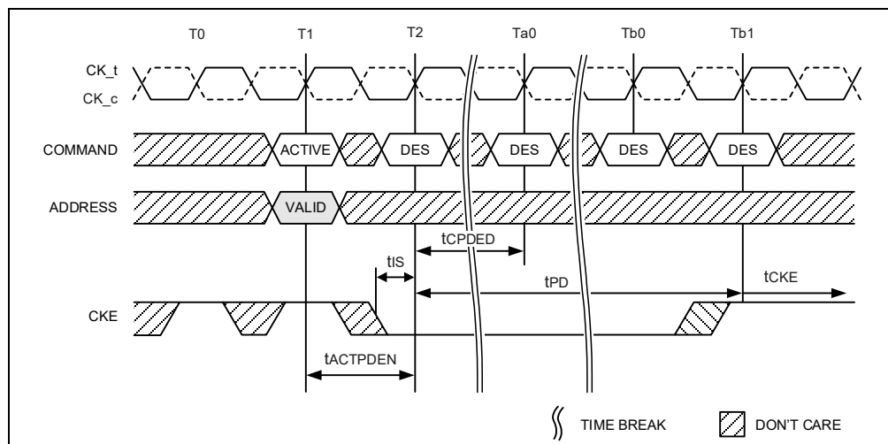
Figure 150 – Activate Command to Power-Down Entry
