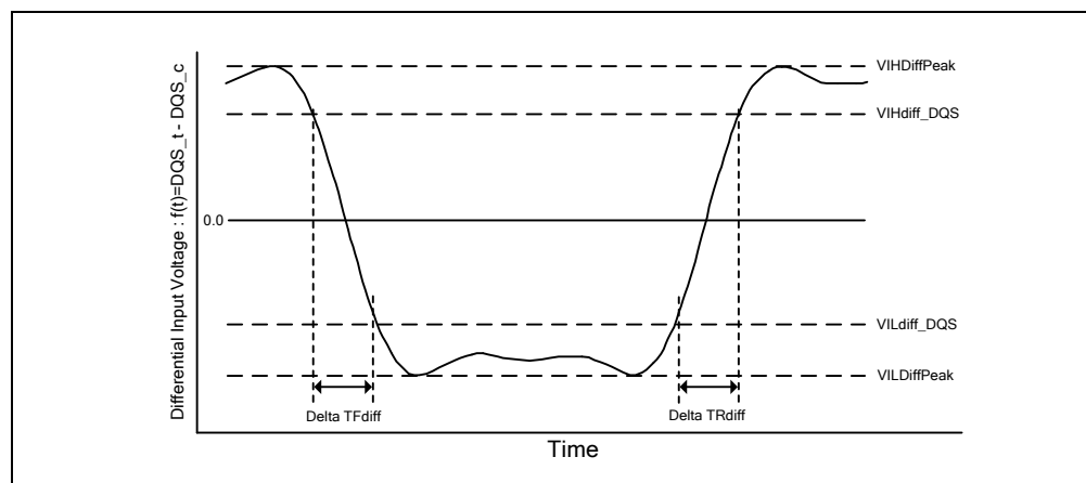
Figure 194 – Differential Input Slew Rate Definition for DQS t , DQS c
