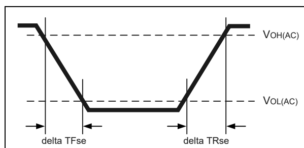
Figure 196 – Single-ended Output Slew Rate Definition
