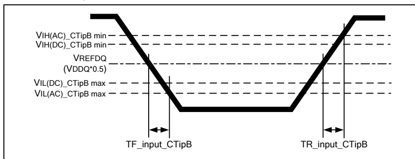
Figure 162 – Input B Slew Rate Definition
