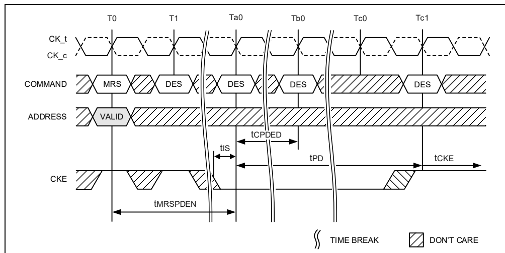
Figure 152 – MRS Command to Power-Down Entry
