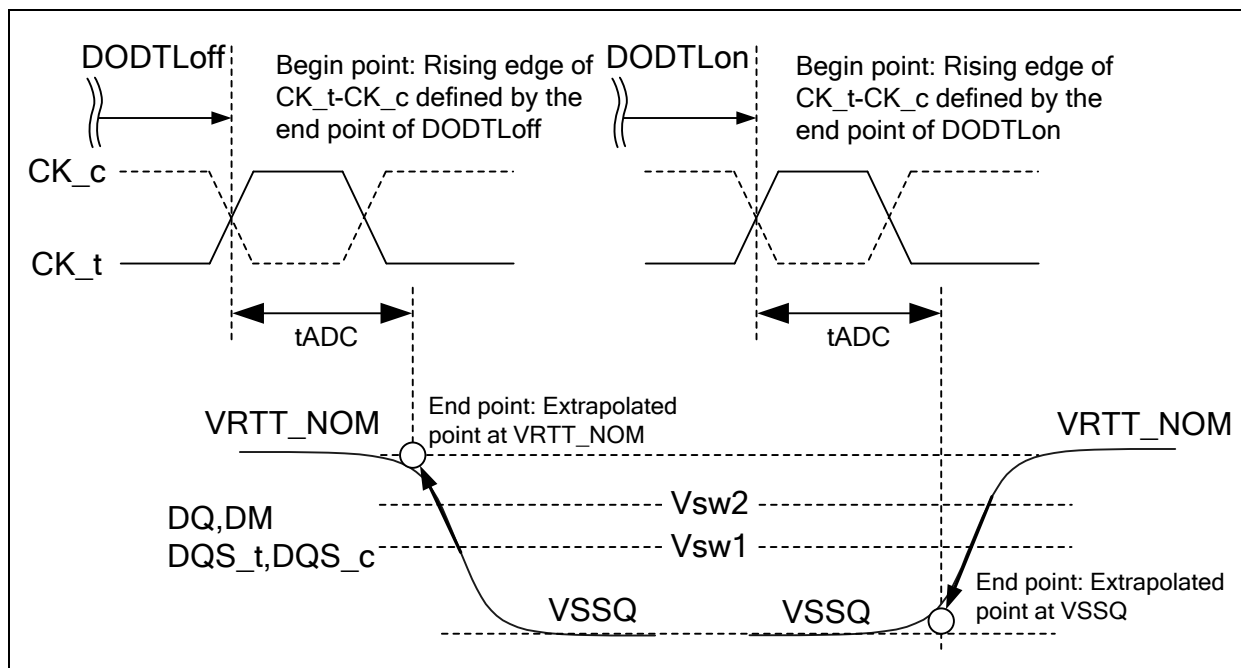
Figure 178 – Definition of t_{ADC} at Direct ODT Control
