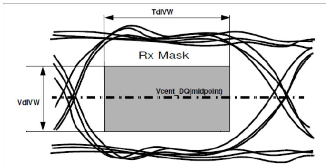
Figure 203 – DQ Receiver (Rx) compliance mask
