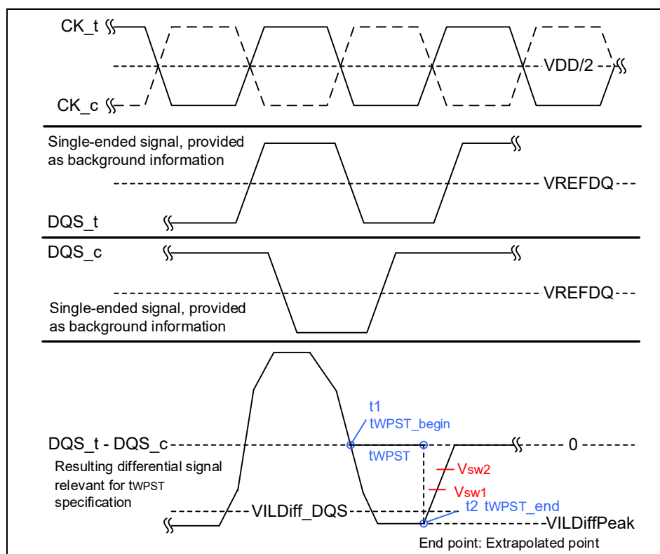
Figure 108 – Method for calculating tWPST transitions and endpoints
