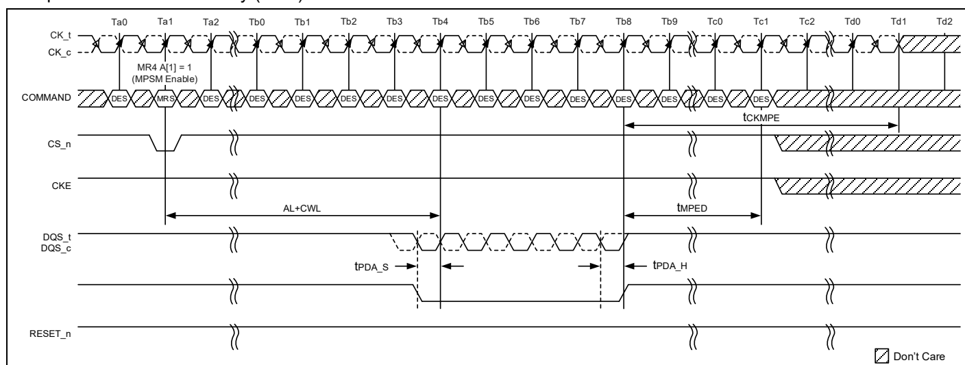
Figure 156 – Maximum Power Saving mode Entry with PDA
