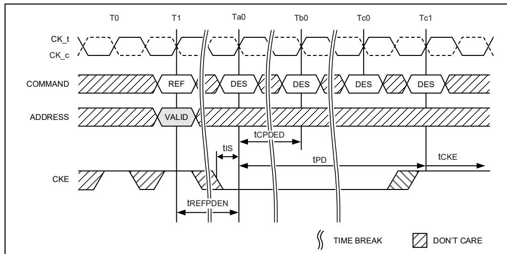
Figure 149 – Refresh Command to Power-Down Entry
