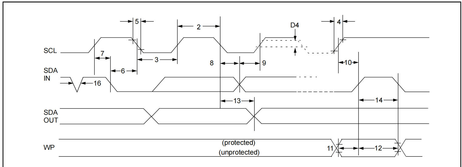
FIGURE 1 : BUS TIMING DATA
