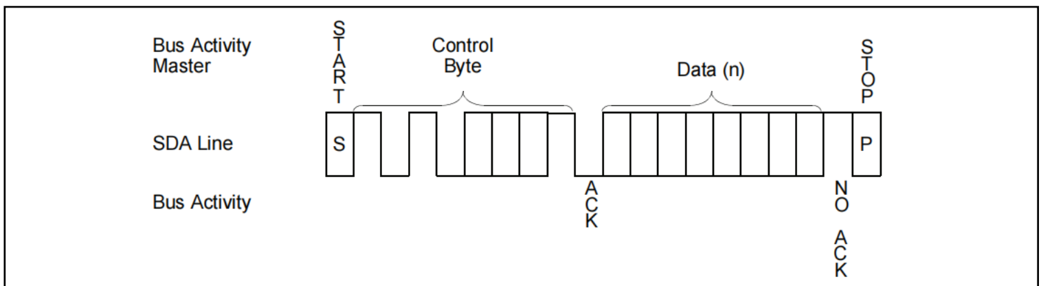
FIGURE 9: CURRENT ADDRESS READ
