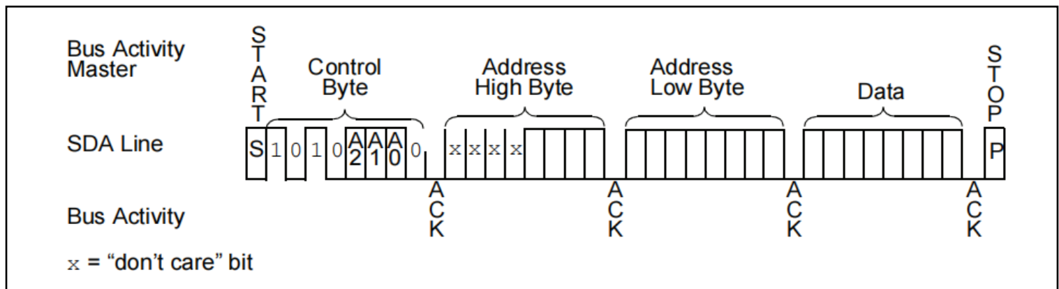
FIGURE 6 : BYTE WRITE
