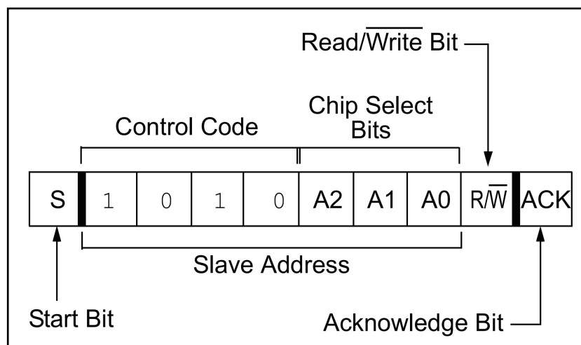
FIGURE 4: CONTROL BYTE FORMAT
