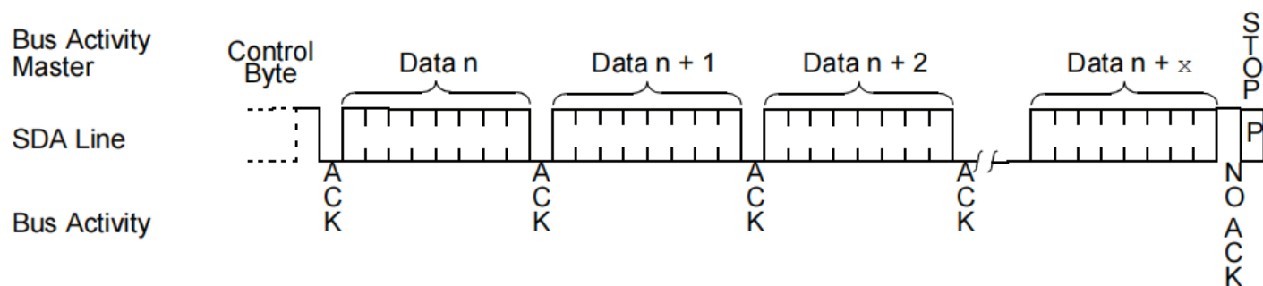
FIGURE 11.SEQUENTIAL READ
