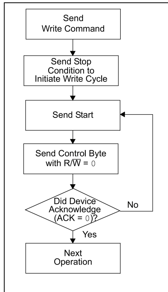
FIGURE 8: ACKNOWLEDGE POLLING FLOW
