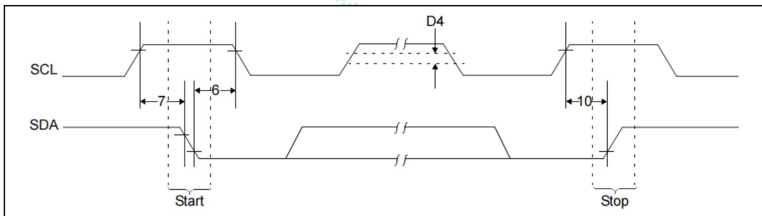
FIGURE 2: BUS TIMING START/STOP
