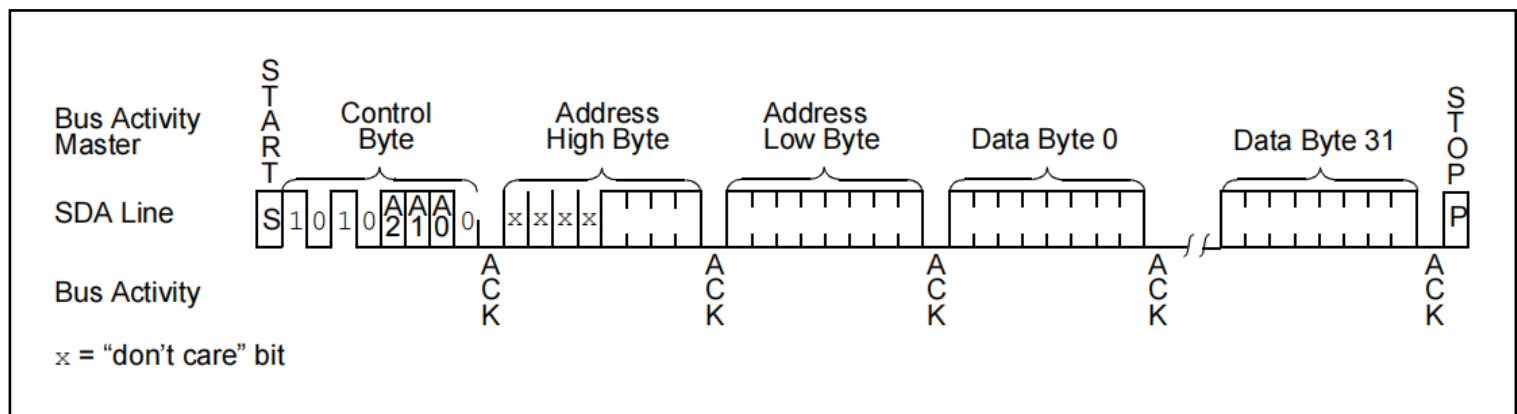
FIGURE 7: PAGE WRITE
