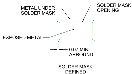
器件封装焊盘布局举例 SCALE:15X
