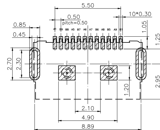
RECOMMEND P.C.B LAYOUT(TOP VIEW) (COMPONENT SIDE) TOLERANCE±0.05
