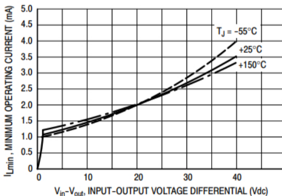
Minimum Operating Current
