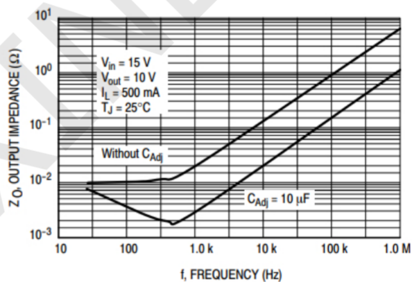
Output Impedance
