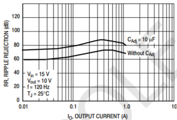
Ripple Rejection versus Output Current
