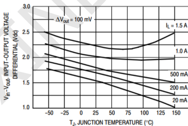
Dropout Voltage
