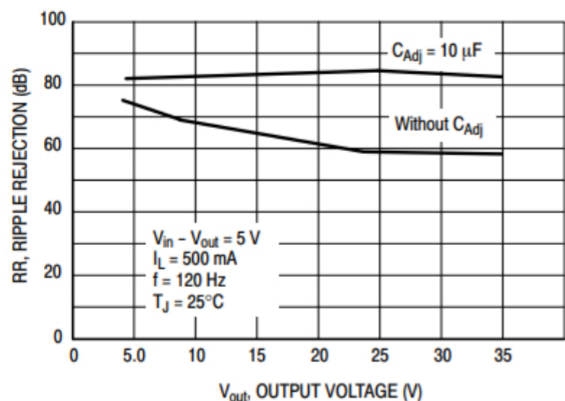
Ripple Rejection versus Output Voltage
