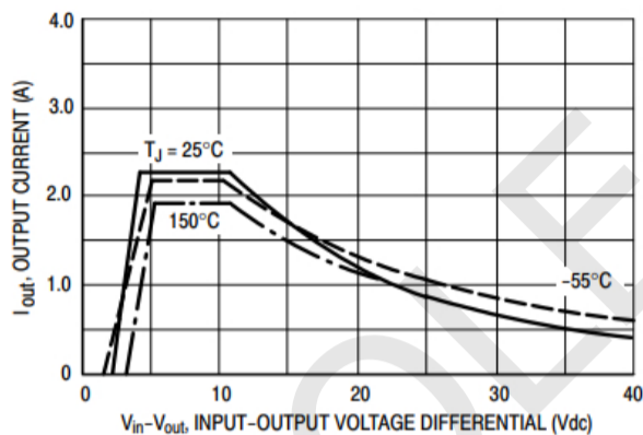
Current Limit
