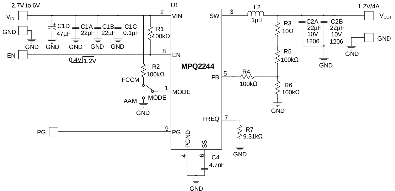
Figure 6: Typical Application Circuit ( V_{OUT} = 1.2V , I_{OUT} = 4A )
