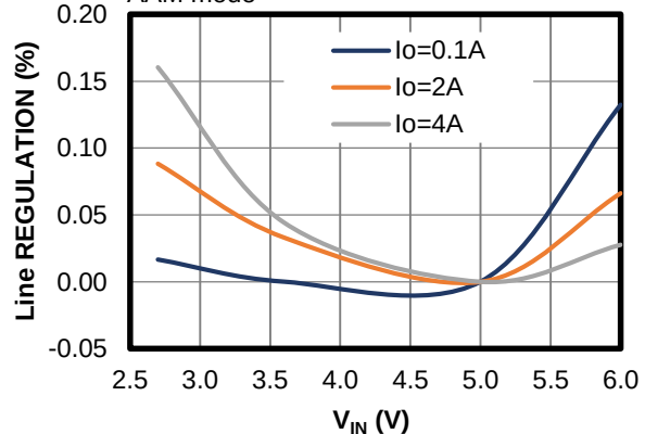
Line Regulation
