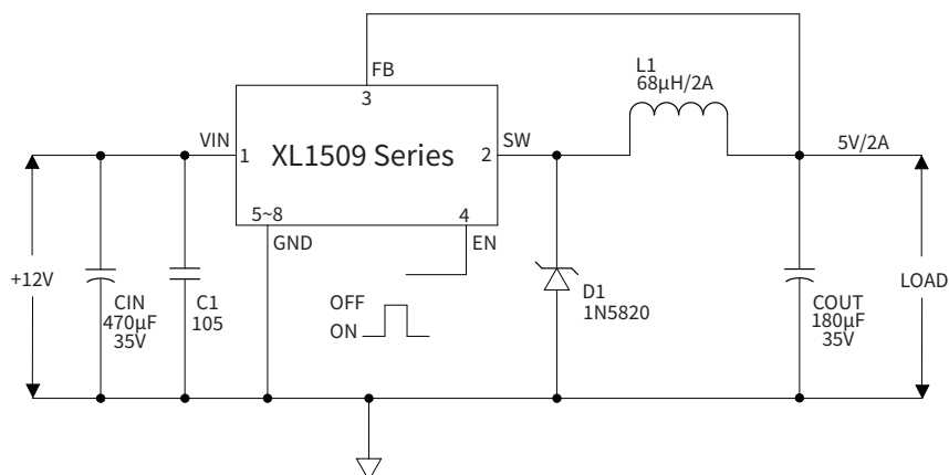
Figure 2.XL1509 Series Typical Application Circuit
