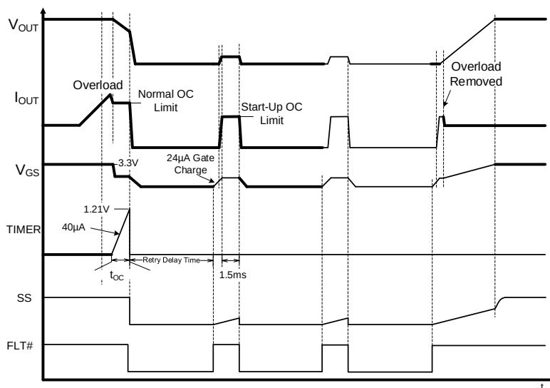
Figure 5: Normal OCP Behavior in Auto-Retry Mode
