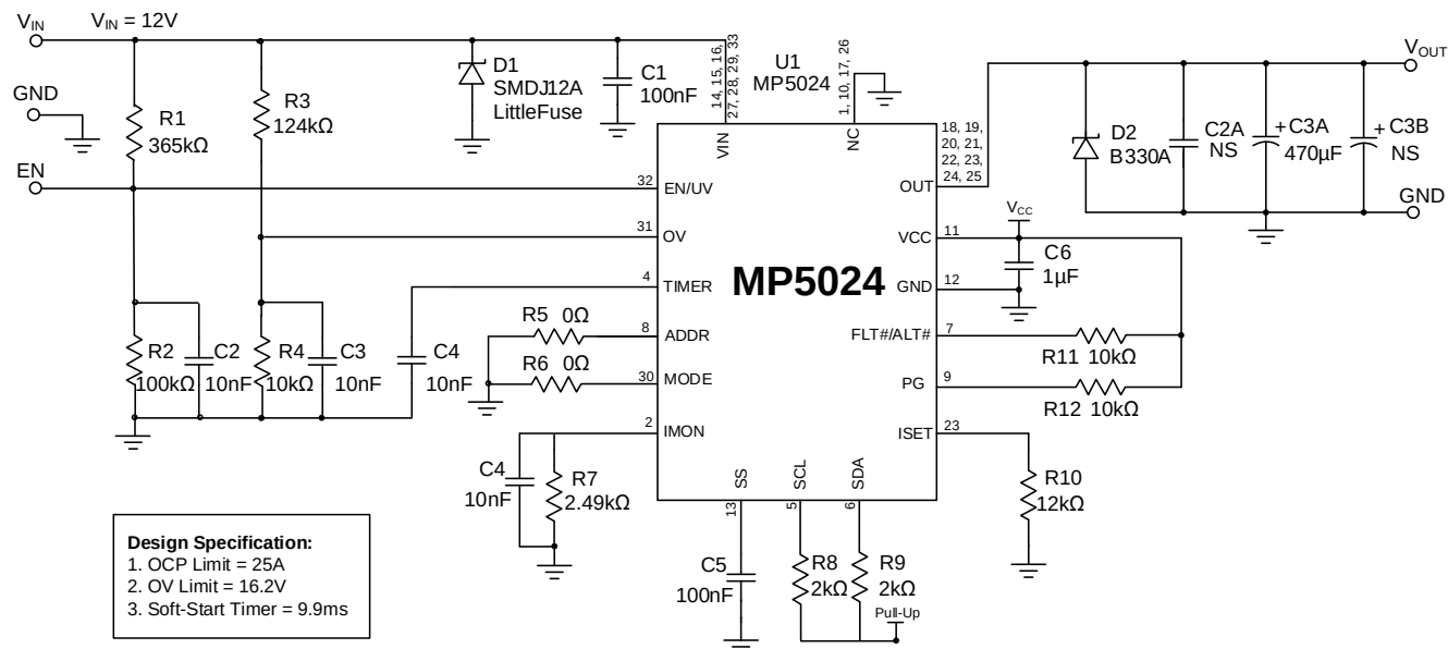
Figure 15: Typical Application Circuit (V IN = 12V, OC Limit = 25A)
