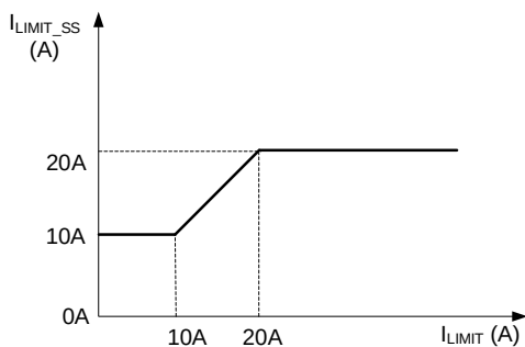
Figure 3: Start-Up Current Limit Compared to Normal Over-Current Limit
