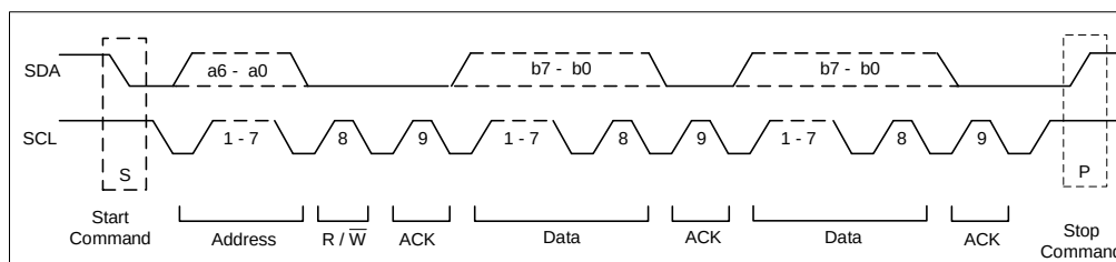
Figure 12: Data Transfer over the PMBus
