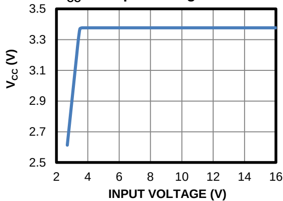
V_{CC} vs. Input Voltage
