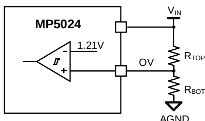
Figure 8: OV Connection
