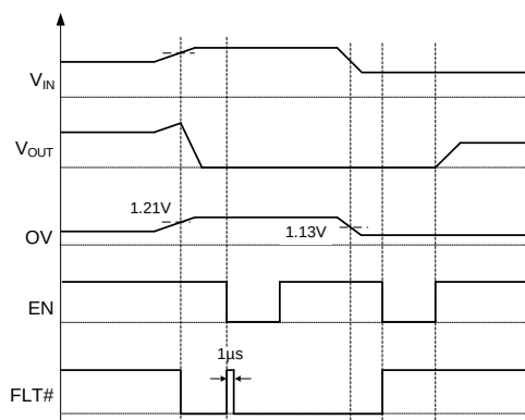
Figure 9: OVP Behavior
