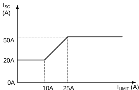
Figure 6: Short-Circuit Current Limit to Normal Over-Current Limit
