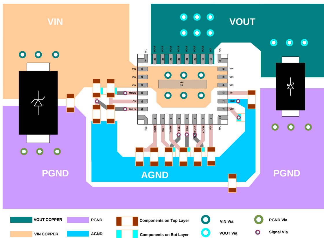
Figure 14: Example of PCB Layout (Placement and Top Layer PCB)
