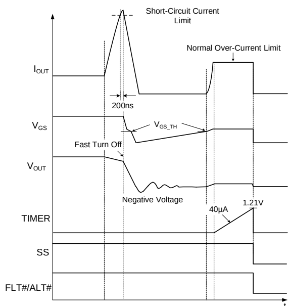
Figure 7: SCP Behavior in Latch-Off Mode
