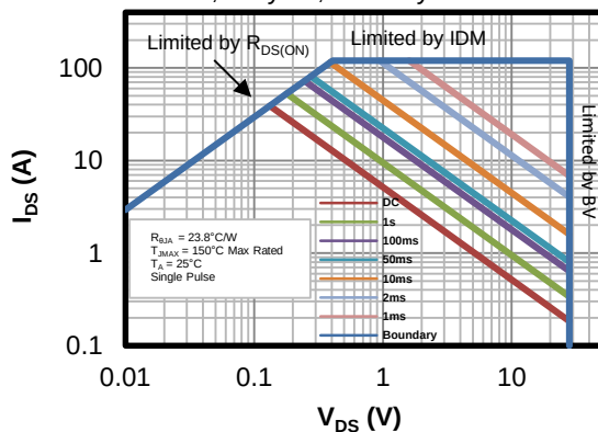
Safe Operation Area (SOA)
