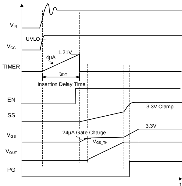
Figure 2: Start-Up Sequence
