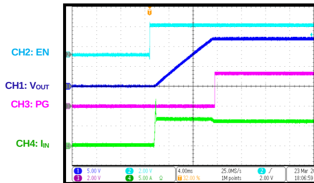
Start-Up via EN
