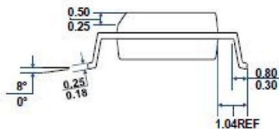
LEFT-SIDE VIEW
