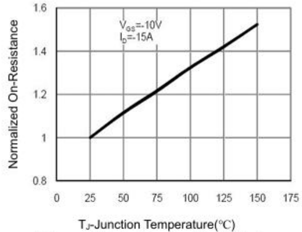
Figure 8 Drain-Source On-Resistance
