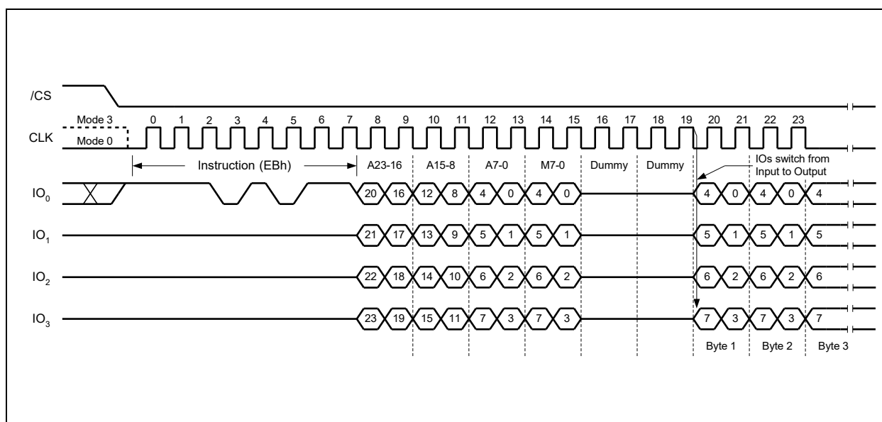
Figure 25a. Fast Read Quad I/O Instruction (Initial command or previous M5-4≠10, SPI Mode) "Set Read Parameters" command (C0h) can set the number of dummy clocks.
