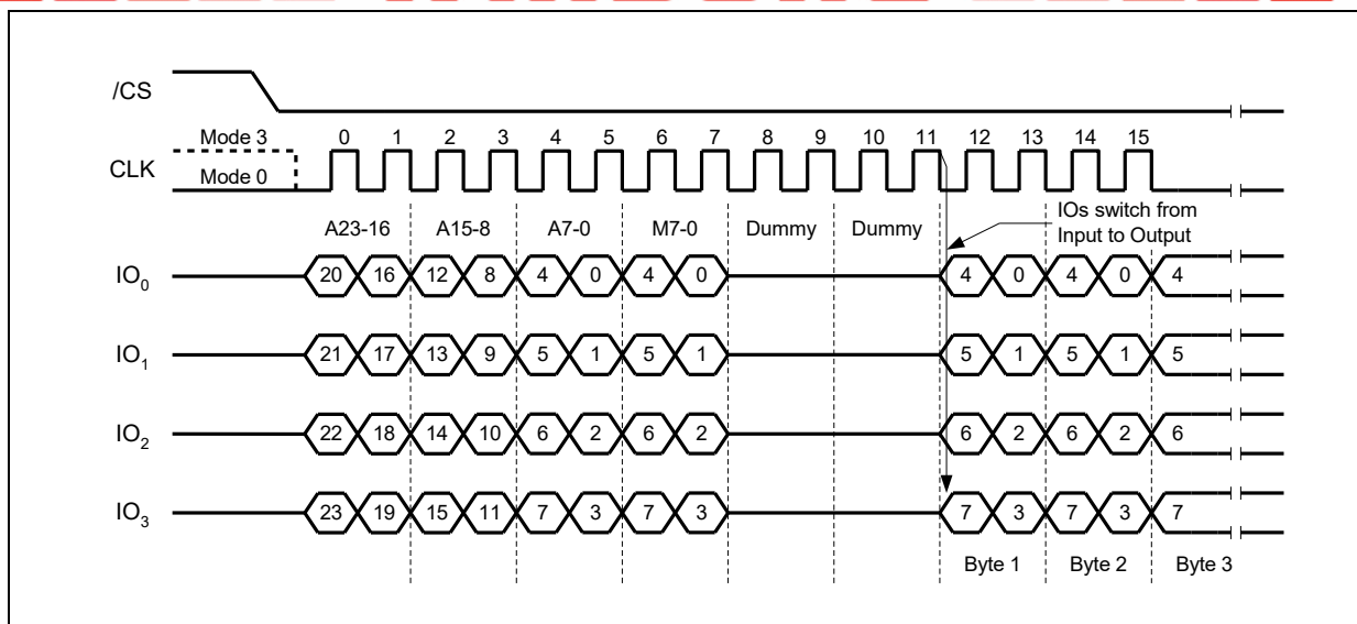
Figure 25b. Fast Read Quad I/O Instruction (Previous command set M5-4 = 10, SPI Mode)
