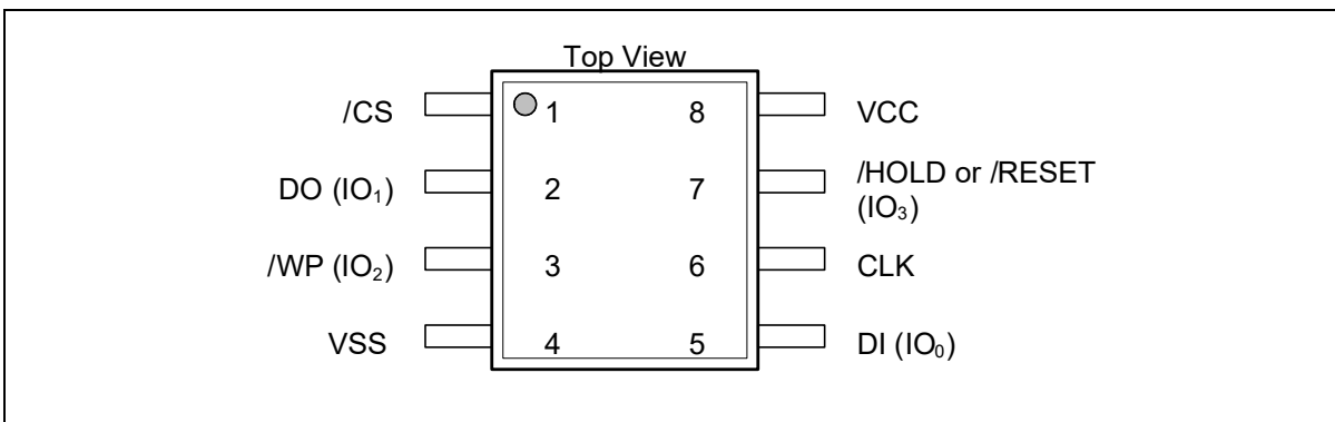
Figure 1a. Pin Assignments, 8-pin SOP 150/208-MIL (Package Code SN, SS)
