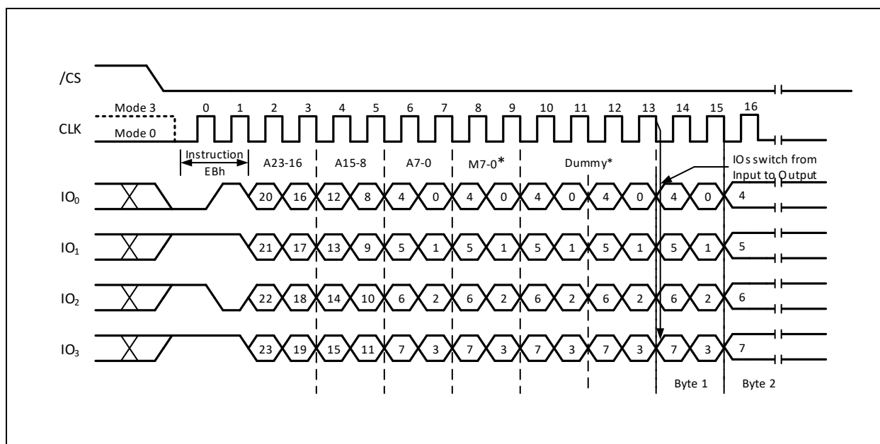
Figure 25c. Fast Read Quad I/O Instruction (Initial command or previous M5-4≠10, QPI Mode) “Set Read Parameters” command (C0h) can set the number of dummy clocks.
