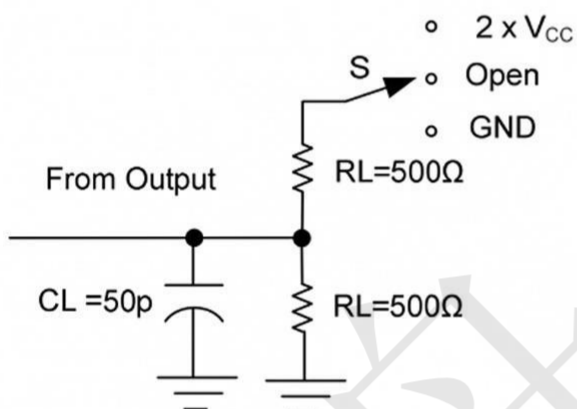
TEST CIRCUIT
