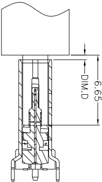
AFTER MATING
