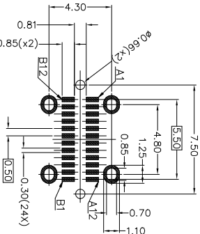
RECOMMENDED PCB LAYOUT(TOP VIEW) THICKNESS 1.5±0.10MM;DEFAULT TOLERANCE:±0.05
