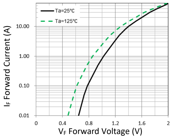
Figure 1. Forward Characteristic(typ.)
