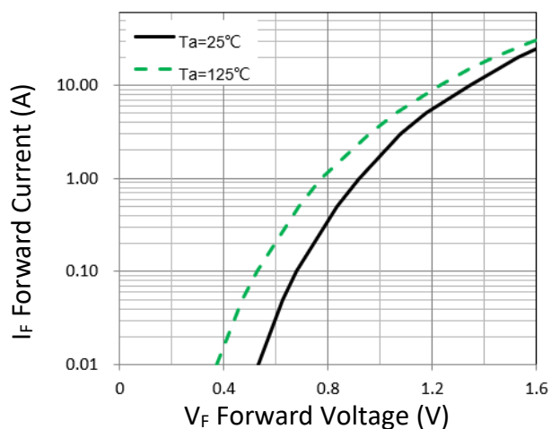
Figure 1. Forward Characteristic(typ.)
