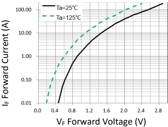
Figure 1. Forward Characteristic(typ.)
