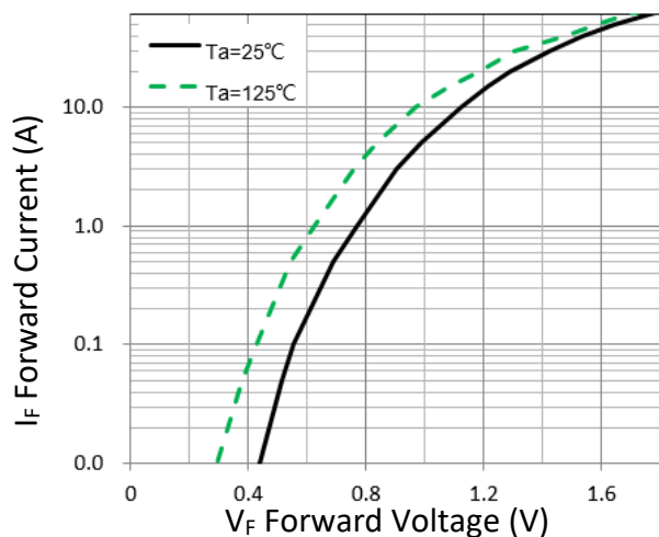
Figure 1. Forward Characteristic(typ.)
